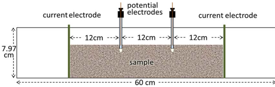
Figure 3-4. Sketch of the sample holder used to make SIP measurements during evaporative drying of unsaturated samples
