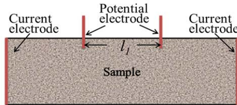
Figure 2-2. Four point laboratorial system. l_1 is the spacing between two potential electrodes
