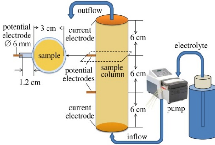
Figure 3-2. Sketch of the saturated experimental setup
