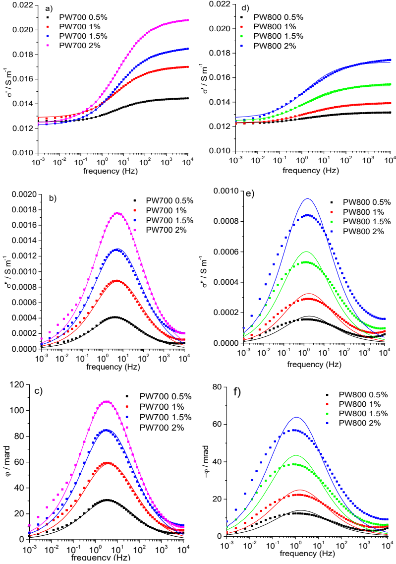
Figure 5-2. Real part \sigma'(\omega) , imaginary part \sigma''(\omega) , and phase \varphi(\omega) of the measured complex electrical conductivity for sand-biochar mixtures with various mass fractions of PW700 (a, b, c) and PW800 (d, e, f) with 4 mM NaCl (dots). The predictions obtained with the Wong model using the prescribed and fitted model parameters in Tab. 5-4 and Tab. 5-5 are also provided (lines).
