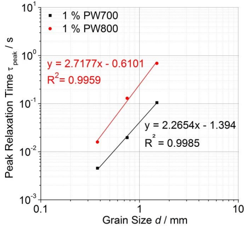
Figure 4-5. Peak relaxation time \tau_{peak} of PW700 and PW800 as a function of grain diameter d of biochar in sand-biochar mixtures (4 mM NaCl).
