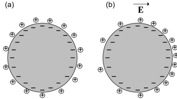
Figure 2-3. Illustration of the (a) static Stern layer and (b) polarized Stern layer under an applied electrical field.
