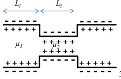
Figure 2-9. Schematic illustration of 1-D pore space model consisting of an interconnected wide pore with a length L_1 (m) and ion mobility \mu_1 ( \text{m}^2 \text{V}^{-1} \text{s}^{-1} ), and a narrow pore with a length L_2 (m) and ion mobility \mu_2 ( \text{m}^2 \text{V}^{-1} \text{s}^{-1} ).
