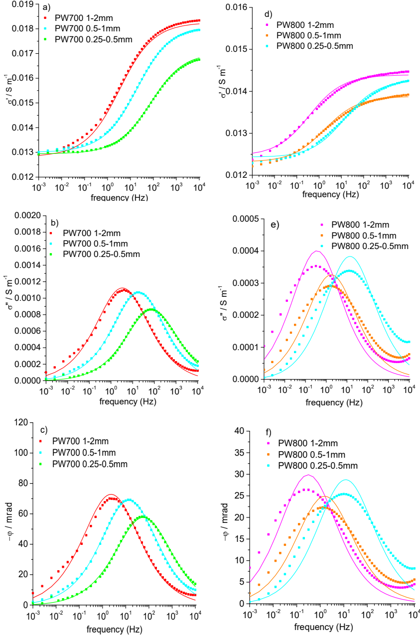
Figure 5-3. Real part \sigma'(\omega) , imaginary part \sigma''(\omega) , and phase \phi(\omega) of the measured complex electrical conductivity for sand-biochar mixtures with various particles sizes of PW700 (a, b, c) and PW800 (d, e, f) with 4 mM NaCl (dots). The predictions obtained with the Wong model using the prescribed and fitted model parameters in Tab. 5-4 and Tab. 5-5 are also provided (lines).
