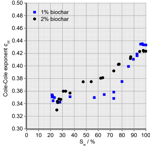
Figure 6-6. Cole-Cole exponent ( c_{cc} ) as a function of saturation ( S_w ) obtained by fitting a Cole-Cole model to spectral induced polarization (SIP) data for the 1% and 2% sand-biochar mixture with PW800.
