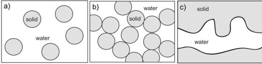
Figure 2-5. Three types of porous materials characterized by different polarization mechanisms. a) Suspended colloidal particle. b) Granular porous medium. c) Porous continuous solid phase (Revil and Cosenza, 2010).
