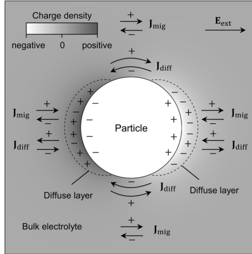
Figure 2-6. Illustration of electrode polarization of a suspended conductive particle in electrolyte (Bücker et al., 2018).
