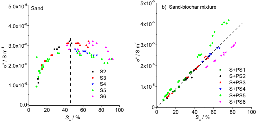
Figure 6-11. Measured imaginary part of the complex electrical conductivity \sigma'' at 10Hz as a function of water saturation S_w ; a) pure sand sample, b) sand-biochar mixture with 2 % biochar PS. Please note that the scale of the Y-axis of panel b) for biochar is one order of magnitude larger than that of panel a) for sand.
