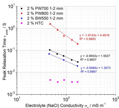
Figure 4-11. Peak relaxation time \tau_{\text{peak}} of mixtures of 2 % PW700, PW800, BW550 and HTC in sand as a function of electrolyte conductivity (NaCl).
