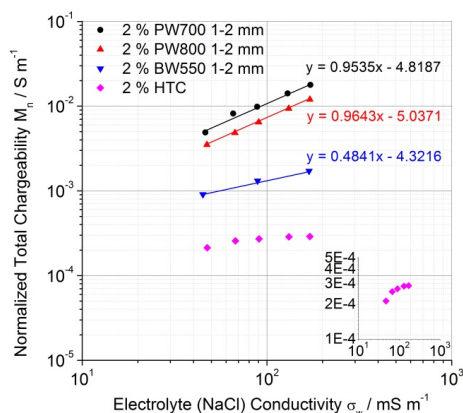
Figure 4-10. Normalized total chargeability M_n of mixtures of 2 % PW700, PW800, BW550 and HTC in sand as a function of electrolyte conductivity (NaCl).
