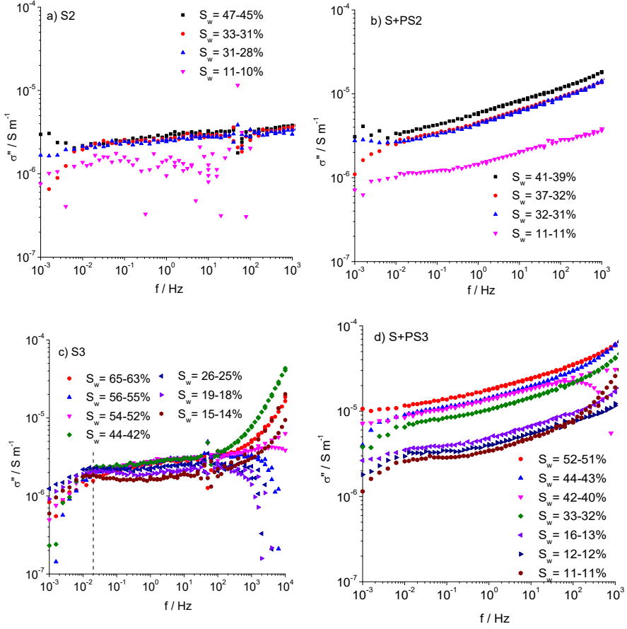
Figure 6-10. Frequency-dependent imaginary part of the complex electrical conductivity ( \sigma'' ) of sample set S2 (top row) and sample set S3 (bottom row). S indicates pure sand samples. S+PS indicates sand-biochar mixture with 2 % biochar PS. Obvious noise can be observed at around 50 Hz for some measurements, which was caused by the presence of other power sources (AC 230 V/50 Hz).
