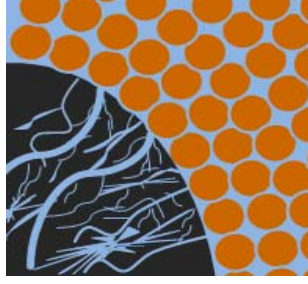
Figure 6-2. Conceptual illustration of different types of porosity present in sand-biochar mixtures. Orange indicates sand particles that result in a relatively narrow pore size distribution, whereas the black area indicates biochar with a heterogeneous pore size distribution with both large and small pores.
