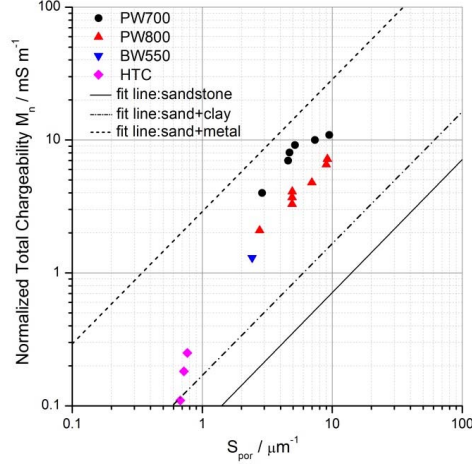
Figure 4-12. Relationship between normalized total chargeability M_n derived from Debye decomposition and the normalized specific surface area per unit mass S_{por} for different sand-biochar mixtures (NaCl electrolyte, 100 mS m -1 ). For comparison, fitting curves for different materials from Weller et al. (2010) are also provided.
