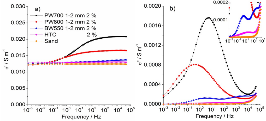
Figure 4-1. Complex conductivity of mixtures of sand and 2 % of different biochars (4 mM NaCl); a) real part, b) imaginary part. The inset expands the y-scale to highlight the spectra of samples with low polarization.
