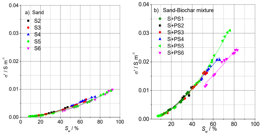
Figure 6-9. Measured real part of the complex electrical conductivity \sigma' at 10 Hz as a function of water saturation S_w and fitted curves of the simplified Archie's law; a) pure sand samples, b) sand-biochar mixtures with 2 % biochar PS.
