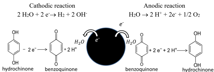
Figure 5-1. Schematic illustration of a possible redox reaction at the surface of biochar.
