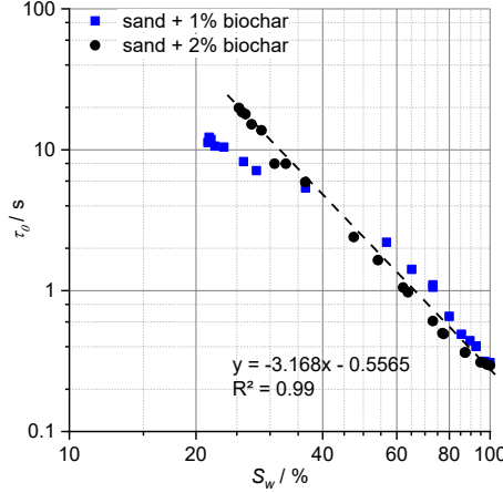
Figure 6-7. Relaxation time ( \tau_0 ) as a function of saturation ( S_w ) obtained by fitting a Cole-Cole model to spectral induced polarization (SIP) data for the 1% and 2% sand-biochar mixture with PW800.
