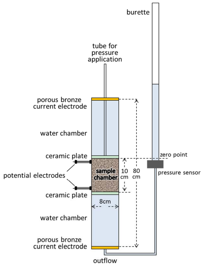
Figure 3-3. Sketch of the sample holder used to make SIP measurements during pressure drainage of unsaturated samples
