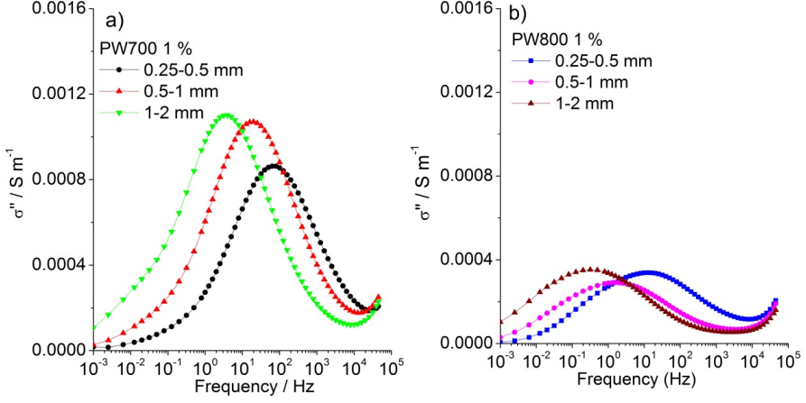
Figure 4-4. Imaginary part ( \sigma'' ) of the complex conductivity of a) PW700 and b) PW800 with different particle diameter of biochar in sand-biochar mixtures (4 mM NaCl).
