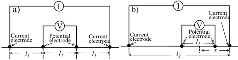
Figure 2-1. Two types of four-point electrode array for SIP measurements: a) Wenner array; l_1 is spacing between each pair of adjacent electrodes. b) Schlumberger array; l_1 and l_2 are the spacing between two potential electrodes and two current electrodes, respectively. x is the distance between one current electrode and the middle point of two potential electrodes.
