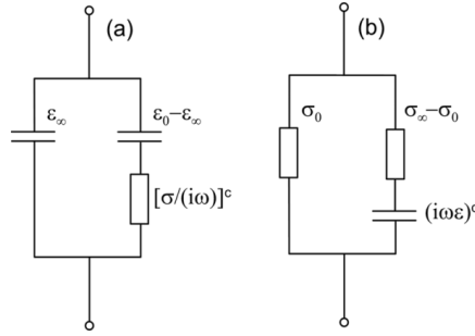
Figure 2-7. Equivalent electrical circuit model for the Cole–Cole equation formulated with (a) dielectric permittivity and (b) electrical conductivity (Tarasov and Titov, 2013).
