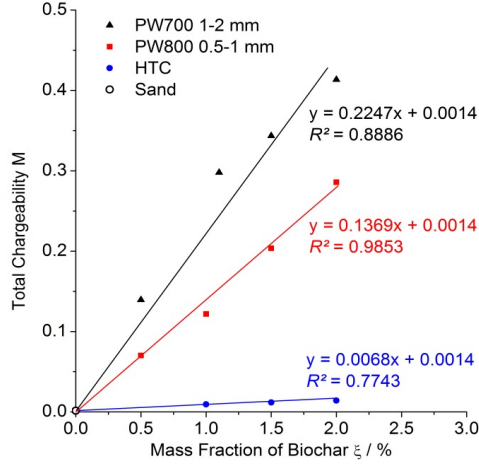
Figure 4-3. Total chargeability M of PW700, PW800 and HTC as a function of mass fraction of biochar in sand-biochar mixtures (4 mM NaCl).
