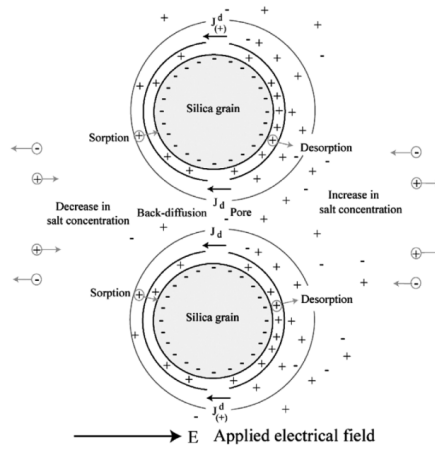
Figure 2-4. Illustration of membrane polarization (Revil and Cosenza, 2010; Revil and Florsch, 2010)
