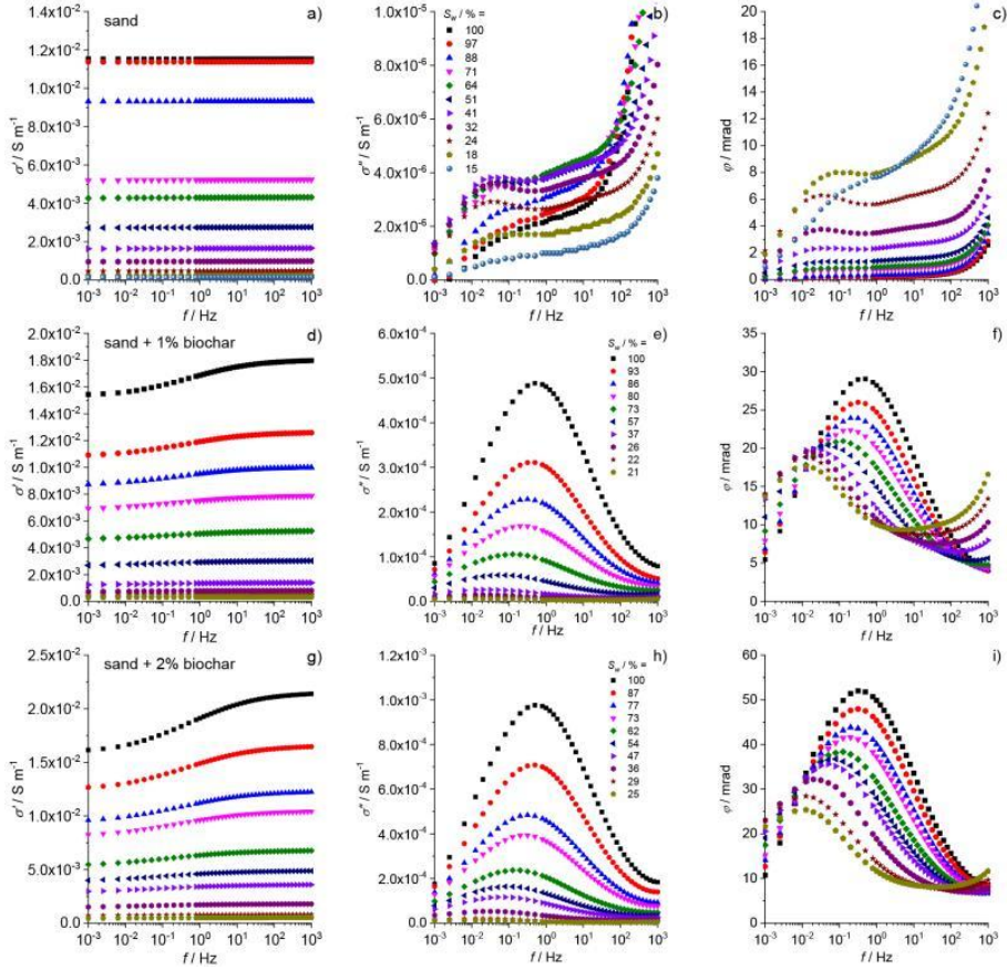
Figure 6-3. SIP measurements on pure sand (top row), 1% sand-biochar mixture with PW800 (middle row), and 2% sand-biochar mixture with PW800 (bottom row) for a range of saturation. SIP measurements are presented as the real part of the electrical conductivity \sigma' (left column), the imaginary part of the electrical conductivity \sigma'' (middle column), and the phase of the electrical conductivity \phi (right column).
