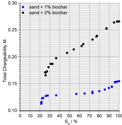
Figure 6-5. Total chargeability ( M ) as a function of saturation ( S_w ) obtained by fitting a Cole-Cole model to spectral induced polarization (SIP) data for the 1 % and 2 % sand-biochar mixture with PW800.
