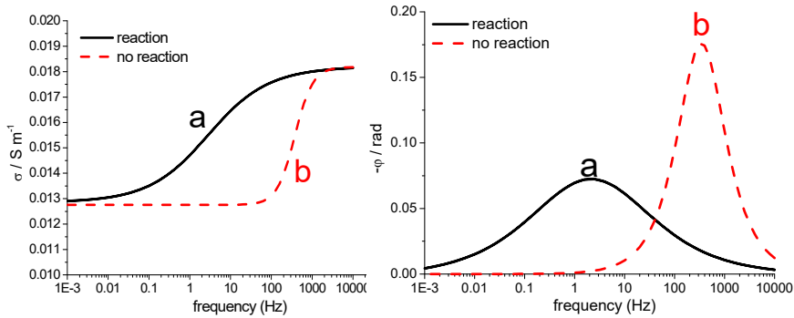
Figure 2-8. Effect of redox reactions on the predicted SIP response by the Wong model. The parameters for the model with redox reactions (curve a) are: \alpha = 1.8 \times 10^{-7} \text{ A s}^2 \text{ kg}^{-1} \text{ mol}^{-1} , \beta = 0.18 \text{ m mol}^{-1} \text{ s}^{-1} , c_r = 0.003 , D = 1.4 \times 10^{-9} \text{ m}^2 \text{ s}^{-1} , \varepsilon = 8.9 \times 10^{-11} \text{ F m}^{-1} , and v = 0.08 . In the case of the model without redox reactions (curve b), the parameters \alpha = \beta = c_2 = 0 and all other parameters were left unchanged.
