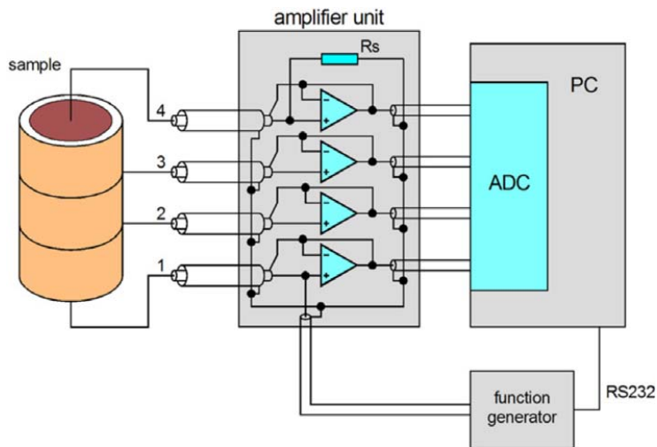
Figure 3-1. Sketch of the four-point measurement system (Zimmermann et al., 2008). Electrodes 1 and 4 are used for current injection and electrodes 2 and 3 are used for voltage measurements
