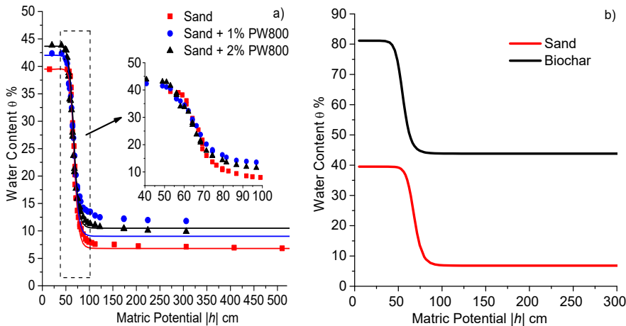
Figure 6-1. Water retention characteristics describing the relationship between water content ( \theta ) and matric potential ( h ) for pure sand and the two sand-biochar mixtures with 1% and 2% PW800 biochar; (a) measured values and fits according to Eq. (6-2) and (6-3) using the curves from (b) for pure sand and pure biochar; (b) fit for pure sand by Eq. (6-2) and modeled curve for pure biochar according to Eq. (6-2) and (6-3) from the fit for the 2% sample.
