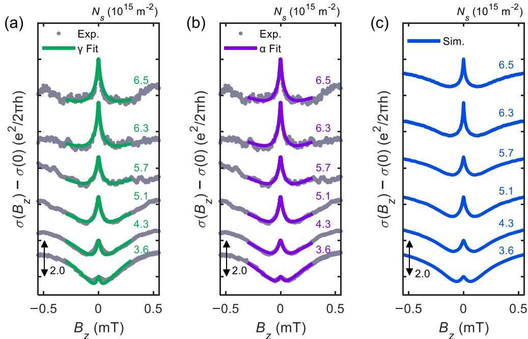
FIG. 12. (a) Measured weak antilocalization (WAL) signals and fits with single common \gamma and individually set L_\phi as fit parameters. (b) Measured signals and fits with |\alpha| and L_\phi as free fit parameters. (c) The real-space simulated WAL curves corresponding to the experiments in each N_s .
