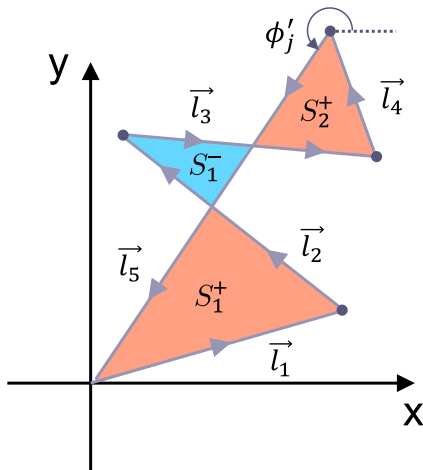
FIG. 8. The j th closed loop of electron trajectory with the number of scatterings n_{\text{scat}} = 5 . This consists of line segments \vec{l}_m with m = 1, 2, \dots, 5 . The encircling area S_j is given by S_j = |S_1^+ + S_2^+ - S_1^-| when S_1^+ , S_2^+ , and S_1^- are defined to be positive.
