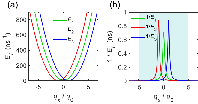
FIG. 6. (a) The Cooperon triplet eigenvalues E_i ( i = 1, 2, 3 ) and (b) their inverse 1/E_i as functions of the wave vector ratio q_x/q_0 at Rashba coefficient \alpha = -2.7 meV Å and Dresselhaus coefficients \beta_1 = 2.3 meV Å, \beta_3 = 0.40 meV Å.
