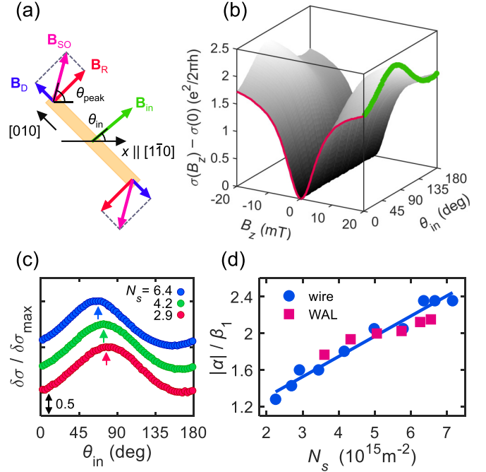
FIG. 4. (a) Schematic orientation of Rashba (red), Dresselhaus (blue), and total spin-orbit (SO) field (pink) and in-plane external magnetic field (green) for [010] -oriented wire. (b) Three-dimensional plot of magnetoconductance \sigma(B_z) - \sigma(0) in [010] -oriented wire structure for various angles of in-plane magnetic field \theta_{in} at gate voltage V_g = 0.0 V ( N_s = 4.2 \times 10^{15} \text{ m}^{-2} ). (c) Weak localization (WL) amplitude \delta\sigma = \sigma(B_z = 20 \text{ mT}) - \sigma(0) is normalized by its maximum \delta\sigma_{max} and plotted (\delta\sigma/\delta\sigma_{max}) as a function of \theta_{in} for carrier densities N_s = 2.9, 4.2 , and 6.4 \times 10^{15} \text{ m}^{-2} . Each signal is vertically shifted for clarity. (d) The ratio between Rashba and linear Dresselhaus SO coefficients |\alpha|/\beta_1 as a function of N_s evaluated from wire measurement (blue) and from SO coefficients on weak antilocalization (WAL) analysis (pink). In wires, considering that 45^\circ < \theta_{peak} < 90^\circ , \alpha < 0 and |\alpha| > \beta_1 are obtained in measured V_g range. The blue solid line shows the linear assumption of |\alpha|/\beta_1 against N_s [ |\alpha|/\beta_1 = R(N_s) = AN_s + C ].
