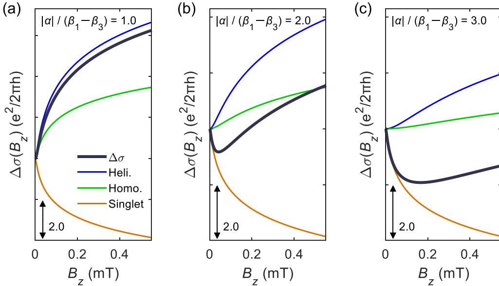
FIG. 7. The magnetoconductance \Delta\sigma(B_z) obtained by Eqs. (3a)–(3d) in the main text (black bold) and its singlet term -e^2\tilde{\Psi}_{\text{singlet}}/4\pi^2\hbar (orange), triplet helical term 2e^2\tilde{\Psi}_{\text{heli}}/4\pi^2\hbar (blue), and triplet homogeneous term e^2\tilde{\Psi}_{\text{homo}}/4\pi^2\hbar (green) for (a) |\alpha|/(\beta_1 - \beta_3) = 1.0 , (b) 2.0, and (c) 3.0.
