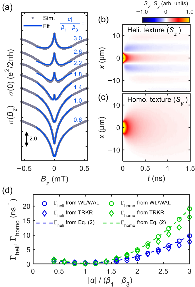
FIG. 2. (a) Real-space simulated magnetoconductance \sigma(B_z) - \sigma(0) (gray) and fits with Eqs. (3a)–(3d) (blue) for various spin-orbit (SO) ratios from |\alpha|/(\beta_1 - \beta_3) = 0.6 to 3.0. Color-scale plot of spatiotemporal evolution of (b) S_z into helical texture and (c) S_y into homogeneous texture at |\alpha|/(\beta_1 - \beta_3) = 1 obtained by Monte Carlo simulation. (d) Relaxation rates of helical \Gamma_{\text{heli}} (blue) and homogeneous \Gamma_{\text{homo}} (green) spin textures extracted from weak localization/weak antilocalization (WL/WAL; circles), time-resolved Kerr rotation (TRKR) simulation (diamonds), and calculated from Eqs. (2a) and (2b) (dashed line) plotted as a function of |\alpha|/(\beta_1 - \beta_3) .
