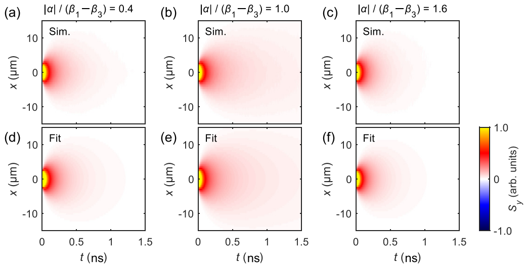
FIG. 10. Color-scale plots of spatiotemporal evolution of S_y into homogeneous textures obtained by Monte Carlo simulation for (a) |\alpha|/(\beta_1 - \beta_3) = 0.4 , (b) 1.0, and (c) 1.6, respectively. (d)–(f) Corresponding fits of S_y to (a)–(c) using Eq. (5b) in the main text.
