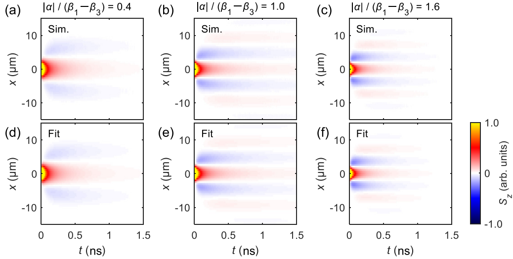
FIG. 9. Color-scale plots of spatiotemporal evolution of S_z into helical textures obtained by the Monte Carlo simulation for (a) |\alpha|/(\beta_1 - \beta_3) = 0.4 , (b) 1.0, and (c) 1.6, respectively. (d)–(f) Corresponding fits of S_z to (a)–(c) using Eq. (5a) in the main text.
