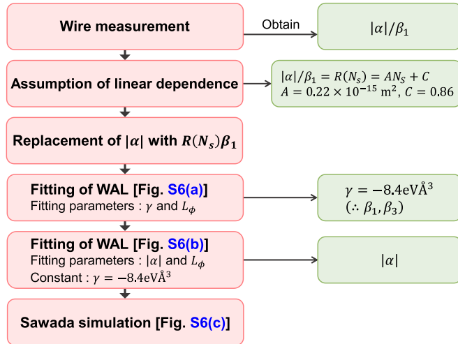
FIG. 11. Flowchart of the extraction of full spin-orbit (SO) coefficients from experimental weak antilocalization (WAL) results by combination of wire measurement.
