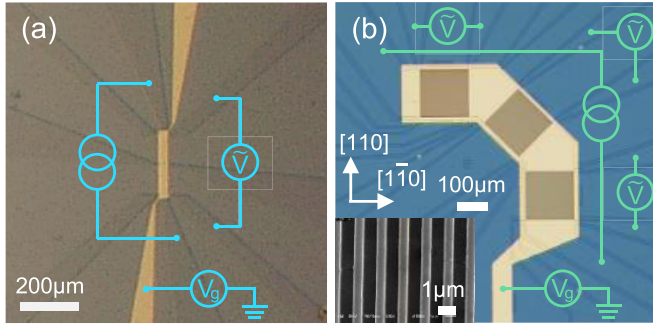
FIG. 3. Optical micrographs of (a) the Hall bar structure and (b) the parallel wire structure. (a) Magnetoconductance was measured in the Hall bar structure to demonstrate the electrical detection of the spin-mode lifetime. (b) Parallel wire structure was prepared along [1\bar{1}0] (left), [010] (middle), and [110] (right) orientations to measure the anisotropic weak localization behavior under in-plane external magnetic field. The [010] -oriented wire was used to evaluate the spin-orbit (SO) ratio \alpha/\beta_1 , as shown in the main text and Fig. 4, while the [1\bar{1}0] - and [110] -oriented wires were for the confirmation of the SO field direction [68,69]. Inset shows a scanning electron microscope image of parallel wire structure.
