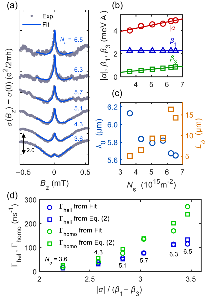
FIG. 5. (a) Measured magnetoconductance \sigma(B_z) - \sigma(0) (gray) and fits with Eqs. (3a)–(3d) (blue) for various carrier densities from N_s = 3.6 to 6.5 \times 10^{15} \text{ m}^{-2} . (b) Full spin-orbit (SO) coefficients |\alpha| , \beta_1 , and \beta_3 as a function of N_s evaluated via weak antilocalization (WAL) analysis in combination with wire measurement. (c) Pitch of the helical texture \lambda_0 (blue) and phase coherence length L_\phi (orange) plotted against N_s . (d) Relaxation rates of helical \Gamma_{\text{heli}} (blue) and homogeneous \Gamma_{\text{homo}} (green) spin textures extracted from the fitting of WAL with Eqs. (3a)–(3d) (circles) and calculated from SO coefficients using Eqs. (2a) and (2b) (square) plotted as a function of |\alpha|/(\beta_1 - \beta_3) . The labeled numerals show the corresponding N_s .
