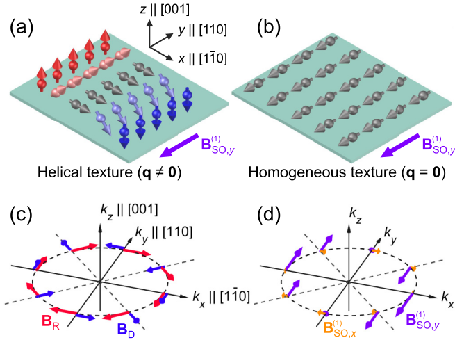
FIG. 1. Schematic view of (a) helical and (b) homogeneous spin textures. (c) Configuration of Rashba (red) and linear Dresselhaus (blue) spin-orbit (SO) field in a (001)-grown quantum well (QW). (d) Near the persistent spin helix (PSH) state, total SO field is dominated by its large y component of SO field B_{SO,y}^{(1)} (purple) with SU(2) symmetry, while small x component B_{SO,x}^{(1)} (orange) breaks the symmetry and cause D'yakonov-Perel' (DP) spin relaxation.
