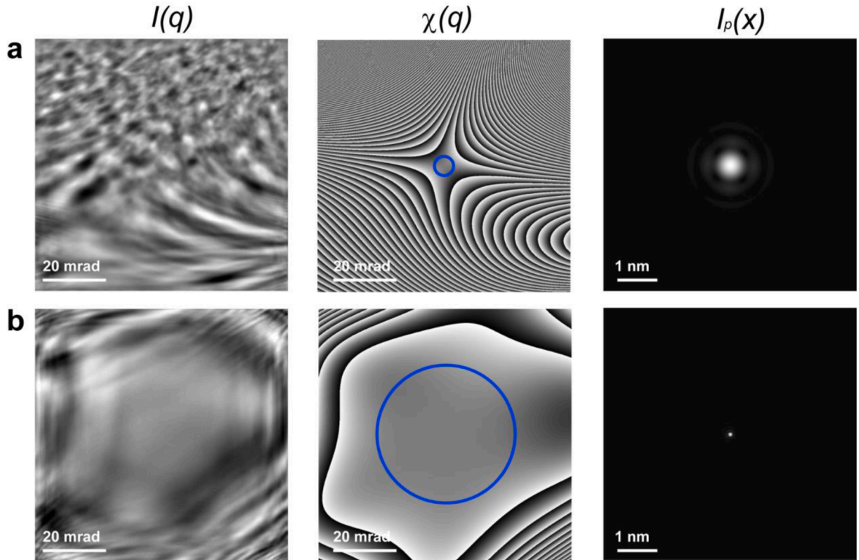
Fig. 4. Simulated images illustrating ANN correction. (a) Uncorrected probe. (b) Corrected probe after subtraction of the aberration values measured using the ANN. (Left) Ronchigram intensity I(q) and (center) corresponding aberration phase \chi(q) calculated at a defocus of C_{1,0} = 0 nm. The blue circle indicates the optimal probe aperture \alpha used to estimate the resolution according to the Rayleigh criterion. (Right) Corresponding calculated probe intensity I_p(x) in vacuum.
