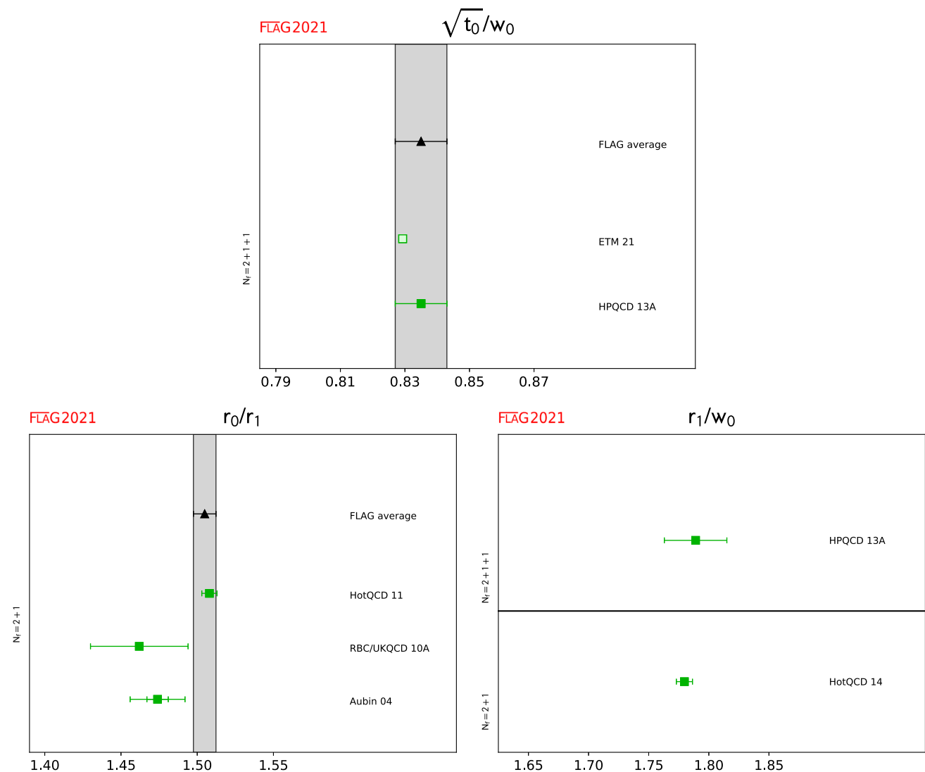
Fig. 53 Results for dimensionless ratios of scales
