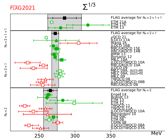
Fig. 14 Cubic root of the SU(2) quark condensate \Sigma \equiv -\lim_{m_u, m_d \rightarrow 0} \langle \bar{u}u \rangle in the \overline{\text{MS}} -scheme, at the renormalization scale \mu = 2 GeV. Square symbols indicate determinations from correlators in the p -regime, up triangles refer to extractions from the topological susceptibility, diamonds to determinations from the pion form factor, and bullet points refer to the spectral density method
