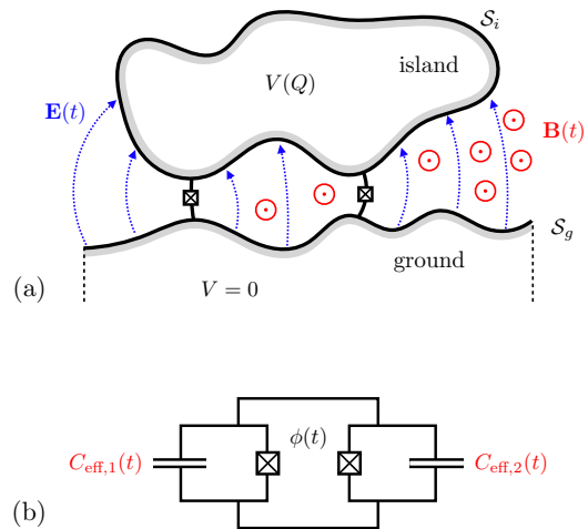
Figure 1. Some of the main accomplishments of this work. (a) We develop a recipe to derive the correct time-dependent Hamiltonian for circuits with a general geometry, taking as input the time-dependent magnetic field \mathbf{B}(t) (red), from which the time-dependent electric field \mathbf{E}(t) (blue) is derived. (b) We find that in this general case, it is not always possible to assign well-behaved capacitances to the two Josephson junctions of a SQUID. While the total capacitance C_{\text{tot}} = C_{\text{eff},1}(t) + C_{\text{eff},2}(t) is guaranteed to be constant in time and positive definite, if we force a mapping to a model with effective junction capacitances C_{\text{eff},j}(t) , these may be negative, time-dependent or even momentarily singular.
