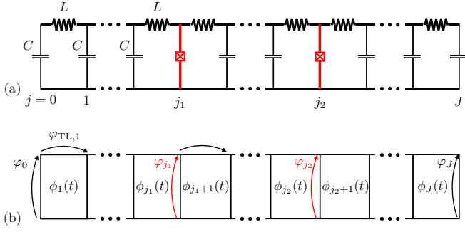
Figure 4. (a) Finite element model to describe the SQUID geometry in Fig. 3(a). The upper arm of the SQUID is described through a transmission line, whereas the lower arm is simply a ground. The Josephson junctions (red) are at positions j = j_1 and j = j_2 . (b) The same finite element model, now showing the temporally and spatially varying flux \phi_j(t) , as well as the branch phase variables for the transmission line, \varphi_{TL,j} , and the ones describing the capacitive and Josephson coupling between ground and transmission line, \varphi_j .
