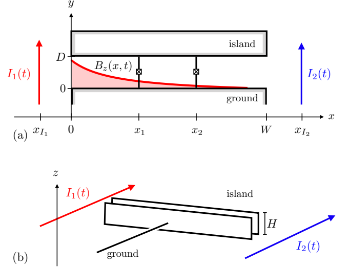
Figure 3. Sketch of the simple SQUID circuit with two magnetic field sources. The setup as shown in this figure leads to all the predicted effects in the main text, such as negative capacitances, or time-dependent capacitances. (a) Top view of the SQUID circuit. The ground and island form a parallel plate capacitor with distance D ( y -direction) and width W \gg D ( x -direction). Two current wire sources I_1 (red) and I_2 (blue) produce magnetic fields. We indicate the spatial distribution of the field for the first source (red curve). The Josephson junctions are placed at positions x_1 and x_2 , 0 < x_{1,2} < W while the sources are placed at x_{I_1} < 0 and x_{I_2} > W . Note that for illustration purposes, the y -axis is exaggerated; in the actual model both the plate distance D and the plate thicknesses should be much smaller than any of the length scales in x direction. (b) In z -direction the planes are of a height H which is large with respect to the distance, H \gg D , but small with respect to the width H \ll W .
