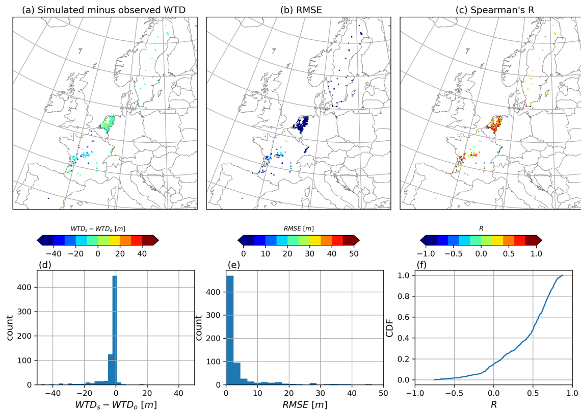
Figure 9. (a) Difference in observed and ParFlow-CLM-simulated WTD at filtered locations ( N = 720 ), (b) RMSE values at filtered locations and (c) Spearman correlation ( R ) values at selected locations. Histogram plots show the distribution of (d) simulated minus observed WTD and (e) RMSE values. (f) Cumulative distribution function (CDF) of Spearman correlation of ParFlow-CLM with observed WTD data.
