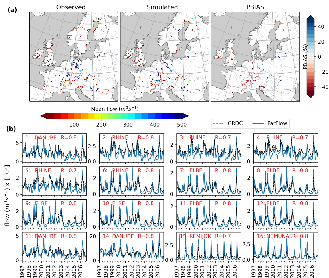
Figure 2. (a) Comparison of observed and simulated average discharge and the percentage bias in monthly discharge (PBIAS) for 176 gauging stations. (b) Comparison of time series of observed and simulated discharge for selected large rivers with drainage areas greater than 50 000 km 2 . Locations of selected gauges in (b) are indicated with corresponding numbers in the left panel of (a).
