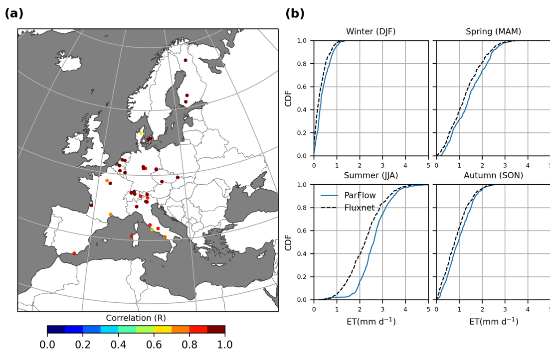
Figure 5. Evaluation of ParFlow-CLM-simulated monthly evapotranspiration (ET) with ground-based observations from 60 eddy covariance FLUXNET stations. (b) Comparison of cumulative distribution of seasonal ET estimated by ParFlow-CLM with FLUXNET stations.
