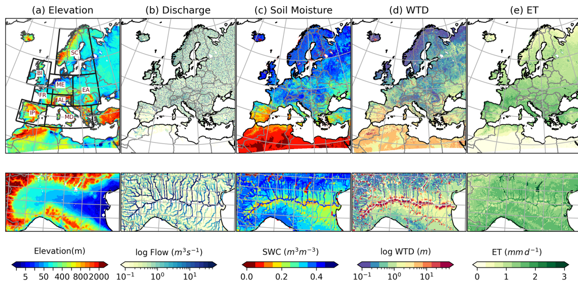
Figure 1. Maps of EURO-CORDEX domain at 3 km resolution ( 1544 \times 1592 grid cells) showing spatially averaged distribution of (a) elevation, (b) discharge, (c) surface soil moisture, (d) water table depth and (e) evapotranspiration (1997–2006), along with close-ups of the Po River basin in the Alpine (AL) region simulated by ParFlow-CLM model. Red color in (d) indicates deeper water table with maximum of 51 m depth. The black boxes in (a) correspond to PRUDENCE regions, with their common abbreviations indicating names of the regions (FR: France; ME: mid-Europe; SC: Scandinavia; EA: eastern Europe; MD: Mediterranean; IP: Iberian Peninsula; BI: the British Isles; AL: Alpine).
