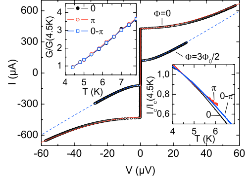
FIG. 8. (Color online) I - V characteristics of a reference 0 junction (#1 in Table I) at T \approx 4.5 \text{ K} and applied magnetic flux \Phi=0 and \frac{3}{2}\Phi_0 , i.e., at the principal maximum and first side maximum of I_c(B) . Lines correspond to the RSJ curve [Eq. (A8)], with I_c=428(118) \text{ } \mu\text{A} and G=8.6(9.7) \text{ } \Omega^{-1} for \Phi=0 ( \frac{3}{2}\Phi_0 ). Upper left inset shows normalized conductances G/G(4.5 \text{ K}) vs T for a 0 , \pi and 0-\pi junction; G(4.5 \text{ K}) \approx 9.5 \text{ } \Omega^{-1} for the 0 and 0-\pi junction, and \approx 9.3 \text{ } \Omega^{-1} for the \pi junction. Lower right inset shows I_c(T) at \Phi=0 , normalized to I_c(4.5 \text{ K})=420, 170 , and 124 \text{ } \mu\text{A} for the 0 , \pi , and 0-\pi junction, respectively. All junctions have dimensions of 10 \times 50 \text{ } \mu\text{m}^2 .
