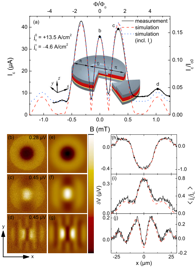
FIG. 5. (Color online). Disk shaped 0- \pi junction No. 6 in Table I: (a) I_c(B) with B \parallel y . Solid (black) curve shows experimental data; dashed (red) curve is calculated using Eq. (9); dotted (blue) curve is calculated using Eq. (13). Inset shows the junction geometry. (b)–(d) LTSEM images \delta V(x,y) (Ref. 57) taken at bias points indicated in (a). (e)–(g) corresponding images \langle j_s \rangle(x,y)/j_c^0 calculated using Eq. (5). (h)–(j) line scans: solid (black) lines \delta V(x) are extracted from the corresponding LTSEM images at y=0 ; dashed (red) lines \langle j_s \rangle(x)/j_c^0 are calculated using Eq. (5).
