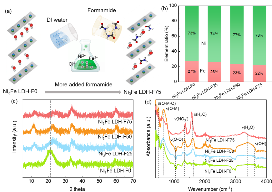
Figure 5.1 (a) Illustration of the synthesis process of NiFe LDH with formamide. (b) elemental ratio of Ni/Fe in the NiFe LDH-F samples. (c) XRD and (d) IR spectra of NiFe LDH-F samples.
