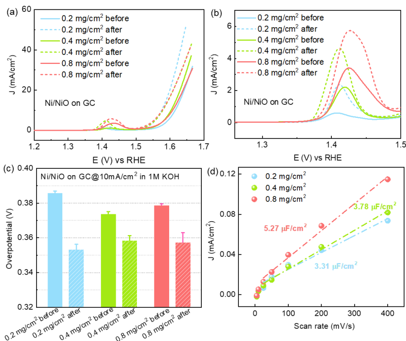
Figure 3.13 OER polarization curves of the Ni/NiO catalyst in 1 m KOH solution with different loadings on GC: 0.2, 0.4 and 0.8 mg/cm 2 . The corresponding (b) amplifying of Ni oxidation region, (c) overpotentials@10 mA/cm 2 and (d) ECSA tests.
