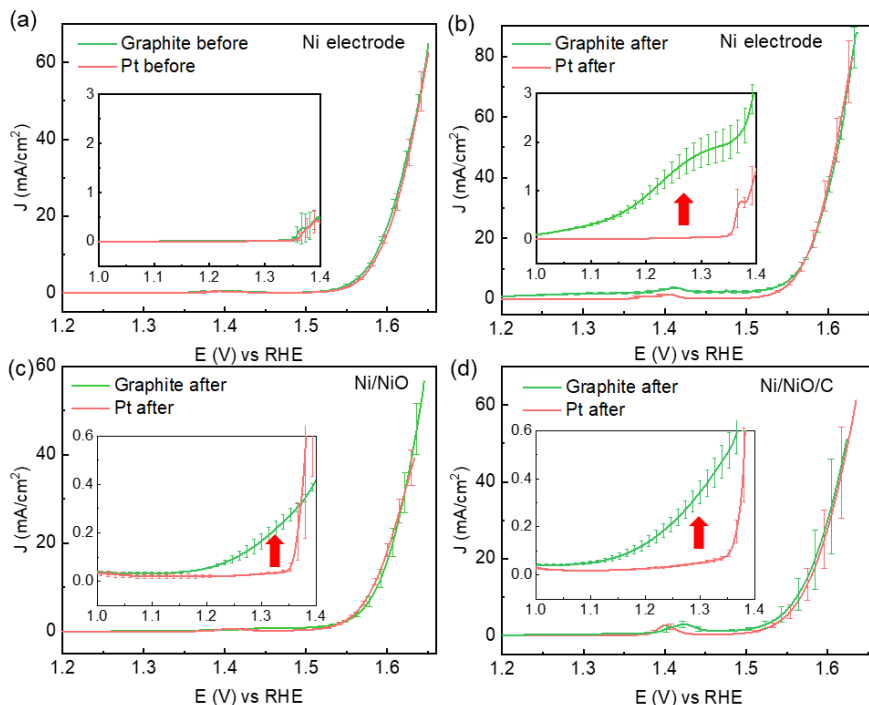
Figure 3.7 Polarization curves of (a,b) Ni electrode, (c) Ni/NiO and (d) Ni/NiO/C samples by two different counter electrodes before (a) and after (b-d)1000 cycling process, including: graphite rod (green) and Pt (red); inserted figures are the corresponding magnification area before nickel redox peak, the added red arrow is the indication of increased current at 1.0-1.4 V after cycling when using graphite as counter electrode.
