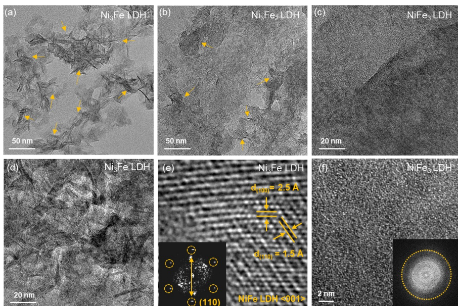
Figure 4.4 Microscopy investigation of the NiFe LDH catalysts. (a-c) TEM images of the \text{Ni}_3\text{Fe} , \text{Ni}_3\text{Fe}_2 and \text{NiFe}_3 LDHs (stacked LDH layers are marked by yellow arrows). (d-f) high-resolution TEM images of \text{Ni}_3\text{Fe} LDH (d-e) and \text{NiFe}_3 LDH (f). The insets in (e-f) show the Fourier transform of the region.
