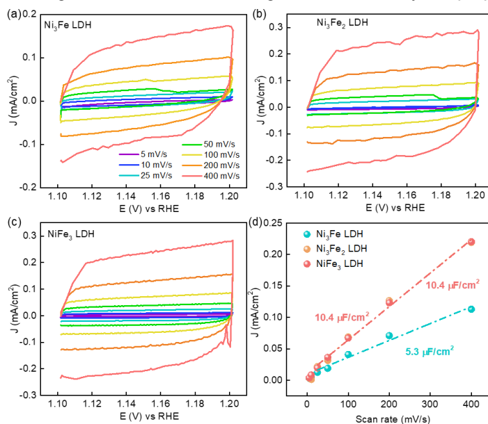
Figure 4.13 Double-layer capacitance measurements for determining electrochemically active surface area for NiFe LDHs from voltammetry in 1 M KOH. (a-c) Cyclic voltammograms of \text{Ni}_3\text{Fe} LDH, \text{Ni}_3\text{Fe}_2 LDH and \text{NiFe}_3 LDH were measured in a non-Faradaic region of the voltammogram at the following scan rates: 5, 10, 25, 50, 100, 200, 400 \text{mV}/\text{s} . (d) The specific capacitance of NiFe LDHs calculated by the slope of the linear fits from the current densities at various scan rates.
