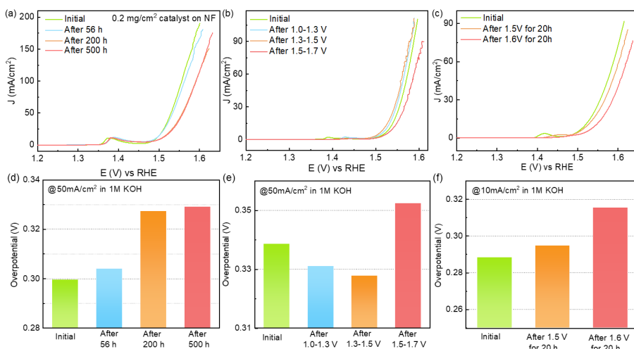
Figure 5.4 Extended stability test of NiFe LDH-F75 catalyst. (a-c) LSV curves before and after (a) keeping at 1.6 V for certain hours, (b) 5000 cycles between different ranges, and (c) keeping at certain potentials for 20 hours, (d-f) the corresponding comparison of overpotentials from (a-c) respectively.
