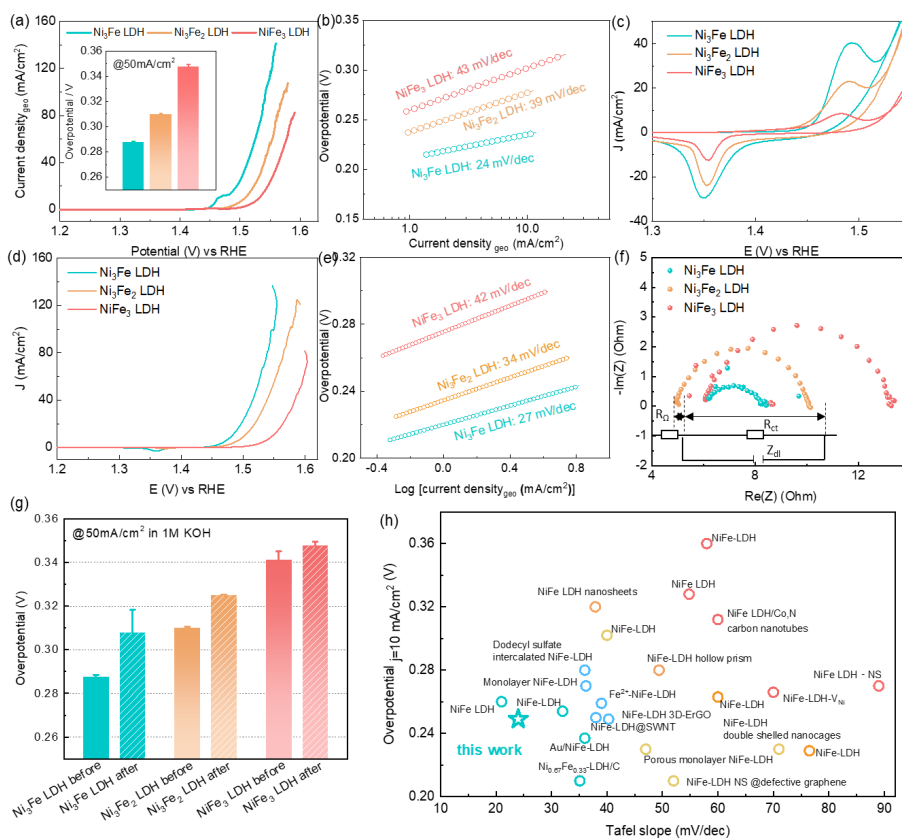
Figure 4.9 (a) Polarization curves of NiFe LDHs. (Inset: the overpotential at 50 \text{mA/cm}^2 ). (b) Tafel slopes. (c) the nickel redox peak. (d) Polarization curves and (e) Tafel slopes at negative scans. (f) impedance spectroscopy at 1.7 V of NiFe LDHs. (g) Overpotential changes after 1000 cycles from 1.0-1.7 Vs. (h) Summary of various NiFe LDH catalysts and corresponding OER activities by the overpotentials at 10 \text{mA/cm}^2 and Tafel slope.
