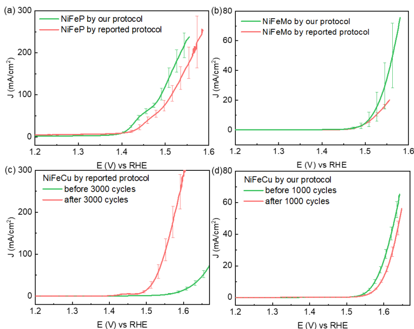
Figure 3.25 OER activity of three typical Ni-based catalysts. (a) NiFeP nanoplate arrays, (b) amorphous NiFeMo oxides and multi-metal-site NiFeCu oxyhydroxide by (c) reported protocols and (d) our testing protocols. Different scales of these figures are used due to the distinct performance of these catalysts.
