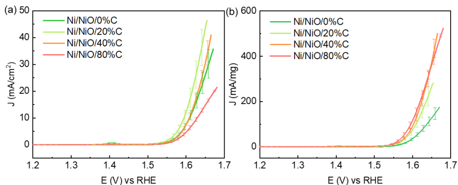
Figure 3.1 Comparison of Ni/NiO with various ratio carbon electrodes. Nominal activity normalized by geometry area (a) and mass activity normalized by rough mass of nickel (b) in Ni/NiO nanoparticles with 0, 20%, 40% and 80% mass ratio XC-72 carbon.
