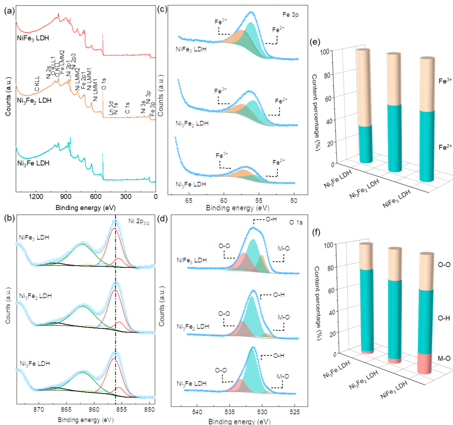
Figure 4.6 XPS spectra of NiFe LDHs. (a) survey profile, Core-level (b) Ni 2p region, (c) Fe 3p region and (d) O 1s region. (e-f) Corresponding Fe and O content from (c) and (d).
