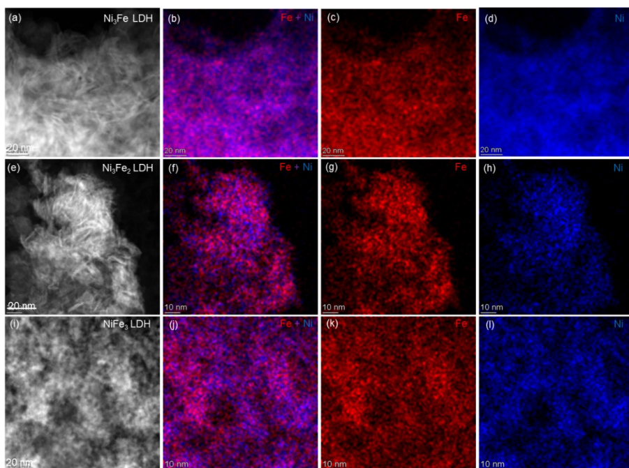
Figure 4.5 HAADF-STEM images and elemental mapping of Ni and Fe distribution in NiFe LDH nanocrystals, (a-d) \text{Ni}_3\text{Fe} LDH, (e-h) \text{Ni}_3\text{Fe}_2 LDH and (i-l) \text{NiFe}_3 LDH.
