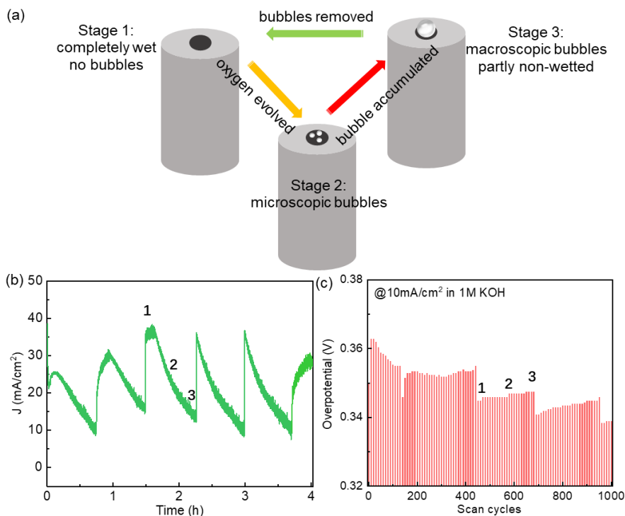
Figure 3.5 (a) illustration of dynamic cycling of bubble formation, accumulation, and elimination during stability tests, (b) CA curves of Ni electrode at 1.6 V over time, (c) overpotentials of CV curves from 1st to 1000th cycles.
