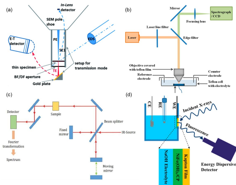
Figure 2.3 Illustration of various characterization techniques. (a) SEM and EDX system. 126 (b) Raman spectroscopy. 127 (c) FTIR spectrometer. 128 (d) In situ XAS setup scheme. 129
