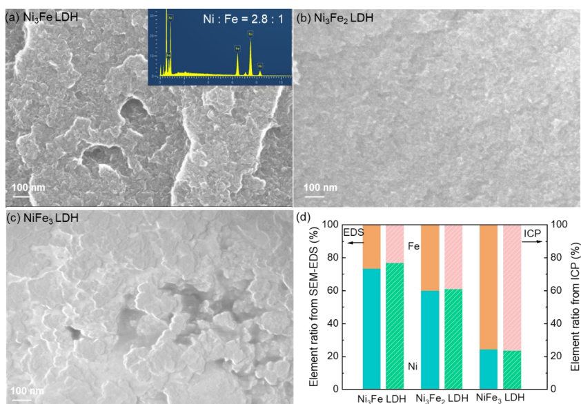
Figure 4.2 (a-c) SEM images of \text{Ni}_3\text{Fe} LDH, \text{Ni}_3\text{Fe}_2 LDH and \text{NiFe}_3 LDH. (d) Element ratio of Ni/Fe in NiFe LDHs by EDX (solid filled bars) and ICP (pattern filled bars).
