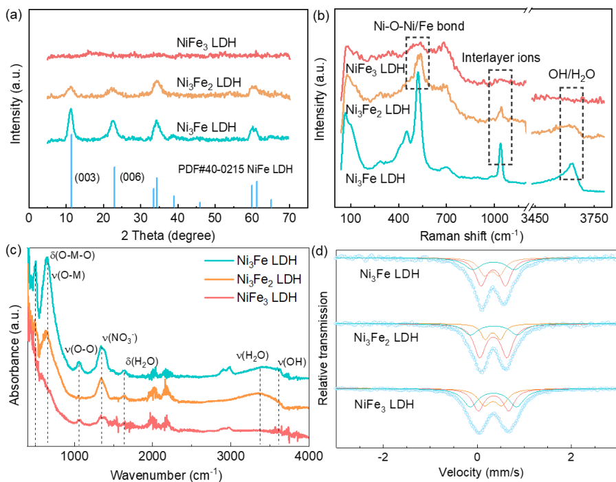
Figure 4.3 Structural characterizations of the NiFe LDH catalysts. (a) XRD patterns, (b) Raman spectra, (c) IR spectra and (d) Mossbauer spectra.
