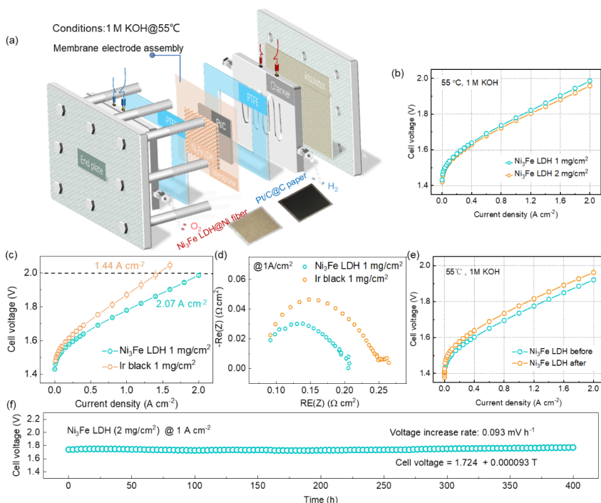
Figure 4.11 Single cell performance of Ni 3 Fe LDH catalyst. (a) Schematic illustration of the electrolyzer cell. (b) Polarization curve of the cells using Ni 3 Fe LDH catalysts as anode with loadings of 1 and 2 mg/cm 2 . (c) Polarization curve of the cell based on Ni 3 Fe LDH@Ni fiber electrode with commercial Ir black @ Ni fiber electrode as an anode, respectively. (d) (e) Polarization curve and (f) galvanostatic curve of water electrolysis using 2 mg/cm 2 Ni 3 Fe LDH catalysts as anode before and after the 400 h at 1 A/cm 2 .
