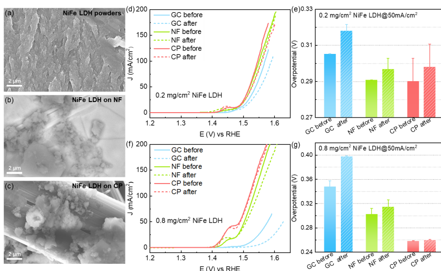
Figure 3.20 (a-c) SEM images of the NiFe LDH catalysts on various substrates. (a) initial NiFe LDH powders, NiFe LDH on (b) NF and (c) CP. The corresponding (d,f) OER polarization curves and (e,g) overpotentials@50 mA/cm 2 before and after cycling between 1.0-1.7 V for 1000 cycles in 1M KOH. Among them, (d,e) the loading of NiFe LDH is 0.2 mg/cm 2 while (f,g) the loading of NiFe LDH is 0.8 mg/cm 2 .
