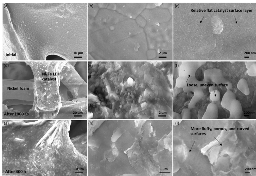
Figure 4.15 SEM image of \text{Ni}_3\text{Fe} LDH catalysts after stability tests. (a-c) initial sample, (d-f) after 1000 cycles between 1.0-1.7 V and (g-i) keeping at 1.6 V for over 400 hours in 1M KOH. The \text{Ni}_3\text{Fe} LDH are drop-casted on nickel foam with the loading of 0.2 \text{ mg/cm}^2 .
