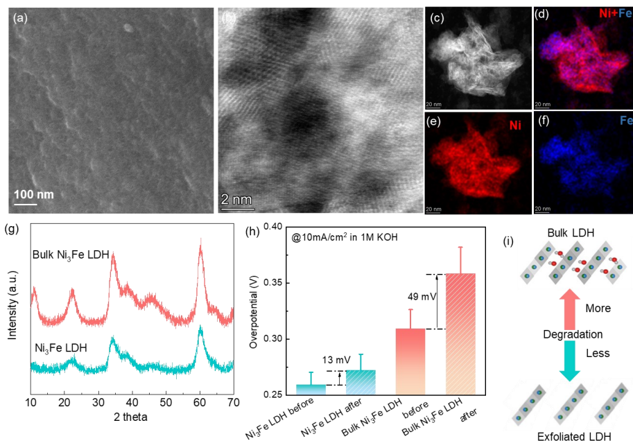
Figure 4.17 (a-f) Electron microscopy of bulk Ni 3 Fe LDH. (a) SEM image, (b) STEM image, (c-f) STEM EDX mapping of Ni and Fe distribution. (g) XRD comparison of exfoliated Ni 3 Fe LDH and bulk Ni 3 Fe LDH. (h) the overpotential at 10 mA/cm 2 of Ni 3 Fe LDH and bulk Ni 3 Fe LDH during 1000 cycles between 1.0-1.7 V in 1M KOH. (i) the illustration of the correlation from the layer structure of LDH with its degradation degree.
