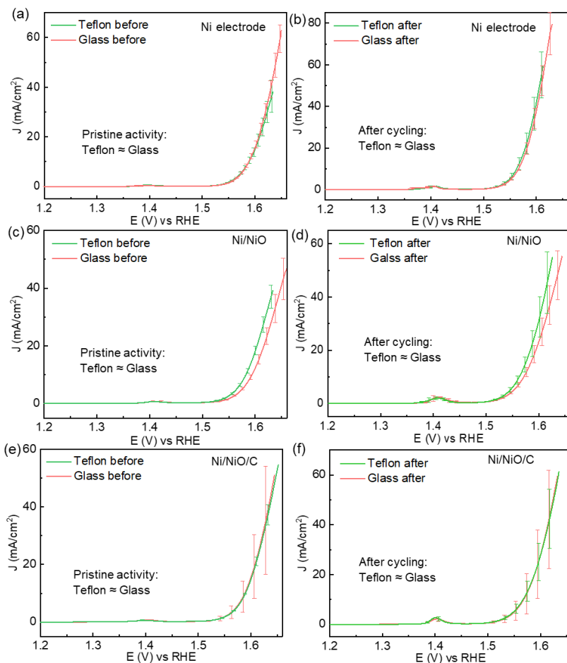
Figure 3.8 Polarization curves of (a,b) Ni electrode, (c,d) Ni/NiO and (e,f) Ni/NiO/C samples by two different cells before (a,c,e) and after (b,d,f) 1000 cycling process, including: Teflon cell b (green) and glass cell (red).
