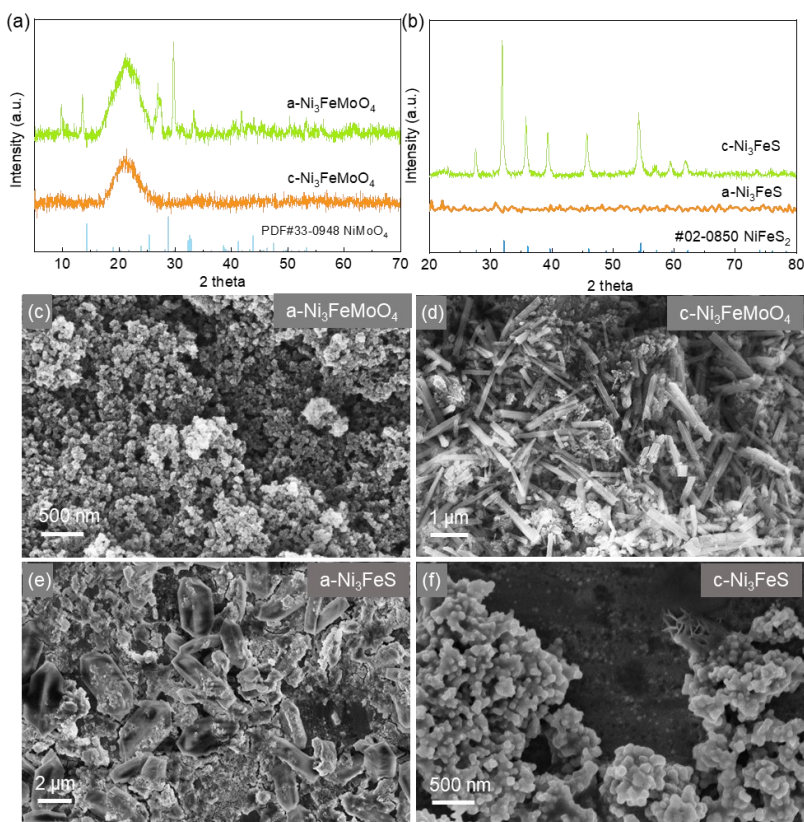
Figure 5.15 XRD patterns of (a) amorphous and crystalline \text{Ni}_3\text{FeMoO}_4 , (b) amorphous and crystalline \text{Ni}_3\text{FeS} . (c-f) SEM images of (c) amorphous and (d) crystalline \text{Ni}_3\text{FeMoO}_4 , (e) amorphous and (f) crystalline \text{Ni}_3\text{FeS} samples.
