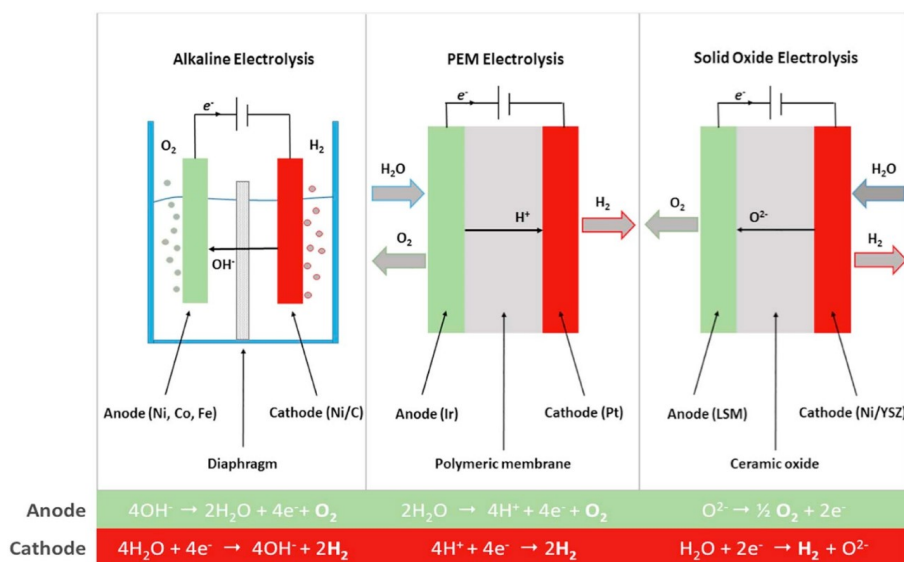
Figure 1.2 Illustration of three kinds of water electrolyzers, alkaline, PEM and SOE. 2
