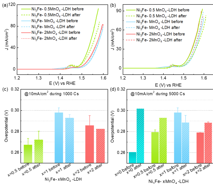
Figure 5.8 (a,b) Polarization curves and (c,d) corresponding overpotentials at 10 mA/cm 2 of Ni 3 Fe-xMnO 4 -LDH catalysts before and after (a,c) 1000 and (b,d) 5000 cycles between 1.0-1.7 V in 1 M KOH.
