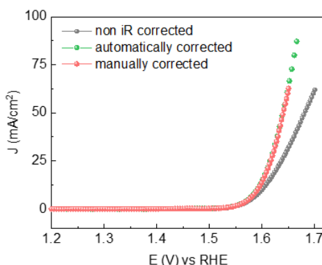
Figure 3.2 LSV curves of a Ni-based electrode in 1 M KOH without and with 85% iR drop compensation manually corrected or automatically corrected using the potentialstat.
