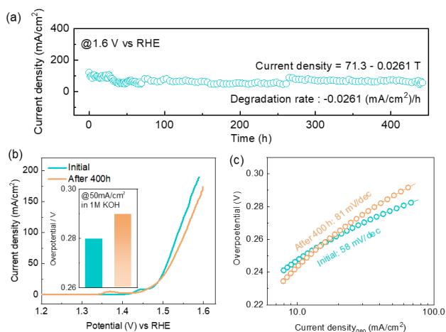
Figure 4.10 (a) Potentiostatic stability of the Ni 3 Fe LDH at 1.6 V for over 400 hours. (b) Corresponding LSV curves and overpotentials (inset), (c) Tafel slope during this process.
