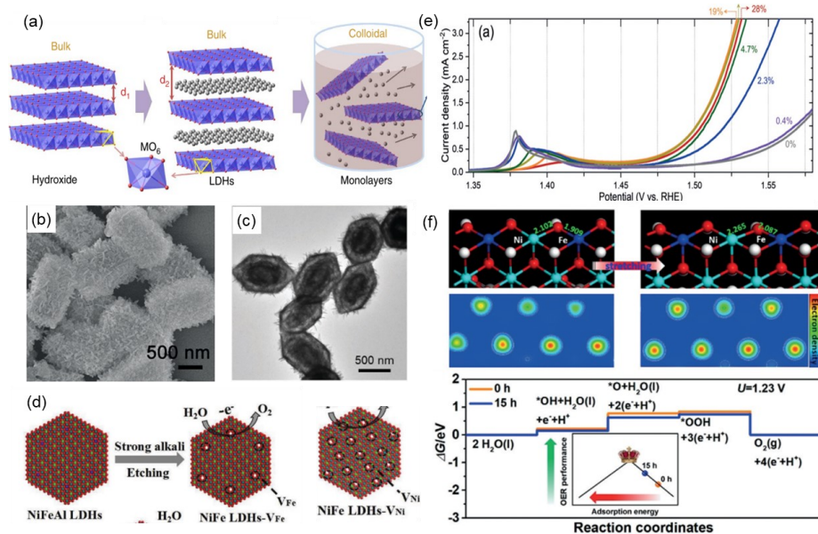
Figure 1.11 Summary of reported approaches to improve the OER activities of NiFe LDHs. (a) Illustration of exfoliation process to peel off bulk LDHs into monolayers. 102 (b,c) morphology design of NiFe LDH (b) hollow prisms 104 and (c) double-shelled nanocages. 105 (d) introduction of cation vacancies in NiFe LDHs. 106 (e) LSV curves of NiFe LDHs with various Ni/Fe ratio. 107 (f) The strain effect on OER performance of NiFe LDH. 108
