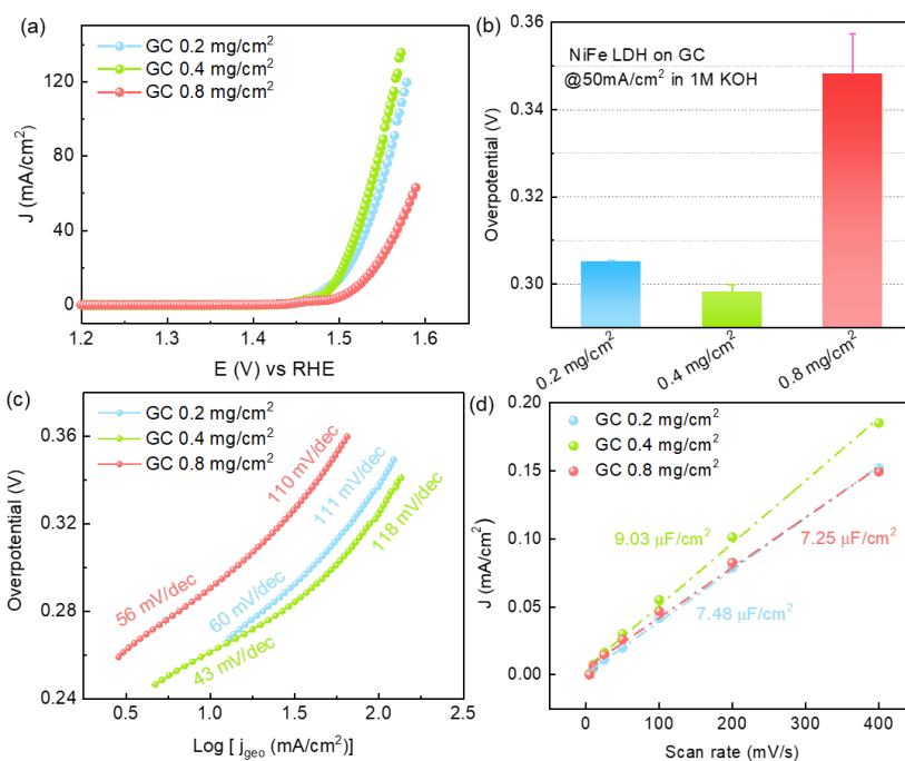
Figure 3.12 OER polarization curves of the NiFe LDH catalysts in 1 M KOH solution with different loadings on GC: 0.2, 0.4 and 0.8 mg/cm 2 . The corresponding (b) overpotentials@50 mA/cm 2 , (c) Tafel slopes and (d) ECSA tests.
