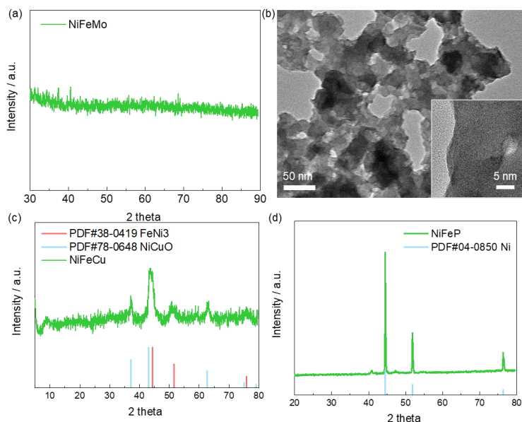
Figure 3.24 Characterization of synthesized Ni-based materials. (a) XRD pattern and (b) TEM images of amorphous NiFeMo. XRD pattern of (c) NiFeCu and (d) NiFeP.
