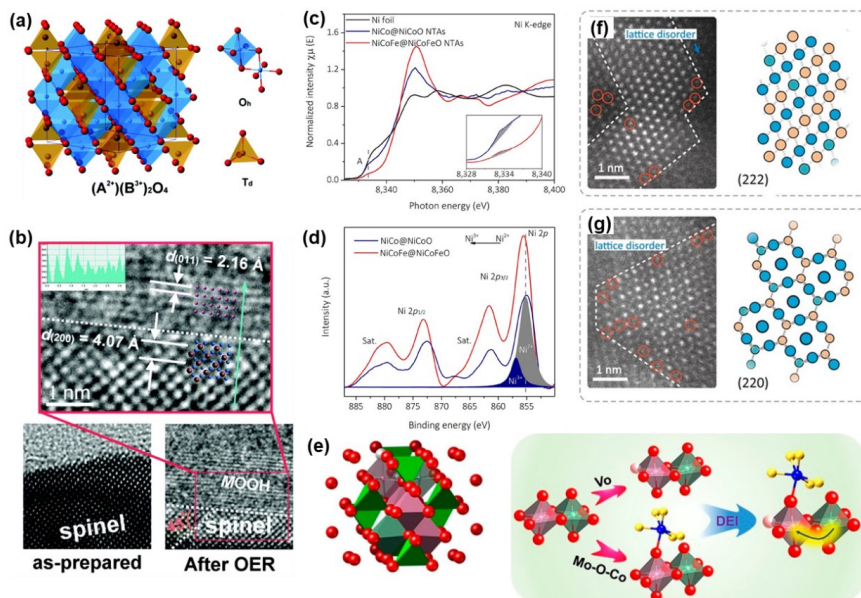
Figure 1.7 Ni-based spinel electrocatalysts. (a) Crystal structure of the spinel AB_2O_4 and corresponding octahedral sites ( O_h ) and tetrahedral sites ( T_d ). (b) HRTEM analysis of NiFe_2O_4 nanocubes before/after oxygen evolution reaction. 56 (c,d) XAS and XPS spectra of Ni in the incorporation of Fe into the binary Ni-Co inverse spinel NiCoFe@NiCoFeO . 104 (e) the creation of double-exchange interaction in spinel NiCo_2O_4 . 52 (f,g) HAADF images of cycled Zn_{0.4}Ni_{0.6}Co_2O_4 nanoparticles. 55
