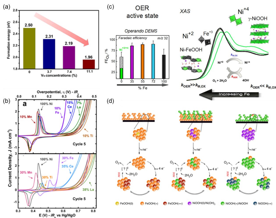
Figure 1.5 Ni-based oxyhydroxides. (a) The calculated formation energies for \gamma -NiOOH from \alpha -Ni(OH) 2 with different V_{\text{Ni}} concentrations. 19 (b) Voltammetry \text{Ni}_{1-z}\text{M}_z\text{O}_x\text{H}_y films, where M is a metal cation, at approximately upper z \approx 0.1 and lower z \approx 0.3 . 56 (c) The role of Fe in mixed NiFe catalysts. The presence of Fe could promote a stabilization of low-valent Ni centers, and enhance the OER rate k_{\text{OER}} , which may exceed the rate of the metal oxidation k_{\text{M,OX}} . 28 (d) schematic representations of the water oxidation process based on the experimental observations herein for FeOOH. 29
