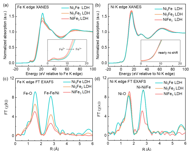
Figure 4.7 XAS spectra of the NiFe LDH catalysts. Normalized XANES spectra of (a) Fe K edge and (b) Ni K edge of NiFe LDHs. EXAFS r-space spectra of the (c) Fe K edge and (d) Ni K edge of NiFe LDHs. The r-space spectra were Fourier-transformed from Ni and Fe K-edge k^3 -weighted EXAFS spectra.
