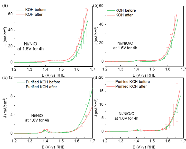
Figure 3.11 Potentiostatic stability of Ni/NiO and Ni/NiO/C catalysts. (a-d) polarization curves of (a,c) Ni/NiO and (b,d) Ni/NiO/C samples in KOH (a,b) and purified KOH (c,d) before and after potentiostatic test at 1.6 V vs RHE for 4 hours, LSV before (green) and LSV after (red). Different scales are chosen to present the OER performance of the catalysts in electrolytes.
