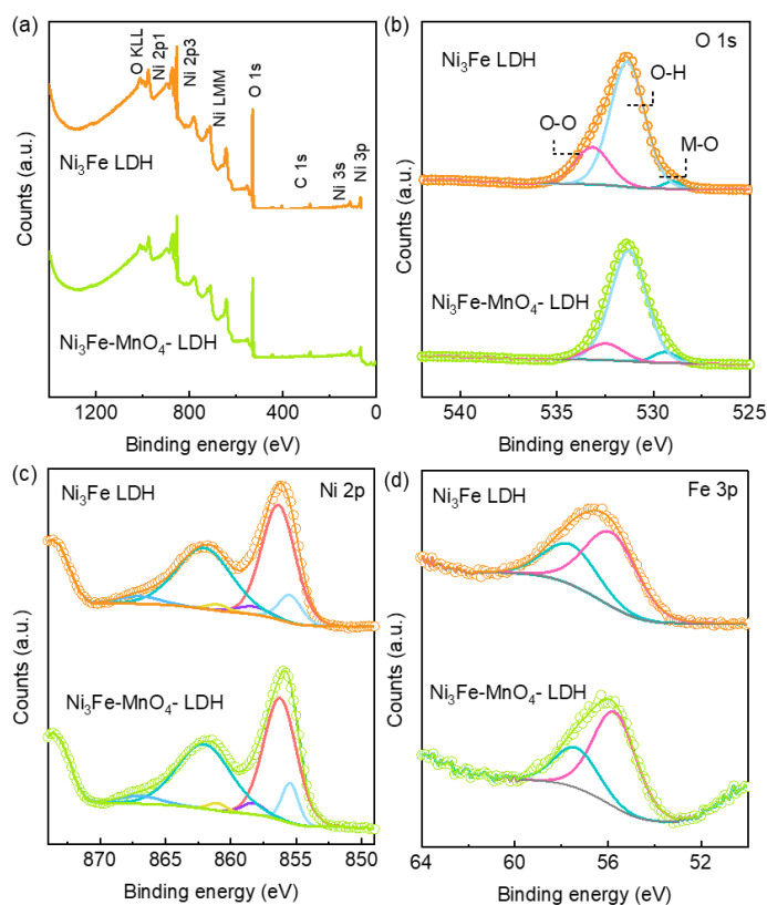
Figure 5.7 XPS spectra of \text{Ni}_3\text{Fe-MnO}_4\text{-LDH} and \text{Ni}_3\text{Fe} LDH samples. (a) survey spectra. (b) O 1s region. (c) Ni 2p region. (d) Fe 3p region.
