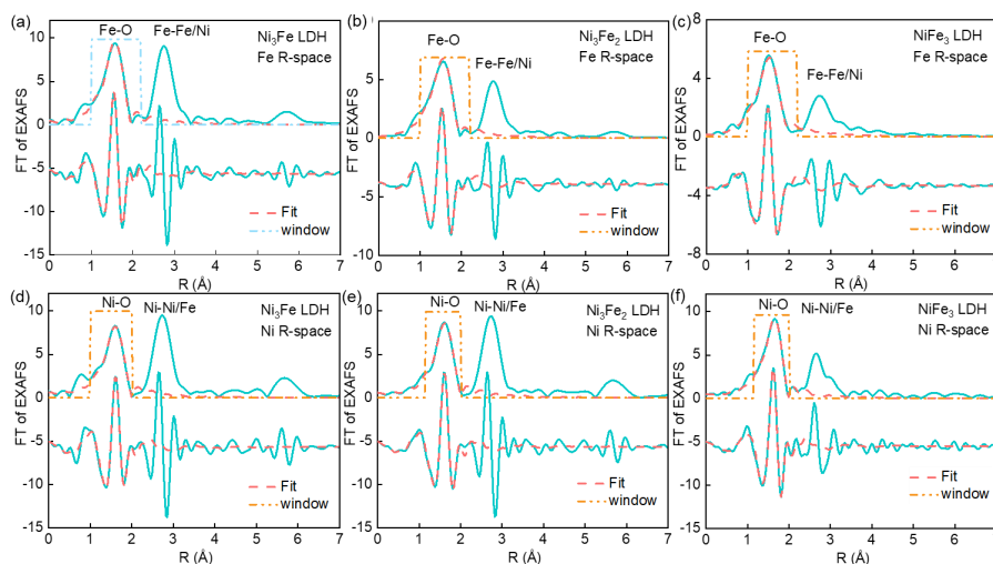
Figure 4.8 Fe K-edge (a-c) and Ni K edge (d-f) Fourier-transformed EXAFS spectra and the fitting results of NiFe LDHs. (a,d) \text{Ni}_3\text{Fe} LDH, (b,e) \text{Ni}_3\text{Fe}_2 LDH, (c,f) \text{NiFe}_3 LDH.
