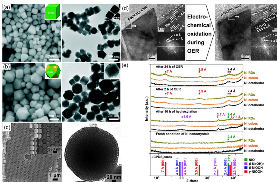
Figure 1.4 Ni nanocrystal electrocatalysts. (a,b) SEM and TEM image of (a) Ni nanocubes and (b) Ni cuboctahedra. 10 (c) SEM image of 3D ordered mesoporous Ni sphere arrays and TEM image of one of the mesoporous Ni spheres. 11 (d,e) Structural analyses of heteroepitaxial \beta -Ni(OH) 2 and \beta -NiOOH phases on Ni. (d) HRTEM images of the Ni octahedron after hydroxylation and after OER stability for 2 h. (e) Magnified XRD spectra of the Ni nanocrystals with different shapes under different conditions. 13
