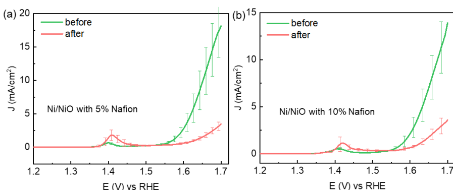
Figure 3.10 LSV curves of Ni/NiO catalysts with different ratio (a) 5\% , (b) 10\% Nafion before and after 1000 cycles between 1.0 - 1.7 V.
