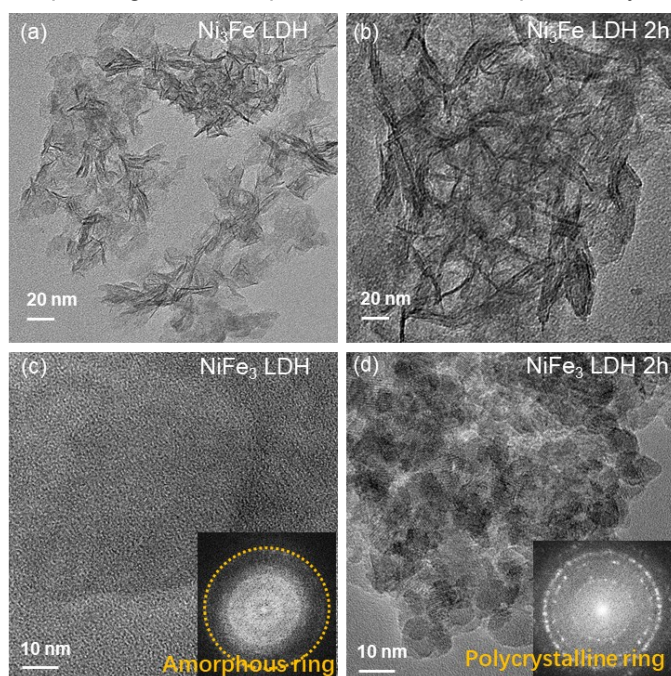
Figure 5.13 TEM images of NiFe LDH (a,c) before and (b,d) after hydrothermal treatment. (a,b) \text{Ni}_3\text{Fe} LDH. (c,d) \text{NiFe}_3 LDH.
