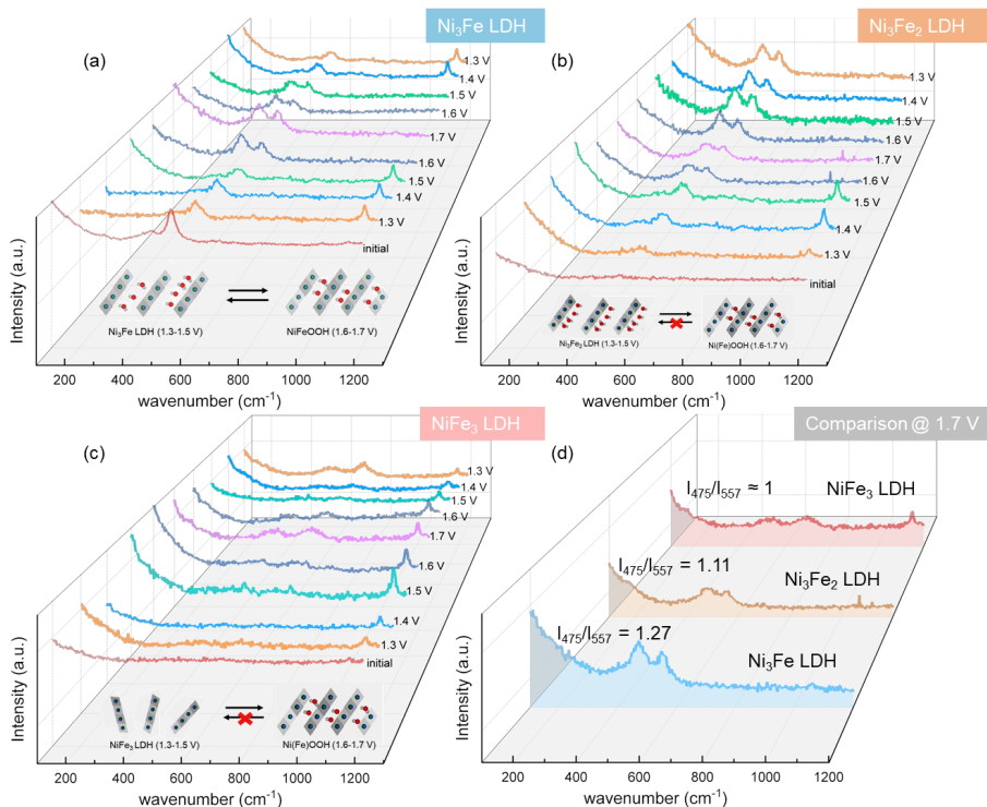
Figure 4.14 In-situ Raman spectra of the NiFe LDH catalysts. Spectra were obtained after keeping initial sample at different potentials in sequence: 1.3 V, 1.4 V, 1.5 V, 1.6 V, 1.7 V, 1.6 V, 1.5 V, 1.4 V, 1.3 V. (a) Ni 3 Fe LDH, (b) Ni 3 Fe 2 LDH and (c) NiFe 3 LDH. (d) Comparison of the Raman band for NiFe LDHs at high potential 1.7 V and the corresponding value of the I_{475}/I_{557} band ratio.
