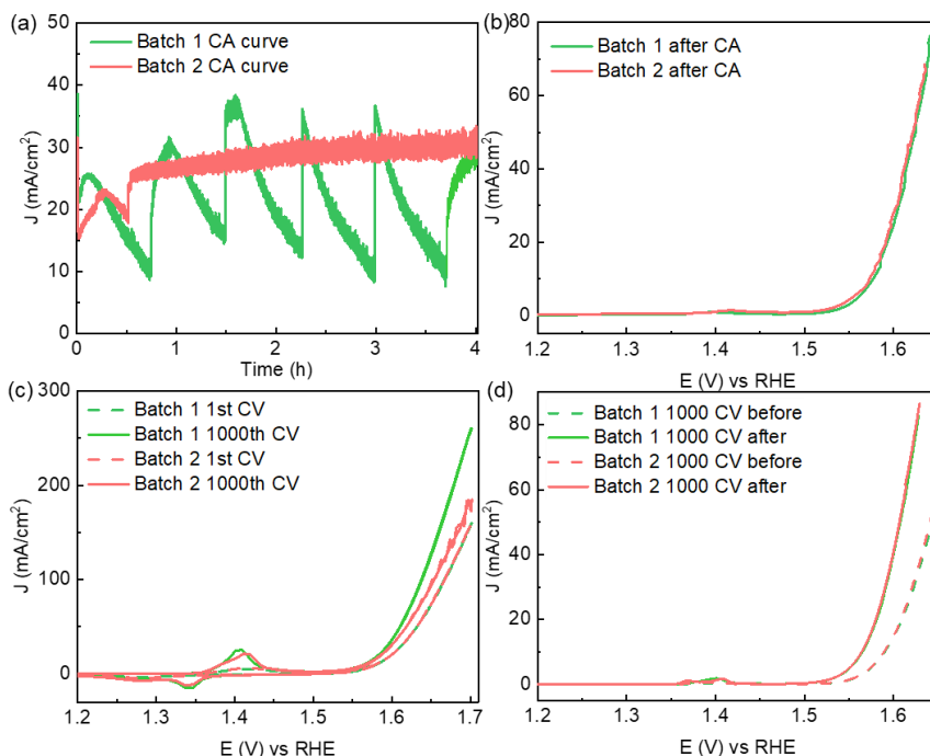
Figure 3.6 (a) CA curves of Ni electrode of two batches at 1.6 V for 4 hours and (b) the corresponding LSV curves after CA process. Although the CA curves show big difference, which may lead to inaccurate evaluation of stability, LSV curve present consistent trend, so these verify the advantage of taking LSV to compare stability, not direct CA curves. (c) 1 st and 1000 th CV curves of Ni electrode of two batches during the cycling between 1.0-1.7 V and (d) the corresponding LSV curves after these 1000 cycling process.
