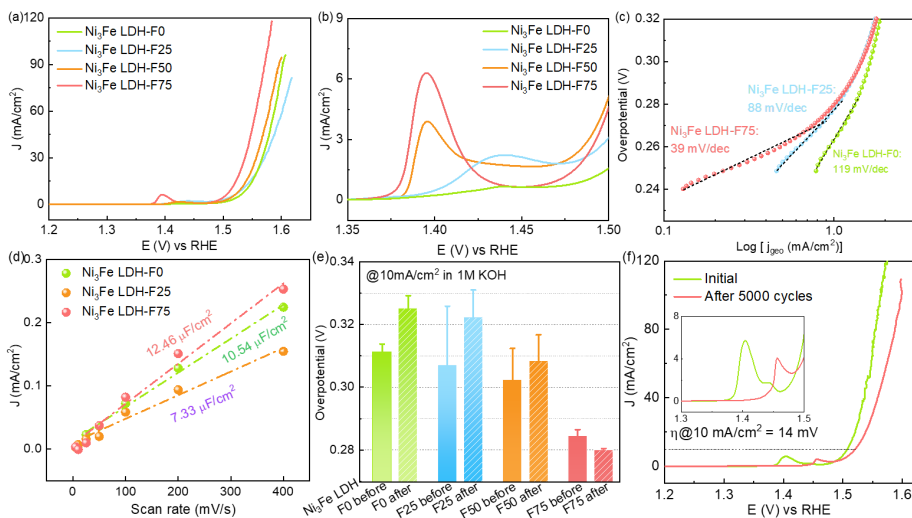
Figure 5.3 Electrochemical performance of NiFe LDH-F samples. (a) polarization curves. (b) corresponding amplified Ni oxidation peak region. (c) Tafel slope. (d) ECSA. (e) the overpotential at 10 mA/cm 2 during 1000 cycles between 1.0-1.7 V. (f) polarization curve and insert Ni oxidation peak during 5000 cycles between 1.0-1.7 V.
