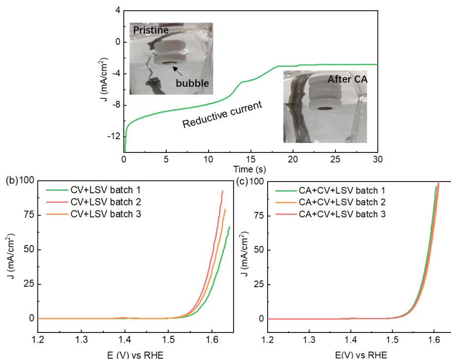
Figure 3.4 (a) the CA curve of Ni electrode at constant reductive potential -0.05 V for 30 seconds. Inserted pictures show the working electrode covered with bubbles at the beginning, and later the bubbles were consumed after the CA process. (b,c) LSV curves of independent three batches of Ni electrode without (b) and with (c) the CA process. Due to the different wettability, the three curves in (b) present some deviation, and the repeatability was improved after CA treatment in (c).
