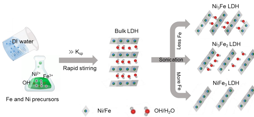
Figure 4.1 Schematic illustration of the preparation process of NiFe LDHs.
