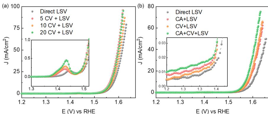
Figure 3.3 CV activation and reductive potential treatment of Ni electrode. (a) LSV curves after several cycles 0 (direct LSV), 5, 10 and 20 CV activation treatment (5, 10, 20 CV + LSV). (b) Comparison of direct LSV, LSV curves after reductive potential treatment at -0.05 V vs for 30 seconds (CA+LSV), LSV curve after 10 cycles CV activation (CV+LSV) and LSV curve after combining 10 cycles activation and reductive potential treatment at -0.05 V vs for 30 seconds (CA+CV+LSV).
