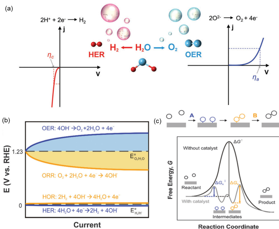
Figure 1.3 (a) polarization curves of the two half reactions of water electrolysis: OER and HER process. 3 (b) schematic diagram of the overpotentials of four half reactions. 4 (c) illustration of the reaction barrier, pathway with and without catalyst. 4
