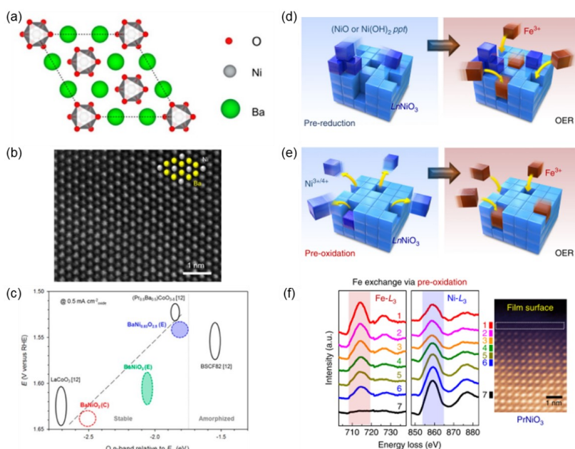
Figure 1.6 (a) Schematic of the BaNiO 3 crystal structure. (b) HADDF image of the BaNiO 3 . (c) OER activity versus the O p band center relative to E_F (eV) of the BaNiO 3 . (d, e) Schematic illustrations surface Fe exchange by (d) pre-reduction and (e) pre-oxidation reactions in LnNiO 3 (Ln = La, Pr, Nd) perovskites. (f) A layer-by-layer EELS analysis of a PrNiO 3 film subject to the Fe exchange via pre-oxidation. 43
