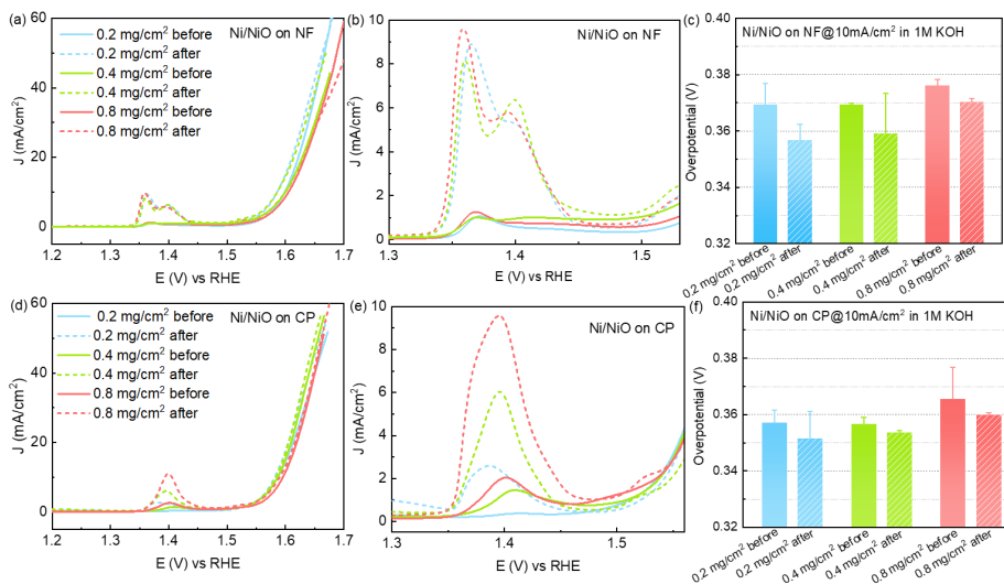
Figure 3.16 (a-c) OER polarization curves, (b) amplifying of nickel oxidation region and (c) overpotentials@10 mA/cm² of the Ni/NiO catalysts with different loadings on NF: 0.2, 0.4 and 0.8 mg/cm² before and after cycling between 1.0-1.7 V for 1000 cycles. (d) OER polarization curves, (e) amplifying of nickel oxidation region and (f) overpotentials@10 mA/cm² of the Ni/NiO catalysts with different loadings on CP: 0.2, 0.4 and 0.8 mg/cm² before and after cycling between 1.0-1.7 V for 1000 cycles.
