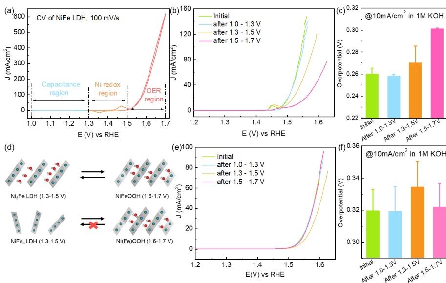
Figure 4.18 (a) CV curve of NiFe LDH between 1.0-1.7 V and the rough range for three separate regions: 1.0-1.3 V, capacitance region; 1.3-1.5 V, nickel redox region; 1.5-1.7 V, OER region. (b) LSV curves of Ni 3 Fe LDH after cycling over these ranges for 5000 cycles and (c) corresponding overpotentials. (d) illustration of the phase transition process of NiFe LDHs during cycling process. (e) LSV curves of NiFe 3 LDH after cycling over these ranges for 5000 cycles and (f) corresponding overpotentials.
