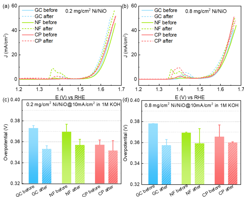
Figure 3.21 (a-b) OER polarization curves, and (c,d) overpotentials@10 mA/cm 2 of Ni/NiO catalysts before and after cycling between 1.0-1.7 V for 1000 cycles in 1M KOH. Among them, (a,c) the loading of Ni/NiO is 0.2 mg/cm 2 while (b,d) 0.8 mg/cm 2 .
