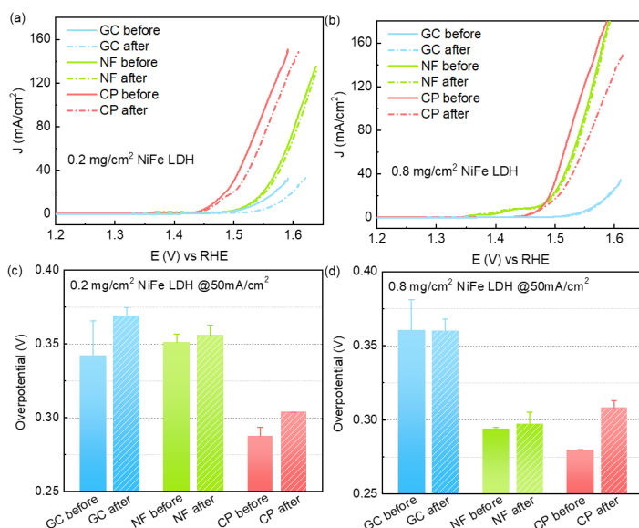
Figure 3.22 (a-b) OER polarization curves, and (c,d) overpotentials@50 mA/cm 2 of the NiFe LDH catalysts on various substrates before and after keeping at 1.6 V for 20 h in 1 M KOH solution. Among them, (a,c) the loading is 0.2 mg/cm 2 while (b,d) 0.8 mg/cm 2 .
