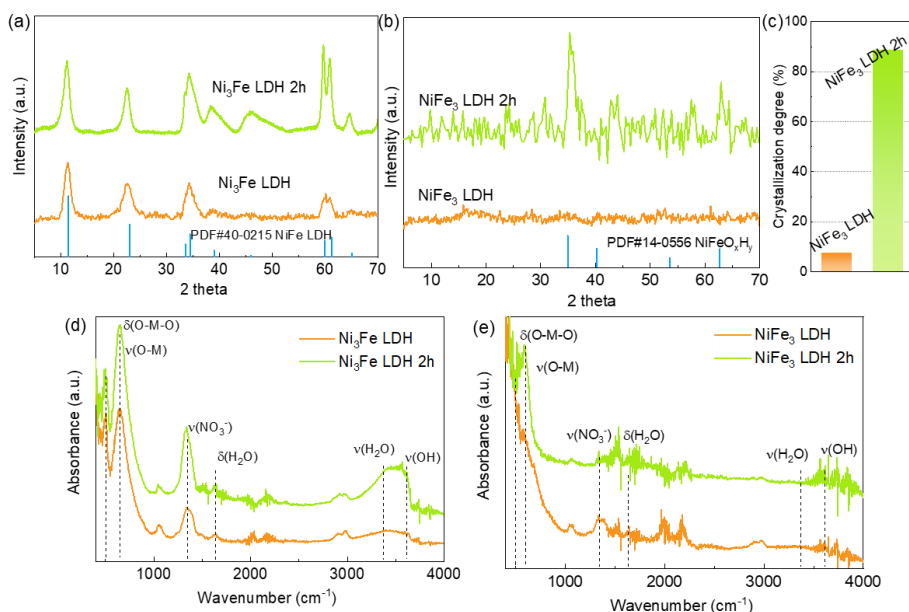
Figure 5.12 (a-c) XRD patterns and (d-e) IR spectra of NiFe LDH before and after hydrothermal treatment. (a,d) Ni 3 Fe LDH. (b,c,e) NiFe 3 LDH.
