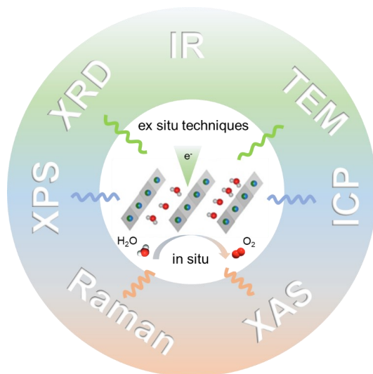
Figure 2.2 Summary of the characterization techniques for NiFe LDH electrocatalysts.
