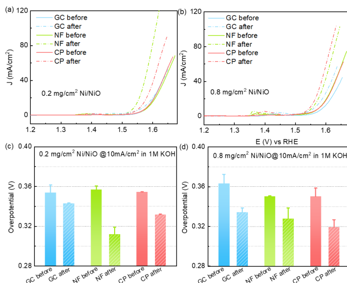
Figure 3.23 (a-b) OER polarization curves, and (c,d) overpotentials@10 mA/cm 2 of the Ni/NiO catalysts on various substrates before and after keeping at 1.6 V for 20 h in 1 M KOH solution. Among them, (a,c) the loading is 0.2 mg/cm 2 while (b,d) 0.8 mg/cm 2 .
