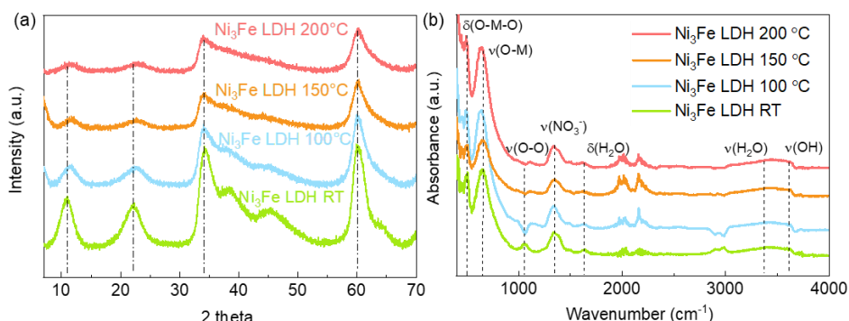
Figure 5.9 (a) XRD pattern and (b) IR spectra of Ni 3 Fe LDH after heat treatment at various temperatures, 100, 150 and 200 °C for 2 hours.
