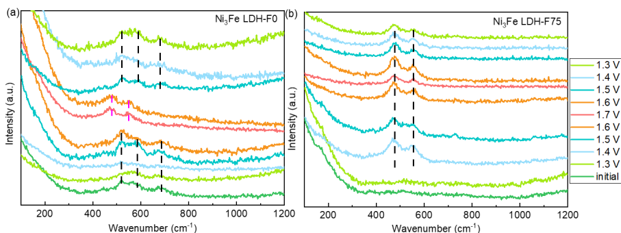
Figure 5.5 In situ Raman spectra of (a) \text{Ni}_3\text{Fe} LDH-F0 and (b) \text{Ni}_3\text{Fe} LDH-F75 catalysts.
