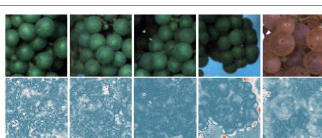
FIGURE 8 | Results for pixel-wise anomaly detection obtained by an FPL-VAE for healthy patches. The original images are displayed in the upper row. A corresponding heatmap of loss values is displayed in the lower row, where a red color represents anomalies and dark blue indicates non-anomalies.
