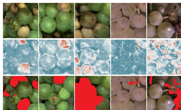
FIGURE 7 | Results for pixel-wise anomaly detection obtained by an FPL-VAE for damaged patches. The original images are displayed in the upper row. A corresponding heatmap of loss values is displayed in the middle, red color represents anomalies, and dark blue indicates non-anomalies. The darker the color, the more certain the network is, that a berry is damaged or healthy. In the third row, the red color highlights the manual annotations of anomalous berry regions.
