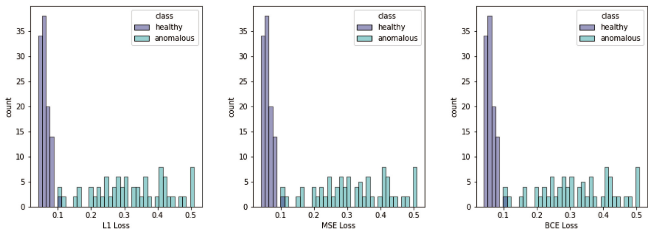
FIGURE 6 | Histograms of different losses, namely \ell_1 , MSE, and BCE. Losses are computed for all test patches containing healthy and anomalous berries.
