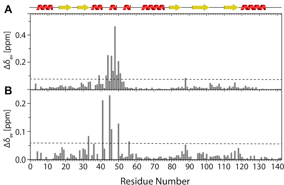
Fig. 3 Backbone amide chemical shift perturbations of PpSB1-LOV due to I48T mutation in the dark-(A) and light state (B). Chemical shift perturbation \Delta\delta_{av} relative to the corresponding dark- and light-state chemical shifts of wild-type PpSB1-LOV. Significant chemical shift changes ( \Delta\delta_{av} ) arising from the I48T mutation are mostly localized around the mutation site (residues 39–51). The significance level
