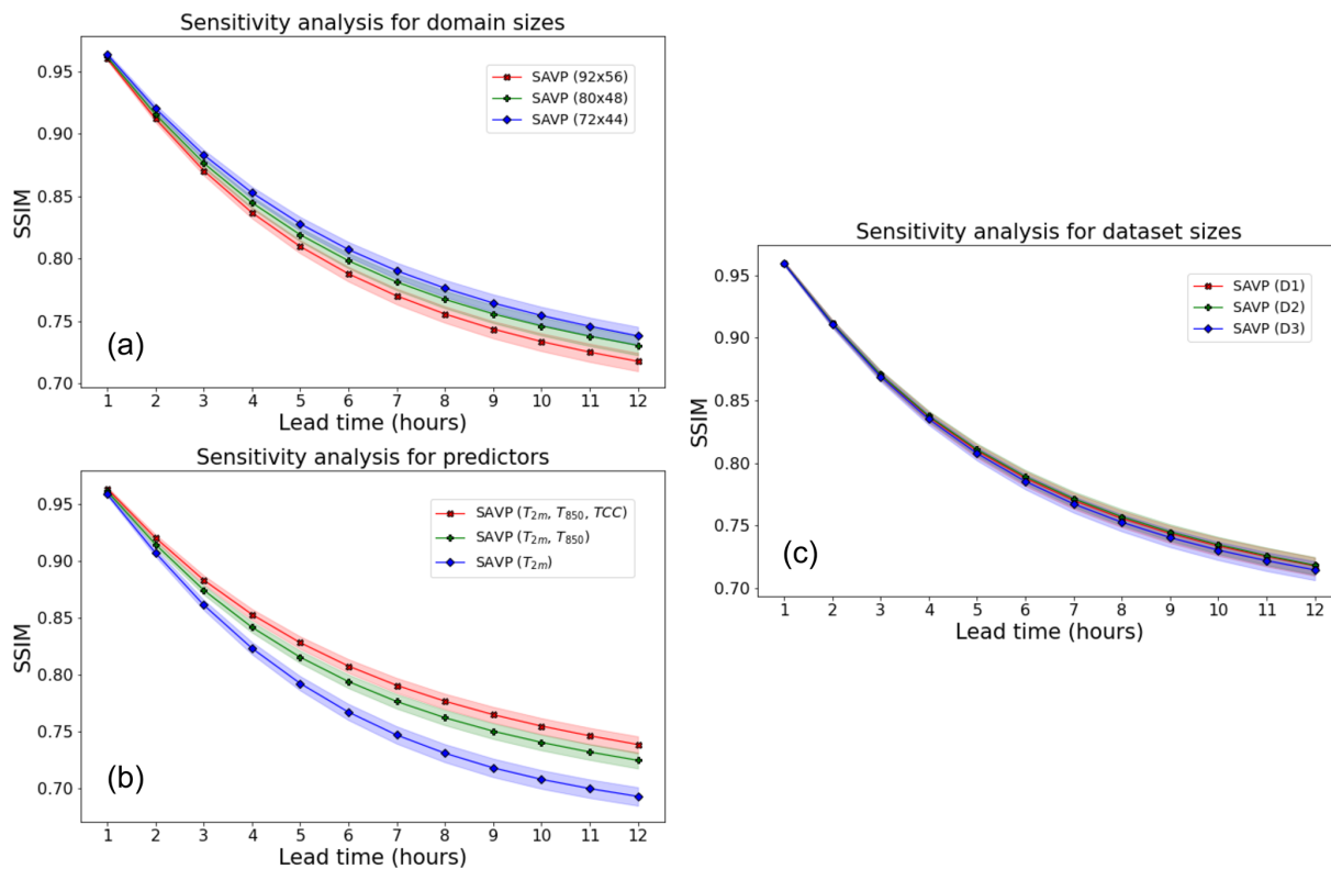
Figure C4. Like Fig. C3 but for SSIM.
