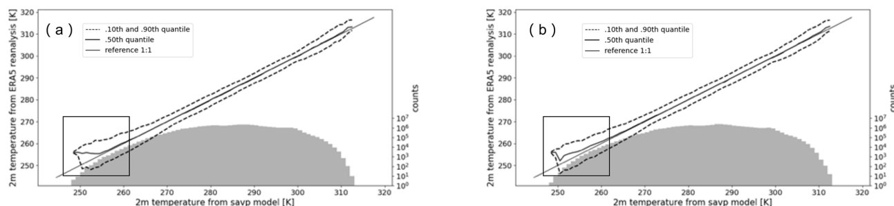
Figure 9. Conditional quantile plots in terms of the calibration-refinement factorization for 2 m temperature forecasts with a lead time of 12 h of the SAVP model with (a) \lambda_1 = 10\,000 and (b) \lambda_1 = 15 .
