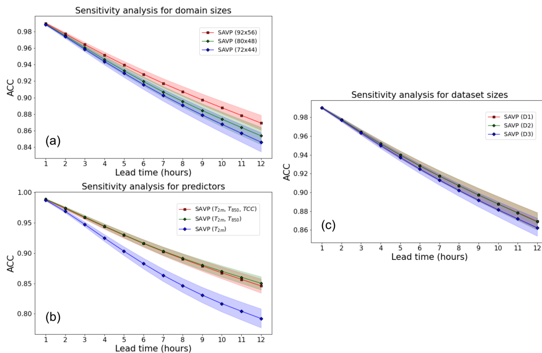
Figure C3. Averaged ACC over the forecast period for 2 m temperature with the SAVP model for different sensitivity experiments using (a) different domain sizes (red – 92 \times 56 ; green – 80 \times 48 ; blue – 72 \times 44 ), (b) different predictors (red – T_{2m} , T_{850} hPa, and TCC; green – T_{2m} , T_{850} hPa; blue – T_{2m} ), and (c) different sizes of the training dataset (red – 11 years; green – 10 years; blue – 8 years). The inter-decile confidence range (colour shaded) is estimated via block bootstrapping.
