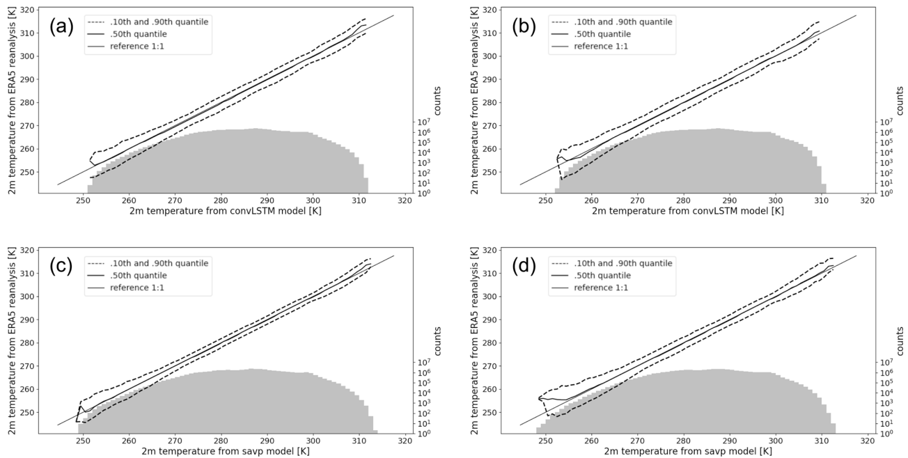
Figure 7. Conditional quantile plots in terms of the calibration-refinement factorization for 2 m temperature forecasts with a lead time of 6 h (a, c) and 12 h (b, d). Panels (a, b) show the factorization of ConvLSTM forecasts, while (c, d) correspond to the SAVP model. The solid straight line denotes the 1 : 1 reference line of a hypothetical perfect model. The dashed lines represent the 10th and 90th quantiles, and the bold solid line represents the median of the ground truth data conditioned on the forecasts, respectively. The marginal distribution of the model forecasts is presented as log histogram (right axis, light grey bars).
