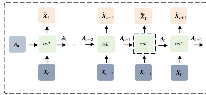
(a) LSTM Future Predictor Model
