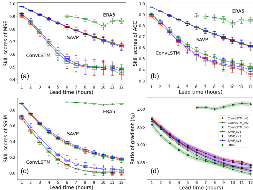
Figure 5. Averaged skill scores of (a) MSE, (b) ACC, and (c) SSIM across lead time ( x axis) for the SAVP and the ConvLSTM models as well as ERA5 short-range forecasts. Both video prediction models are trained with the three cross-validation datasets (with CV 1–3 in D1) displayed in Fig. 2. The testing period of the ERA5 short-range forecasts covers the year 2019, which corresponds to CV 2. The persistence serves as the reference forecast. Sampling uncertainty estimated via block bootstrapping is illustrated by box-and-whisker plot showing the inter-quartile and inter-decile ranges of the skill score values. Panel (d) shows the ratio of the spatially averaged 2 m temperature gradient for the same video prediction models and ERA5 short-range forecasts. The persistence forecasts (not shown) attain a constant value of r_G = 1 since local spatial variability is retained.
