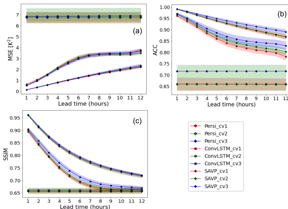
Figure C2. Averaged (a) MSE, (b) ACC, and (c) SSIM across lead time ( x axis) for the SAVP, the ConvLSTM, and the persistence forecasts from Experiment 1 in Table A2. Like in Fig. 2, sampling uncertainty is estimated via block bootstrapping. However, the inter-decile confidence range is now colour shaded for the three cross-validation datasets using different models.
