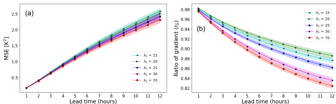
Figure 8. Performance of the SAVP model in terms of (a) MSE and (b) the gradient ratio r_G with variations in the scaling factor for the L1 loss \lambda_1 . Note that the results for \lambda_1 = 70 only differ marginally from using \lambda_1 = 10\,000 .
