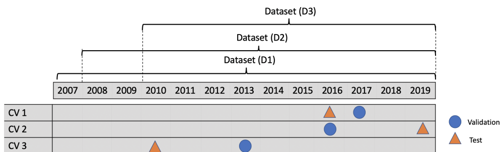
Figure 2. The three cross-validation datasets (CV 1, CV 2, and CV 3) consist of different training, validation, and testing samples from the 13 years ERA5 reanalysis data between 2007 and 2019. Each row represents one data partition. The three datasets (D1, D2, and D3) consist of samples from 2007 to 2019, from 2008 to 2019, and from 2010 to 2019, respectively.
