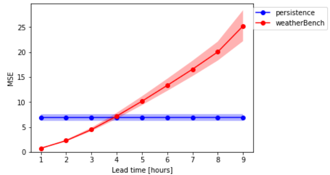
Figure C1. MSE over 9 h forecast for 2 m temperature with inter-decile bootstrap confidence intervals (shading area) using Weather-Bench convolutional neural network and persistence forecasting.
