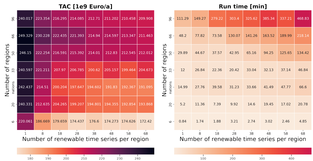
Figure 9. TAC obtained and the associated run time for each combination of parameters considered in this study.
