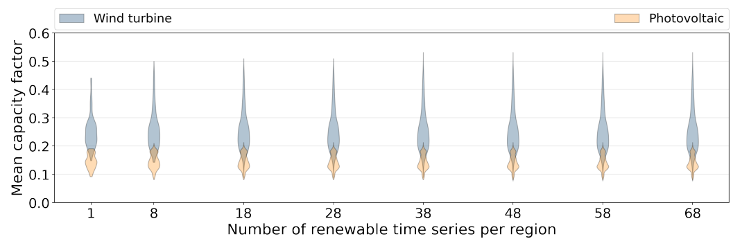
Figure 7. Distribution of installable capacities in all 96 e-highway regions, for different number of VRES time series per region.
