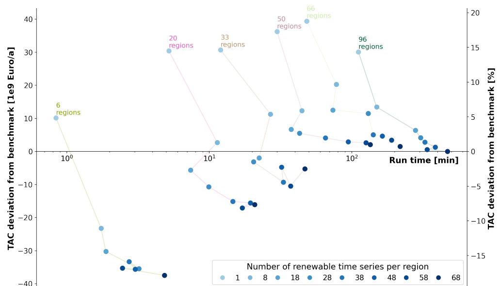
Figure 12. TAC deviation from the benchmark (represented on the y-axis in EUR billion/annum on the left and in % on the right) versus the run time (represented on a logarithmic scale on the x-axis) for each parameter setting. Each dot represents a particular parameter setting. The darker the shade of blue, the greater the number of VRES time series considered, with the lines connecting the dots representing a particular number of regions.
