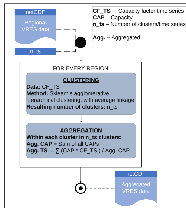
Figure 4. Flowchart of technological aggregation algorithm.
