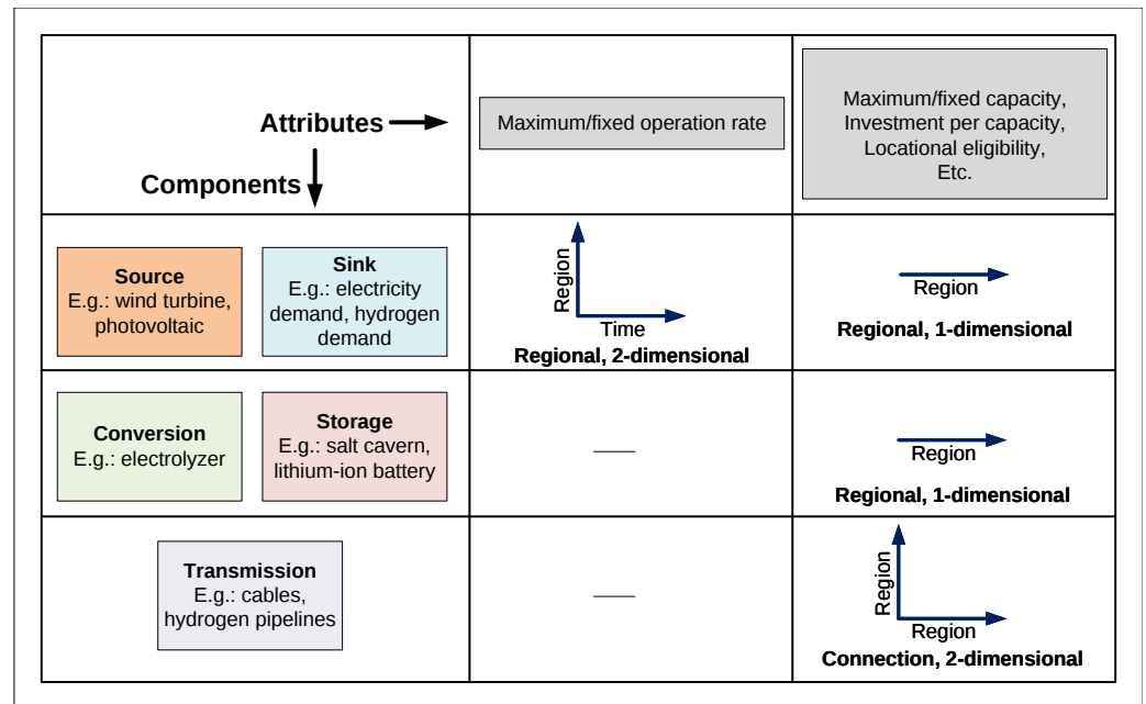
Figure 2. The general data structure of an ESOM.
