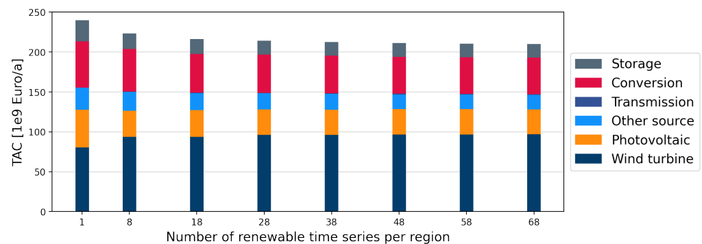
Figure 11. TAC obtained for different technologies in the case of 96 regions, when different numbers of aggregated VRES time series per region are considered.
