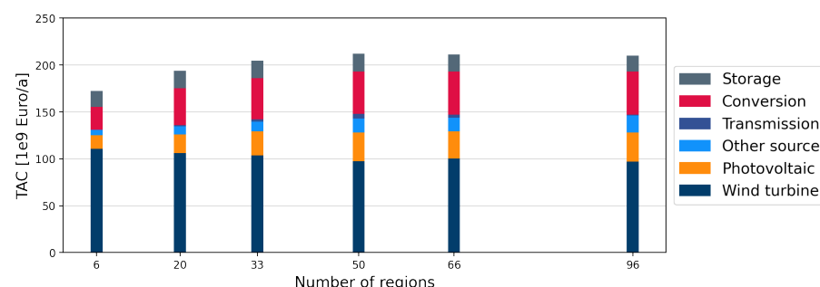
Figure 10. TAC obtained for different technologies in the case of differing numbers of aggregated regions, while considering 68 VRES time series per region.
