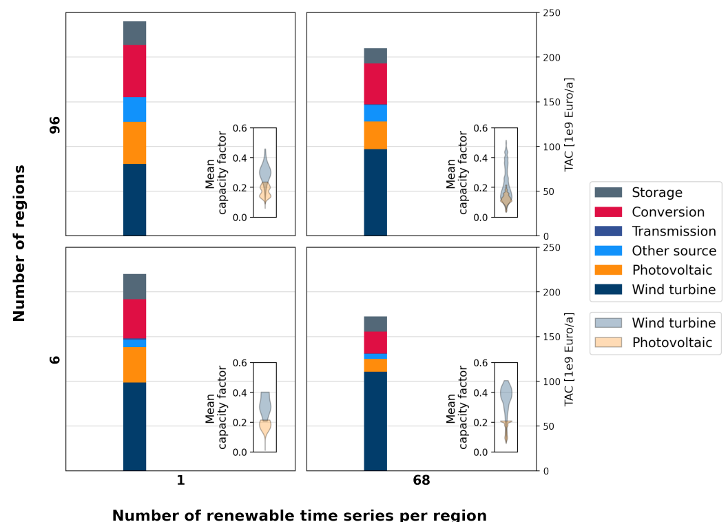
Figure 8. The results of optimization for the extreme parameter combinations (i.e., 6 and 96 regions and 1 and 68 VRES time series per region). For each of these combinations, TAC for different technologies is seen on the left, and the distribution of installed VRES capacities on the right.
