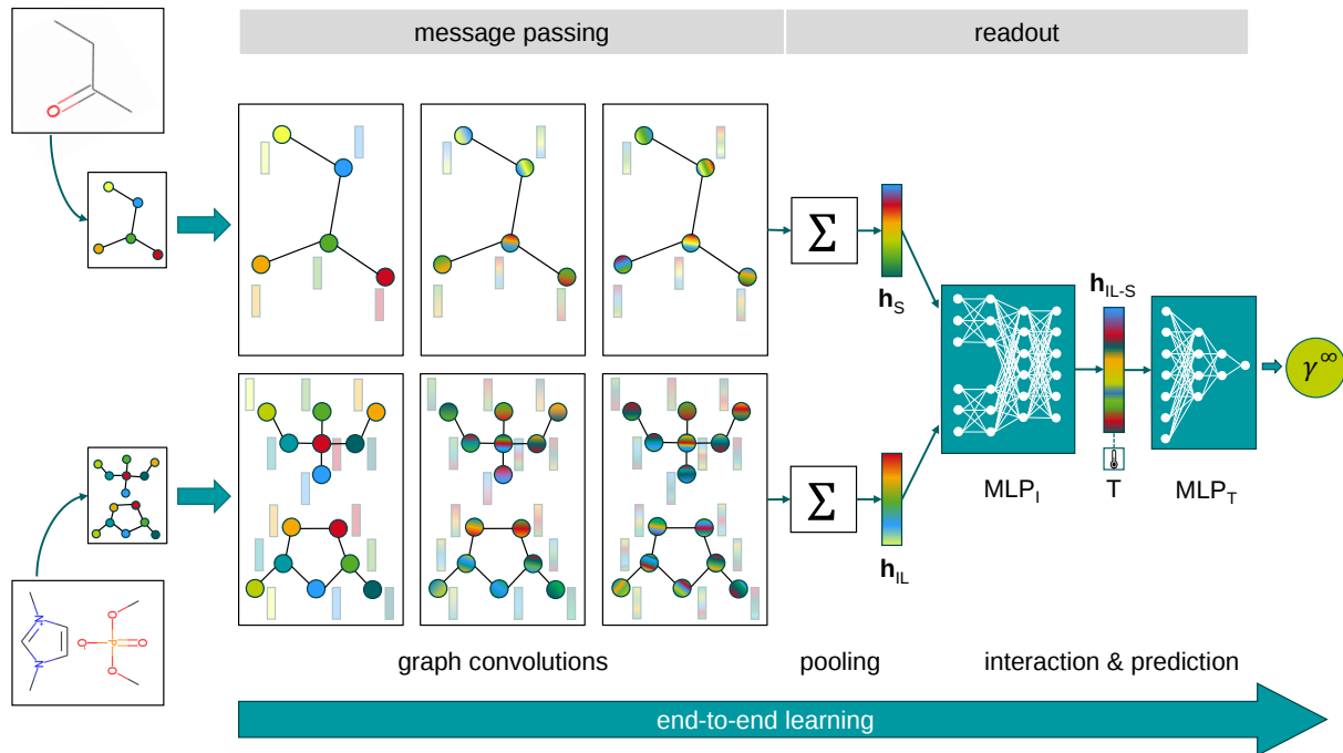
Fig. 1. Graph neural network model for prediction of the temperature-dependent infinite dilution activity coefficient of solutes in ionic liquids.
