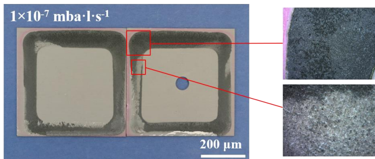
Fig. 4-15. Ink penetration test for sandwich sample (pre-oxidized Aluchrom plates sealed with HNC30); overview on the left and magnification on the right
