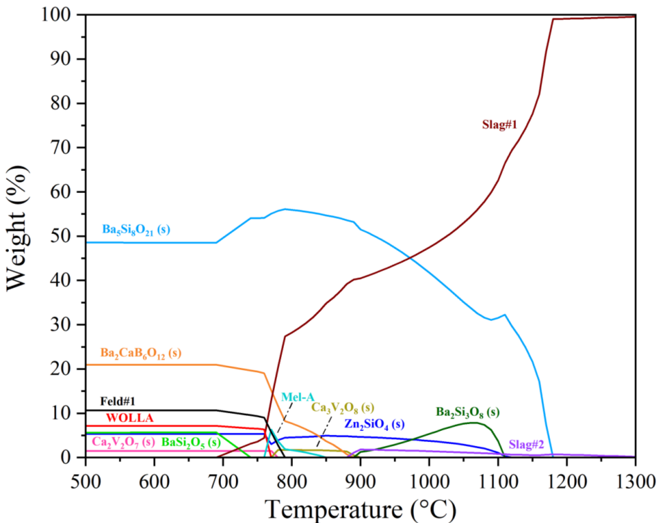
Fig. 4-5. Stable phases versus temperature by FactSage simulation for glass H
