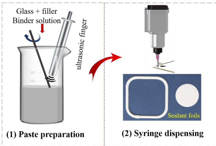
Fig. 3-3. Schematic diagram of robot syringe dispensing process, (1) paste preparation, (2) syringe dispensing and sealant foils
