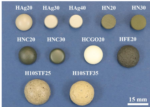
Fig. 4-6. Composite pellets sintered at 850 °C for chemical compatibility investigation
