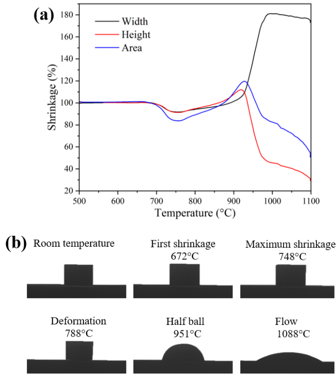
Fig. 4-36. HSM analysis (TOMMIplus) for HBS30 glass composite sealant on Crofer22APU substrate recorded at 5 °C/min, (a) shrinkage curves, (b) Shadow images of the sample at the fixed temperatures
