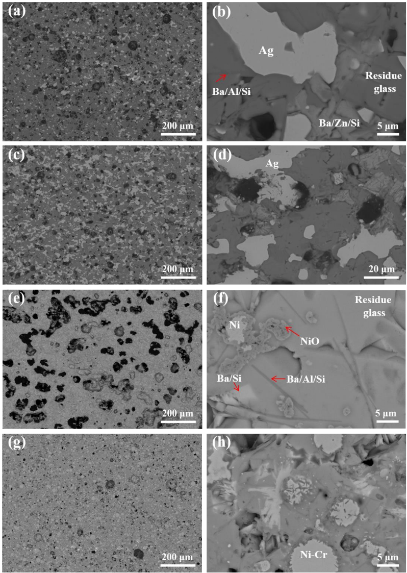
Fig. 4-13. SEM-EDS analyses for annealing composites (a, b) HAg20A, (c, d) HAg40A, (e, f) HN30A, (g, h) HNC30A; overview on the left and magnification on the right
