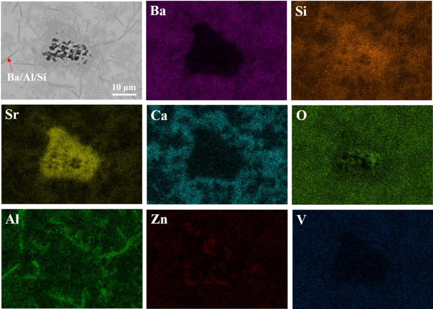
Fig. 4-52. SEM-EDS maps of the sealant HS2S20 from STF25/HS2S20/Aluchrom joint
