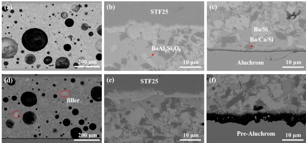
Fig. 4-39. Joints STF25/HBS30/Aluchrom (a-c) and STF25/HBS30/pre-oxidized Aluchrom (d-f); both joints jointed at 960 ^{\circ}\text{C} for 5 min.
