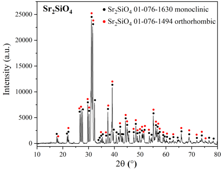
Fig. 4-45. XRD pattern of the synthesized \text{Sr}_2\text{SiO}_4 filler (1350 °C for 30 h)
