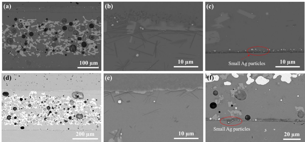
Fig. 4-32. SEM images of cross-section of STF25/HAg40/Aluchrom, joining at: (a-c) 935 °C 5 min, (d-f) 900 °C 30 min
