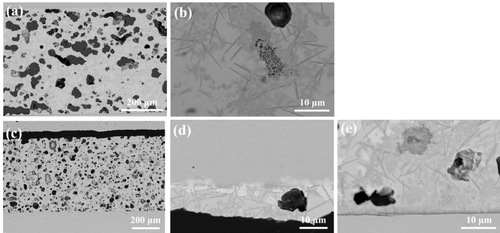
Fig. 4-53. SEM images of the cross-sections of joints STF25/HS2S20/Aluchrom, (a, b) joined at 920 °C for 15 min with a 100 g dead load, (c-e) joined at 850 °C for 10 h with a 150 g dead load
