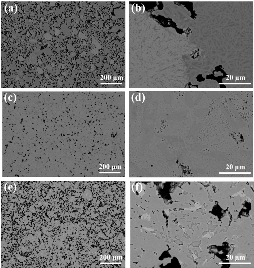
Fig. 4-57. SEM-EDS analyses for the annealed dilatometer samples (a, b) BS6A, (c, d) BS15A, (e, f) BS25A; overview on the left and magnification on the right
