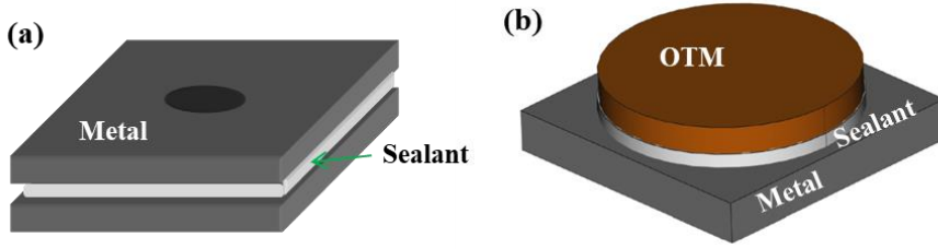
Fig. 3-5. Schematic illustrations of joining geometries: (a) sealant sealing metal plates for gas-tightness testing, (b) sealant assembled with OTM and metallic support
