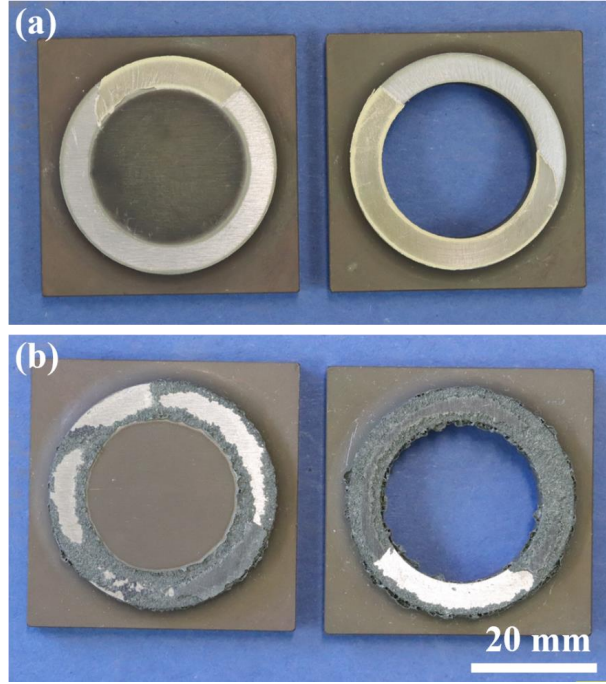
Fig. 4-19. Photograph of fracture surfaces after torsion tests at room temperature for HAG40 (a) and HNC30 (b) glass composite sealants
