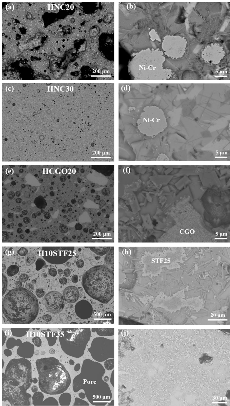
Fig. 4-8. SEM micrographs of composites as joined: (a, b) HNC20, (c, d) HNC30, (e, f) HCGO20, (g, h) H10STF25, (i, j) H10STF35; overview on the left and magnification on the right
