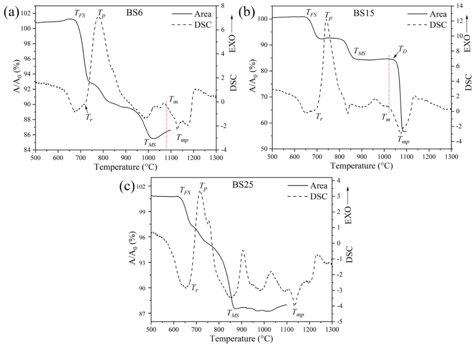
Fig. 4-61. HSM and DTA curves obtained from the powdered BS glasses (a) BS6, (b) BS15, and (c) BS25.
