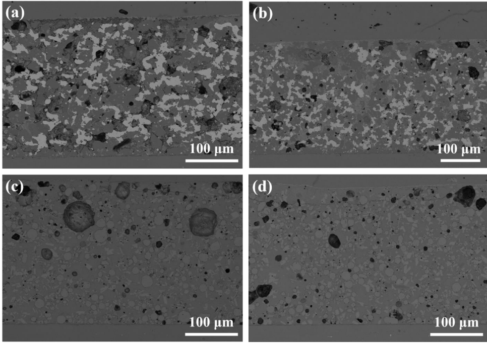
Fig. 4-25. SEM images of the assembled joints after different cycling times, (a) STF25/HAg40/Aluchrom, 2 times cycling, (b) STF25/HAg40/Aluchrom, 10 times cycling, (c) STF25/HNC30/Aluchrom, 2 times cycling, (d) STF25/HNC30/Aluchrom, 10 times cycling.
