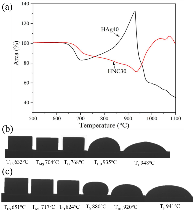
Fig. 4-27. HSM analysis (TOMMIplus) for HAg40 and HNC30 glass composite sealant on Crofer22APU substrate recorded at 5 °C/min, (a) area deformation versus temperature curves, (b) shadow images of HAg40 at the fixed temperatures, (c) shadow images of HNC30 at the fixed temperatures
