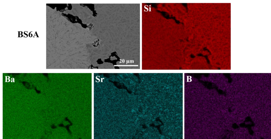
Fig. 4-58. EDS maps of the annealed sample BS6A after sintering at 900 °C for 1 h and thermal treatment at 850 °C for 50 h
