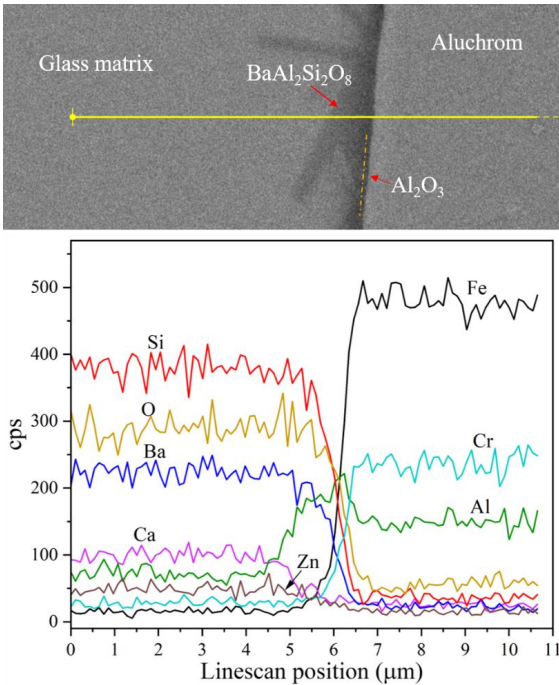
Fig. 4-31. Line scan through the interface between sealant HNC30 and Aluchrom joined at 880 °C 15 min + 920 °C 5 min
