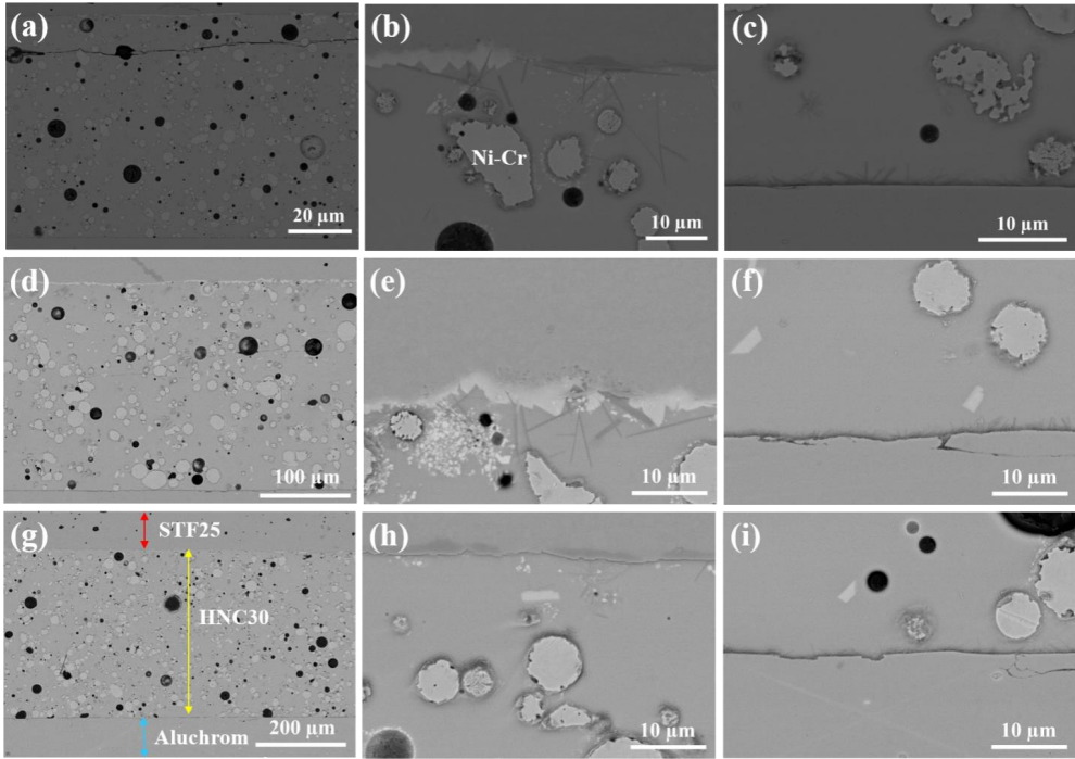
Fig. 4-29. SEM images of cross-section of STF25/HNC30/Aluchrom, (a-c) 880 °C 15 min + 920 °C 5 min, (d-f) 900 °C 15 min, (g-i) 880 °C 30 min
