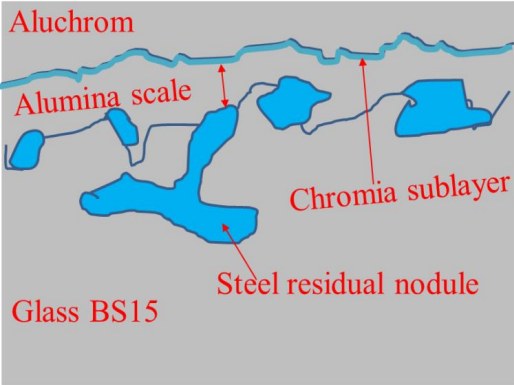
Fig. 4-67. Schematic diagram of the interface reaction between BS15 glass sealant and Alchrom joined at 1075 °C for 5 min
