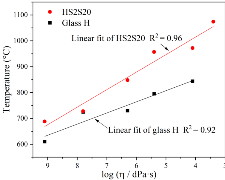
Fig. 4-50. Viscosity-temperature curves of glass H and composite sealant HS2S20
