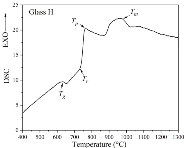
Fig. 4-1. (a) DSC thermograms of glass H at a heating rate of 15 °C/min
