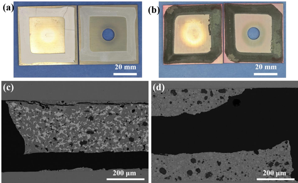
Fig. 4-23. Gas tightness joints Aluchrom/sealant/Aluchrom 50 times cycling thermal treatment, (a) the joint Aluchrom/HAg40/Aluchrom not adhesion anymore after 50 times cycling, (b) after ink penetration test, the chopped Aluchrom/HNC30/Aluchrom joint, some part red ink penetrated into the joint, (c) SEM image of the 50 times cycling cross section of joint Aluchrom/HAg40/Aluchrom, (d) cross section microstructure of the chopped joint Aluchrom/HNC30/Aluchrom after 50 times cycling.
