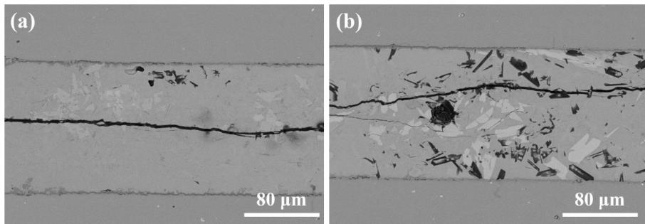
Fig. 4-64. SEM images of the gas-tight joint Alchrom/BS15/Aluchrom joining at 1075 °C for 5 min, (a) and (b) show inhomogeneous structures.
