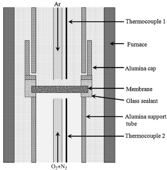
Fig. 2-10. Schematic diagram of the oxygen permeation flux measurements device [88]
