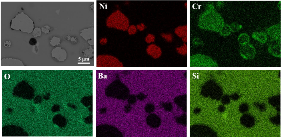
Fig. 4-30. SEM-EDS maps of STF25/HNC30/Aluchrom, joined at 880 °C 15 min + 920 °C 5 min, for investigating the condition of filler Ni-Cr
