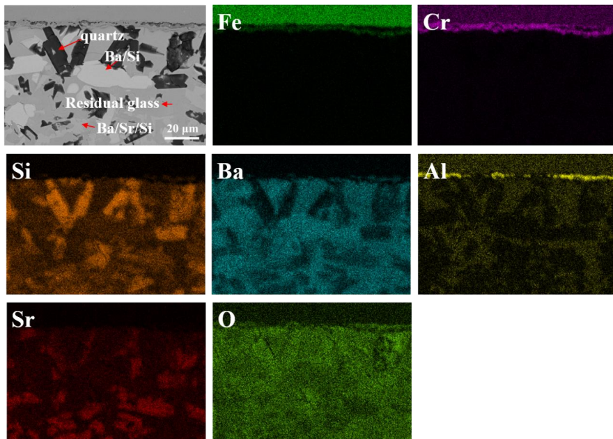
Fig. 4- 65. SEM-EDS maps of the gas-tight joint Alchrom/BS15/Aluchrom joining at 1075 °C for 5 min for analyzing crystalline phases from BS15 sealant and interaction layer of BS15 and Aluchrom.
