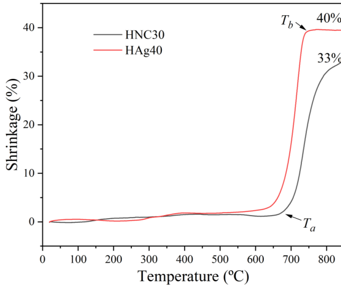
Fig. 4-14. Sinking dilatometer of HAg40 and HNC30
