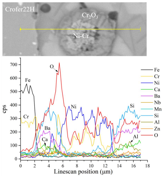
Fig. 4-21. Line scan through the filler Ni-Cr at the sample Crofer22H/HNC30
