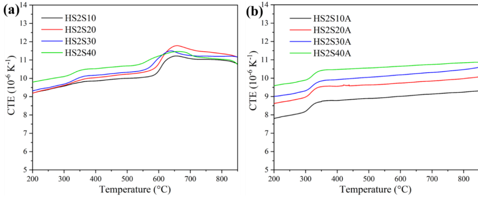
Fig. 4-46. CTE curves for composite samples sintered (a) and annealed (b)
