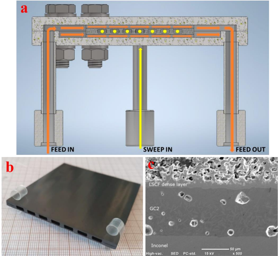
Fig. 2-4. (a) Section of a membrane module prototype, LSCF membrane component assembling in the metallic case with the aid of a Ba-based borosilicate glass (GC2) sealant; (b) final membrane component with dimensions of 60×60 mm; (c) SEM cross section of joint LSCF/GC2 sealant/Inconel [46]
