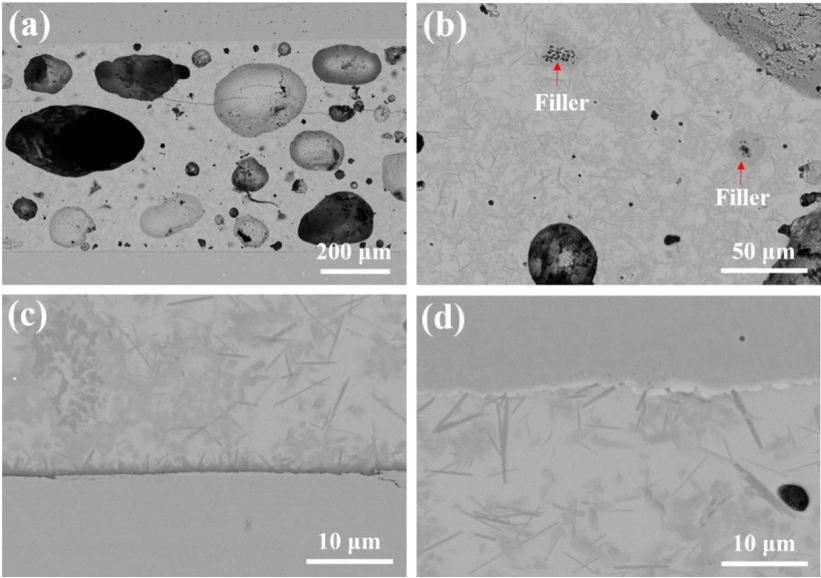
Fig. 4-51. SEM images of the cross-section of joint STF25/HS2S20/Aluchrom joining at 960 °C for 10 min with a 60 g dead load
