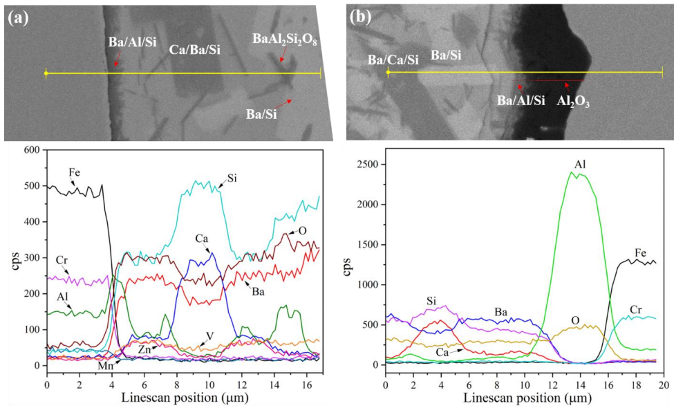
Fig. 4-43. Line scans through the interface between sealant HBS30 and Aluchrom (a), HBS30 and pre-oxidized Aluchrom (b), the samples joined at 960 °C for 5 min
