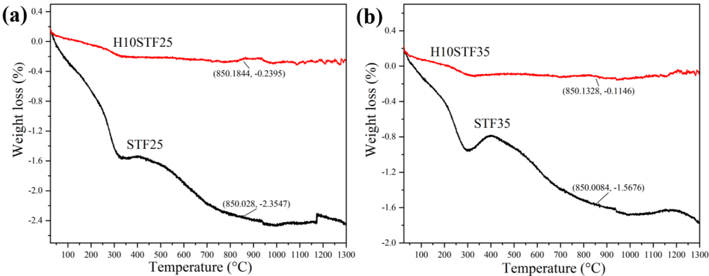
Fig. 4-10. Weight loss curves of STF fillers and mixed with glass H
