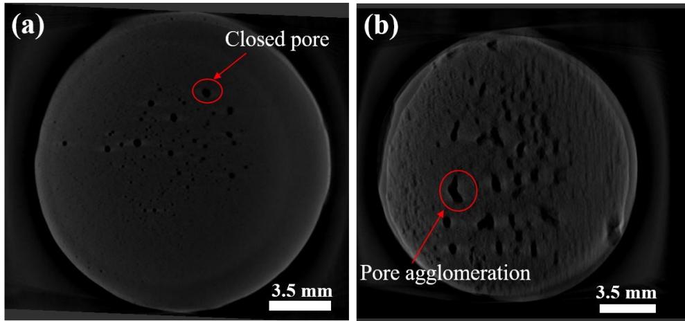
Fig. 4-28. CT images of inner scanning from longitudinal section for inspecting sealants joining behaviors without destruction, (a) STF25/HNC30/Aluchrom joining at 880 °C, 15 min + 920 °C, 5 min, (b) STF25/HAg40/Aluchrom joining at 935 °C, 5 min
