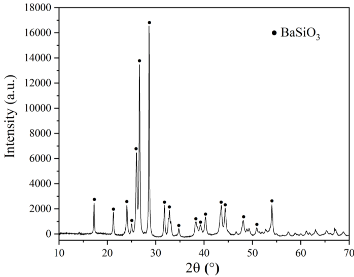
Fig. 4-33. XRD pattern of the BaSiO 3 filler
