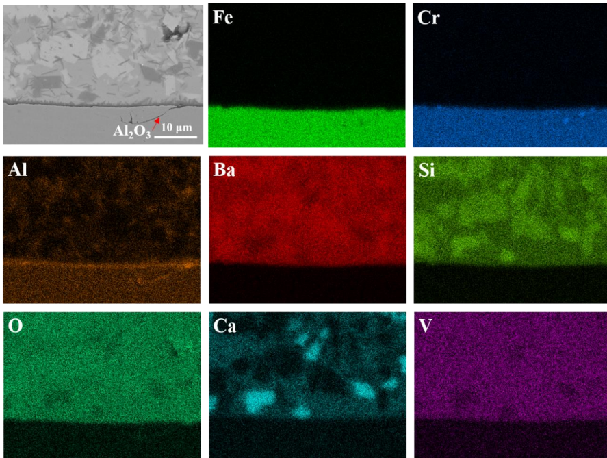
Fig. 4-42. SEM-EDS maps of the joint STF25/HBS30/Aluchrom ( 960\ ^\circ\text{C} , 5 min) for analyzing diffusion layer of Aluchrom and HBS30
