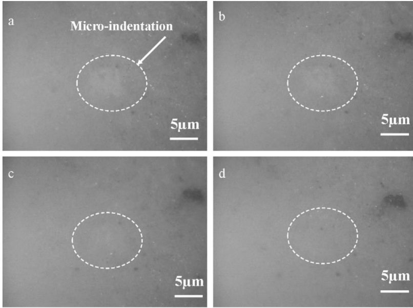
Fig. 2-13. In situ optical images of the calcium borate glass after crystallization at 850 °C in air for one week: in situ observation at (a) room temperature, (b) 700 °C, (c) 800 °C, and (d) 840 °C [102]
