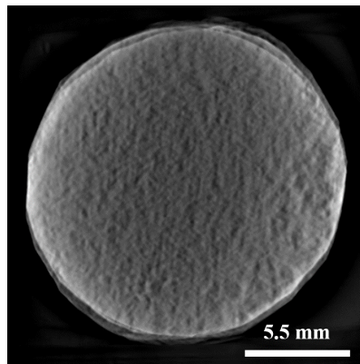
Fig. 4-38. CT images of STF25/HBS30/Aluchrom after joining at 920 °C for 15 min scanning from longitudinal section
