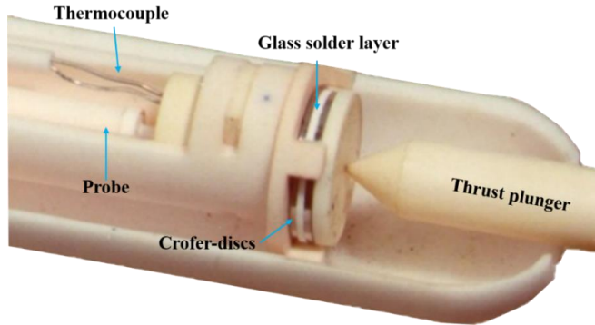
Fig. 3-2. Probe head of the sinking dilatometer
