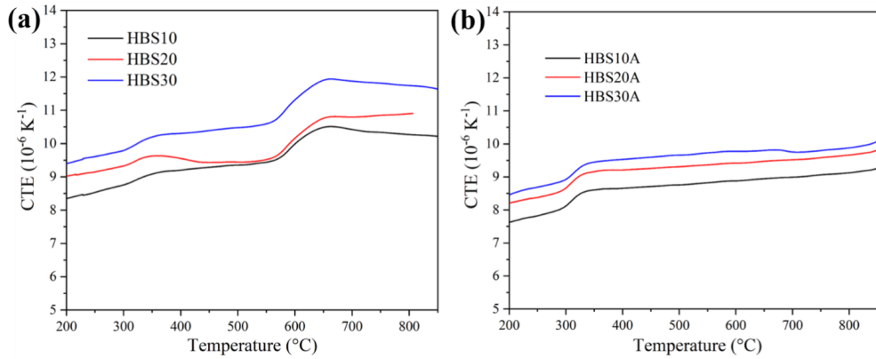
Fig. 4-34. Dilatometer curves of glass H reinforced by \text{BaSiO}_3 with different amount, (a) composite samples as sintered after heat treatment at 850^{\circ}\text{C} for 10 h, (b) additionally treated at 800^{\circ}\text{C} for 1000 h
