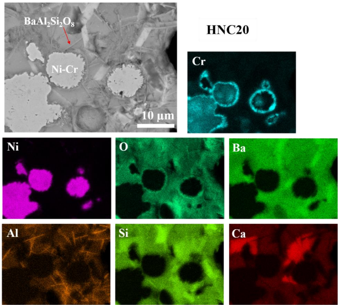
Fig. 4-9. SEM-EDS maps of the HNC20 sample
