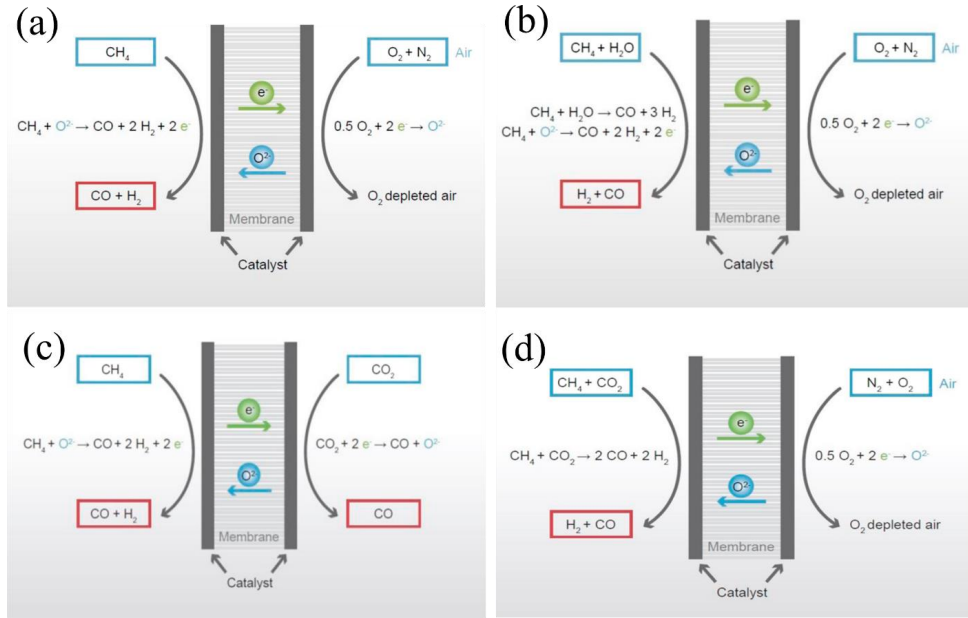
Fig. 2-2. Schematics of the working principles in four oxygen transport membrane reactors: (a) partial oxidation of methane, (b) autothermal reforming of methane, (c) and (d) two possible membrane configurations for the dry reforming of methane [6].
