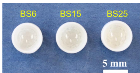
Fig. 4-55. DSC crucibles of BS glasses (cooling rate 15 °C/min)
