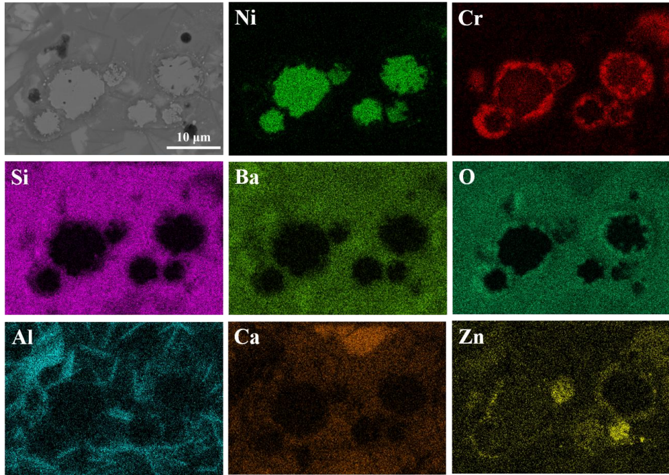
Fig. 4-24. EDS maps of the joint Aluchrom/HNC30/Aluchrom after 50 times thermal cycling
