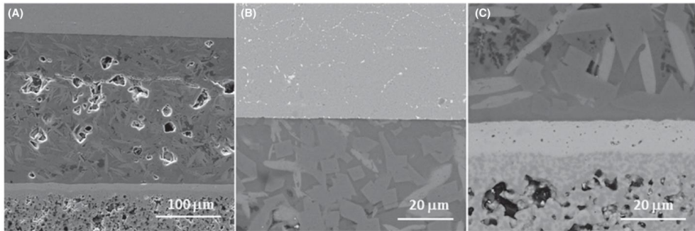
Fig. 2-11. Joint of Crofer 22 H/glass-ceramic/8YSZ sealed by 10B(Sr) composition sealant at 850 °C for 10 h and thermally cycled (50 cycles). (A) General view. (B) Interface steel/sealant. (C) Interface sealant/8YSZ [92]
