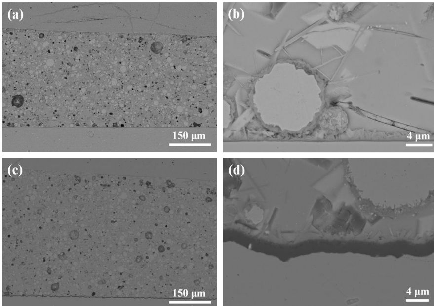
Fig. 4-17. Joints STF25/HNC30/Aluchrom (a-b) and STF25/HNC30/pre-Aluchrom (c-d); both joints sealed at 850 °C with a 400 g dead load
