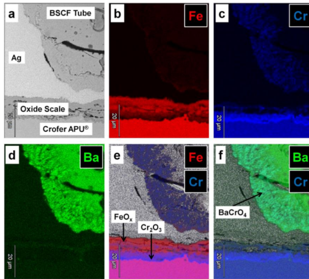
Fig. 2-5. SEM/EDX maps of BSCF/Ag/Crofer 22 APU assembly. (a) overview image; (b) Fe distribution; (c) Cr distribution; (d) Ba distribution; (e) overlapped EDX maps of Fe and Cr; (f) overlapped EDX maps of Ba and Cr [62]
