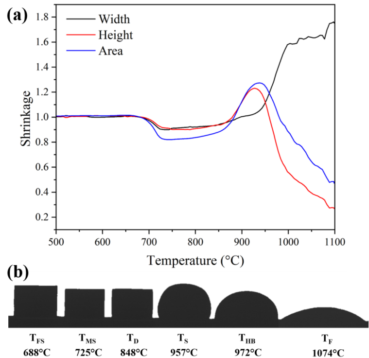
Fig. 4-49. HSM analysis (TOMMIplus) for HS2S20 glass composite sealant on Crofer 22 APU substrate recorded at 5 °C/min, (a) shrinkage curves, (b) Shadow images of the sample at the fixed temperature
