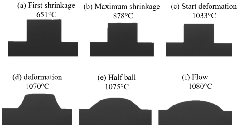
Fig. 4-62. Shadow images of BS15 glass pellet on Crofer22APU substrate from HSM
