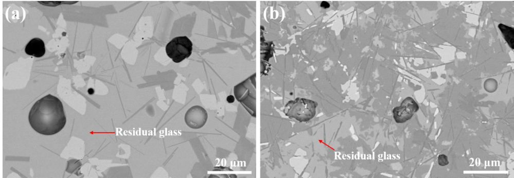
Fig. 4-3. SEM micrographs of dilatometer samples, (a) glass H sintered at 850 ^{\circ}\text{C} for 10 h, (b) the annealed glass H sample sintered at 850 ^{\circ}\text{C} for 10 h then aged at 800 ^{\circ}\text{C} for 1000 h.
