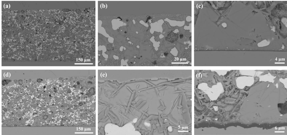
Fig. 4-16. Joints STF25/HAg40/Aluchrom (a-c) and STF25/HAg40/pre-Aluchrom (d-e); both joints sealed at 850 °C with a 400 g dead load
