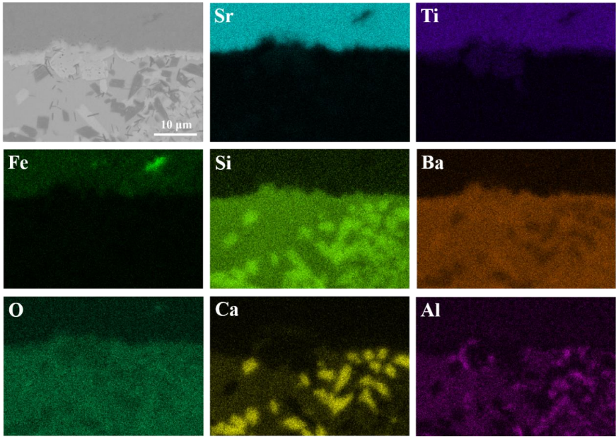
Fig. 4-41. SEM-EDS Trumaps of the joint STF25/HBS30/Aluchrom (960 °C, 5 min) for analyzing diffusion layer of STF25 and HBS30
