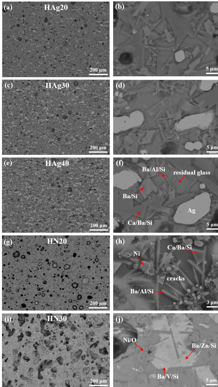
Fig. 4-7. SEM micrographs of composites as joined: (a, b) HAg20, (c, d) HAg30, (e, f) HAg40, (g, h) HN20, (I, j) HN30; overview on the left and magnification on the right
