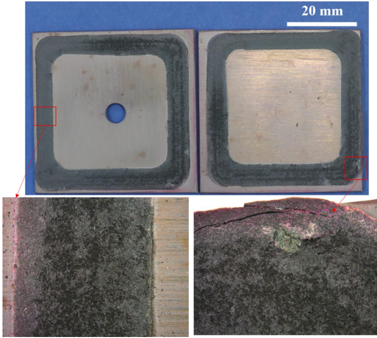
Fig. 4-26. After ink penetration test, the chopped gas-tight joint Aluchrom/HNC30/Aluchrom joint sealed at 850 °C for 10 h and later heated at 800 °C for 500 h
