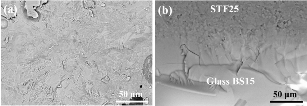
Fig. 4-69. SEM images of BS15/STF25 part from the assembled joint shown in Fig. 4-68 (c), (a) top view on glass sealant layer, (b) side view after breaking of the BS15/STF25 piece
