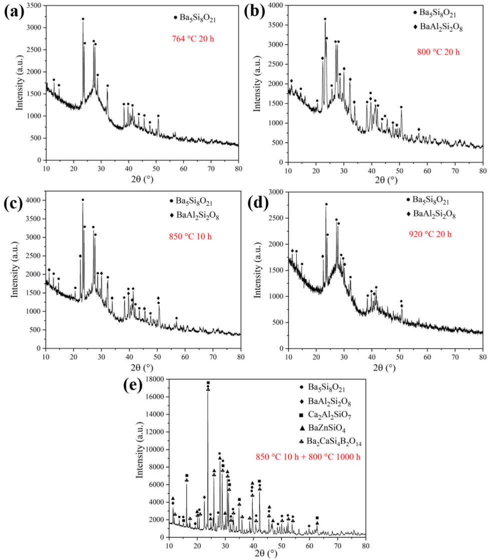
Fig. 4-4. Glass H after different heat-treatments for crystallization analysis, (a) XRD pattern of glass H after heating at 764 ^{\circ}\text{C} for 20 hours, (b) XRD pattern of glass H after heating at 800 ^{\circ}\text{C} for 20 hours, (c) XRD pattern of glass H after heating at 850 ^{\circ}\text{C} for 10 hours, (d) XRD pattern of glass H after heating at 920 ^{\circ}\text{C} for 20 hours, (e) XRD pattern of glass H after heat-treatment at 850 ^{\circ}\text{C} for 10 hours followed by 800 ^{\circ}\text{C} for 1000 hours, with same heating and cooling rate of 2 ^{\circ}\text{C}/\text{min} .
