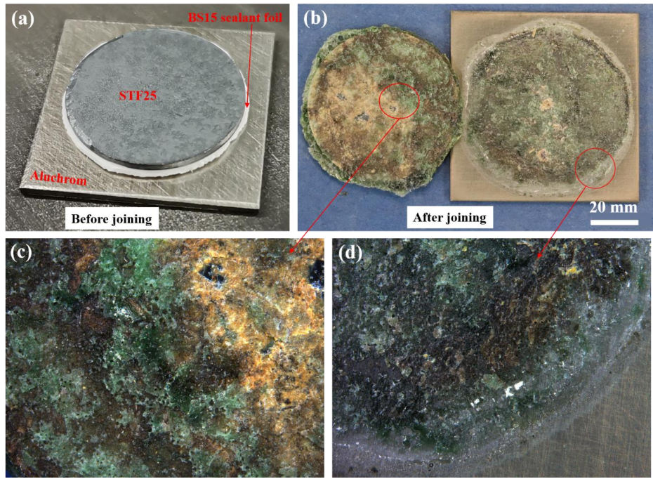
Fig. 4-68. BS15 sealant joining with Aluchrom and STF25 membrane (1075 °C, 5 min), (a) before joining, (b) after joining, (c) zoom in picture of membrane side, (d) zoom in picture of Aluchrom side
