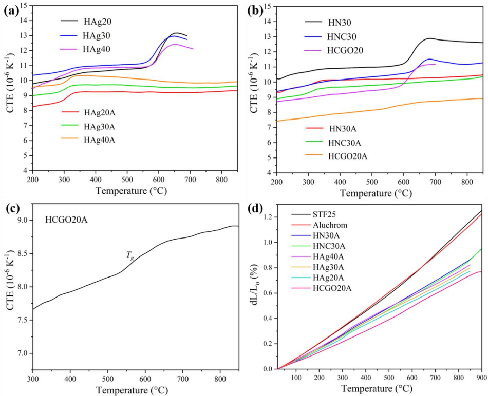
Fig. 4-12. CTE curves for composites samples sintered and annealed: (a) samples with different Ag amounts, (b) compared with different fillers Ni, Ni-Cr (80-20), and CGO samples. (c) CTE curve of annealing sample HCGO20A. (d) Elongation curves after annealing composite samples compared with STF25 and Aluchrom
