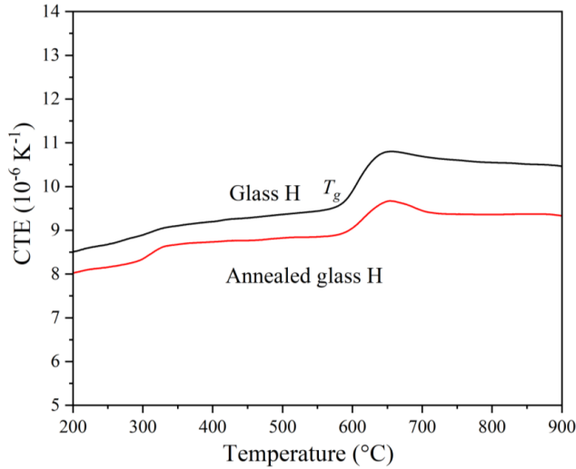
Fig. 4-2. Dilatometer plots of the sintered glass H rod (850 ^{\circ}\text{C} , 10 h) and glass H aged sample (850 ^{\circ}\text{C} , 10 h + 800 ^{\circ}\text{C} , 1000 h)
