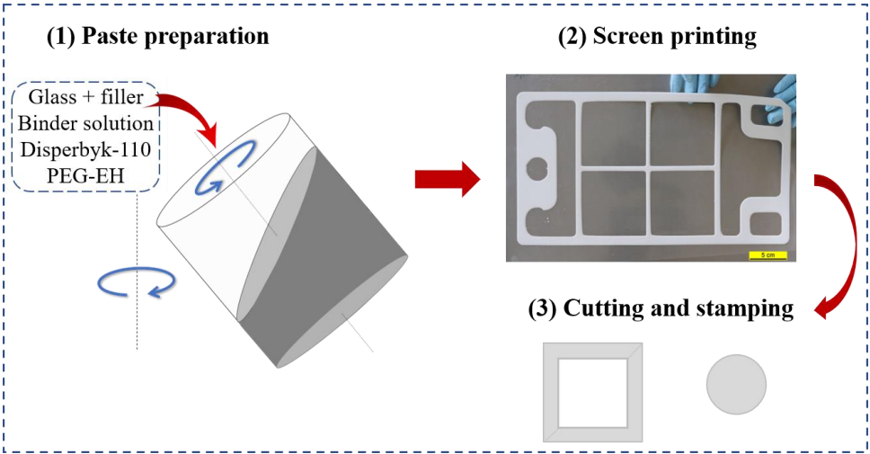
Fig. 3-4. Schematic diagram of screen-printing process, (1) paste preparation, (2) screen-printed sealant green foil, (3) cutting and stamping suitable shapes for next assembling process
