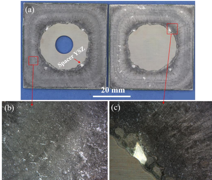
Fig. 4-63. The chopped gas-tight joint Alchrom/BS15/Alchrom joining at 1075 °C for 5 min, (a) overview, (b) and (c) magnification
