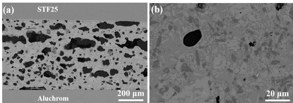
Fig. 4-44. Joint STF25/HBS30/Aluchrom joined at 920 °C for 15 min
