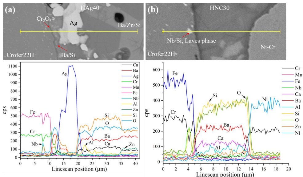
Fig. 4-22. Line scans through the interfaces between (a) HAg40 and Crofer22H, (b) HNC30 and Crofer22H
