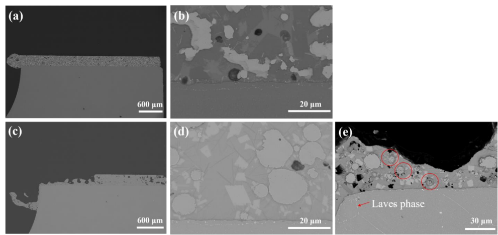
Fig. 4-20. SEM images of cross sections of HAg40 (a, b) and HNC30 (c-e) samples after torsion tests, overview on the left and magnification on the right
