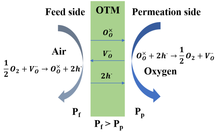
Fig. 2-1. Schematic of oxygen transport processes through an oxygen transport membrane.
