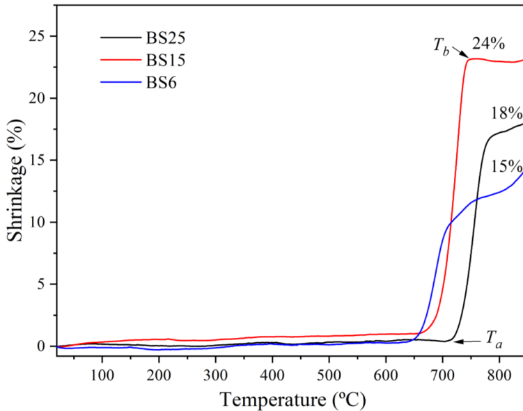
Fig. 4-60. Sinking dilatometry plots of BS glasses
