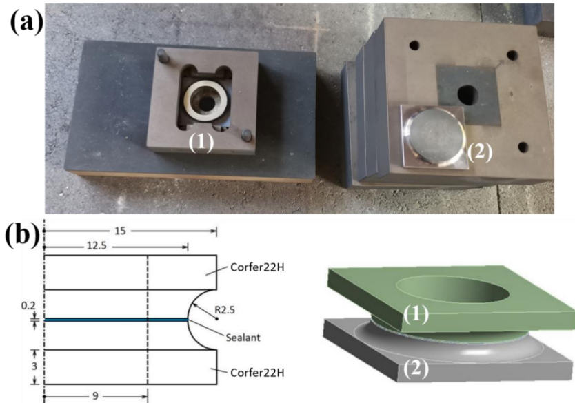
Fig. 3-6. (a) Assembling of hourglass shaped torsion specimen process, sealant was placed in the middle of two Crofer22H plates for further joining at 850 °C for 10 h under a deadload 3900 \pm 100 g; (b) schematic of the hourglass shaped specimens [125] after joining, the dimensions are in mm. (1) is Crofer22H plate with an inner hole of \varnothing 18 mm and green foil of sealant applied to it (2) is opposite Crofer22H plate without hole.
