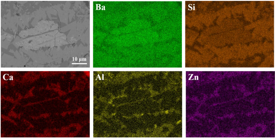
Fig. 4-40. SEM-EDS maps of the sealant HBS30 from STF25/HBS30/pre-Aluchrom joint (960 °C, 5 min) for analyzing filler \text{BaSiO}_3
