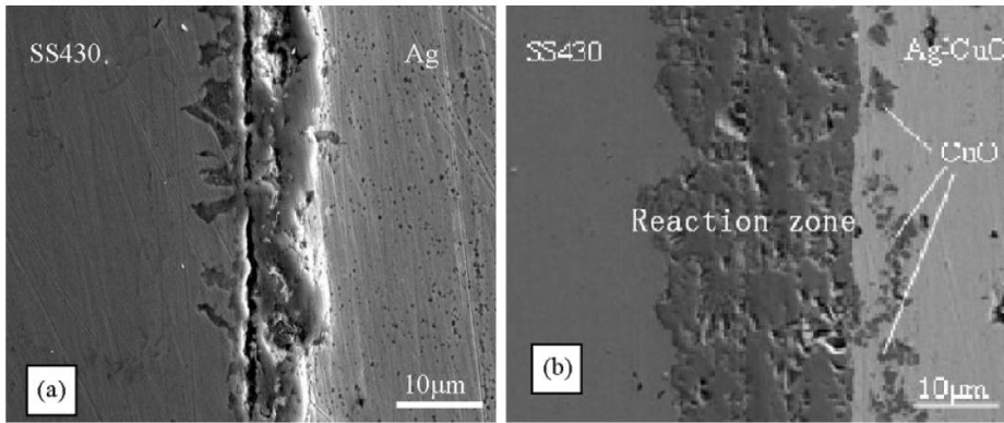
Fig. 2-6. SEM images of cross-sections of the SS430/Ag–CuO sealing interface: brazing in air with (a) pure Ag and (b) 6 mol% CuO [64]
