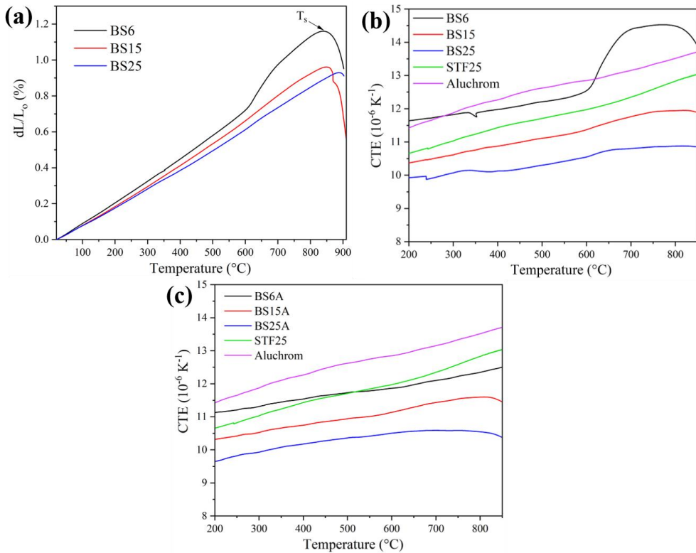
Fig. 4-56. Dilatometer curves of BS glasses, (a) elongation plots, dilatometer softening temperature ( T_s ), (b) CTE of BS glasses as a function of temperature comparing with membrane STF25 and Aluchrom, (c) dilatometer curves of the annealed BS samples after 850 °C for 50 h
