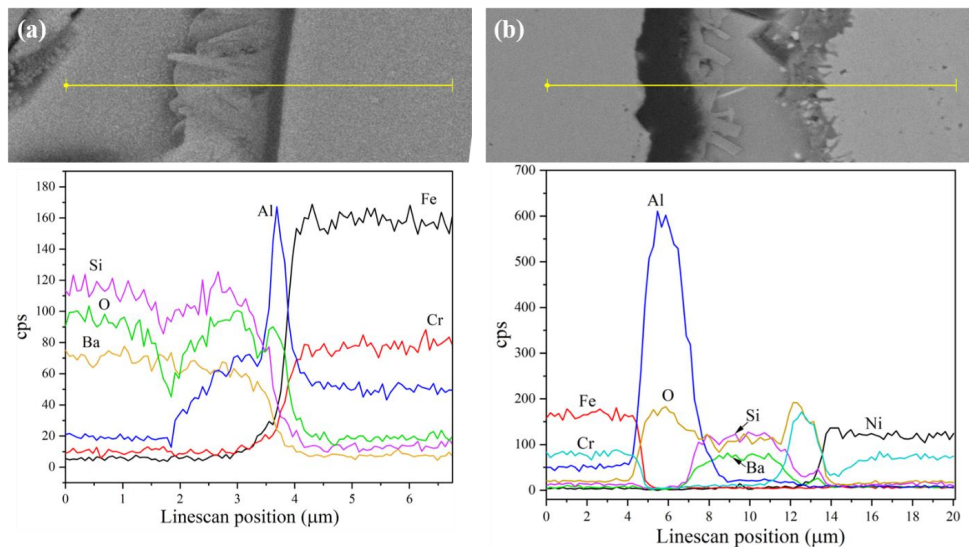
Fig. 4-18. Line scans through the interface between HNC30 and Aluchrom (a), HNC30 and pre-Aluchrom (b)
