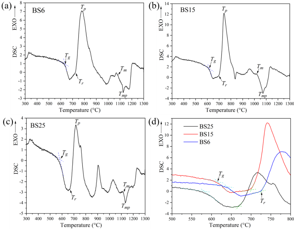
Fig. 4-54. DSC curves of BS glasses at a heating rate of 15 °C/min, (a) BS6, (b) BS15, (c) BS25, (d) magnification of DSC curves between 500 – 800 °C for clear marking T_g and T_r
