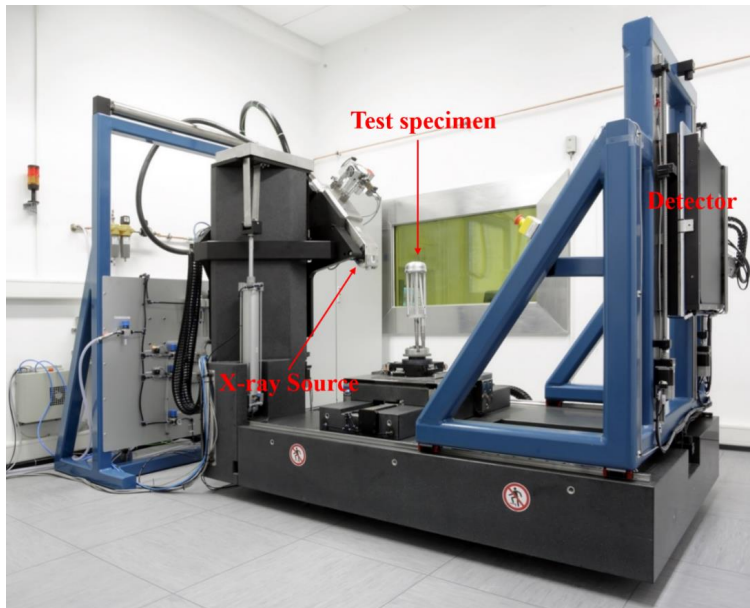
Fig. 3-7. Open X-ray computed tomography system at ZEA-1
