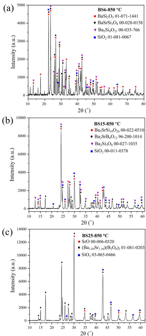
Fig. 4-59. XRD patterns of BS glasses heated at 850 °C for 50 h, (a) BS6, (b) BS15 and (c) BS25
