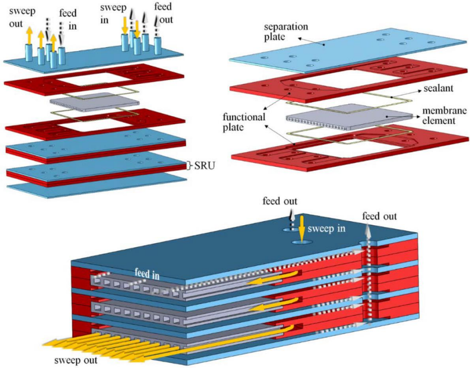
Fig. 2-3. Design concept for the operation of a planar membrane module stack in 4-end mode (top left), single separation unit (SRU, top right), and quarter section with illustrated flow of feed and sweep gas [11].
