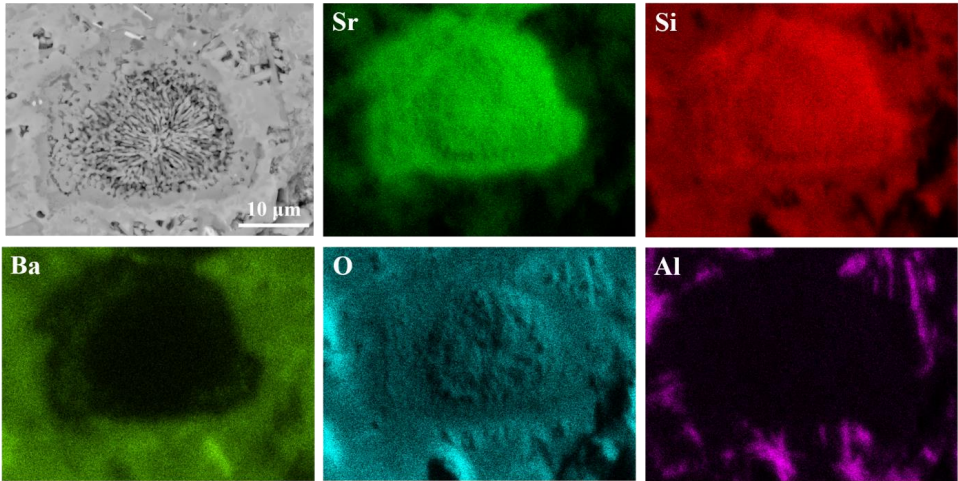
Fig. 4-48. SEM-EDS maps of the HS2S20A sample
