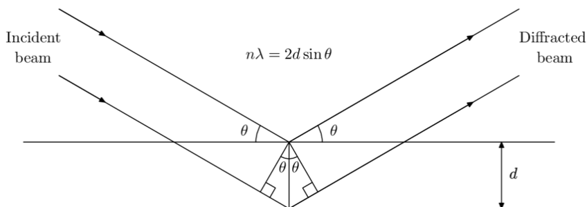
Fig. 3-1. Schematic illustration of Bragg's Law [114]
