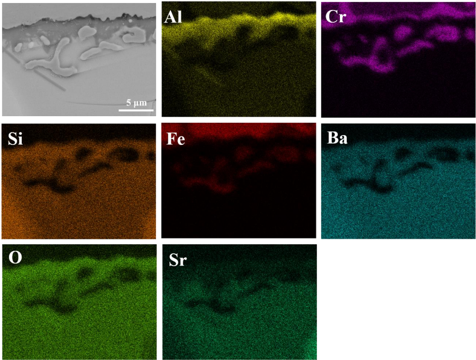
Fig. 4-66. SEM-EDS maps of the gas-tight joint Alchrom/BS15/Alchrom joined at 1075 °C for 5 min to analyze interaction between BS15 glass and Alchrom
