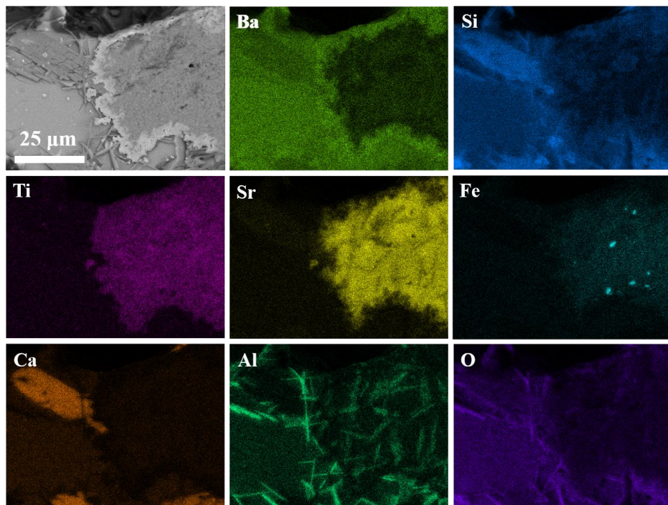
Fig. 4-11. SEM-EDS maps of the H10STF25
