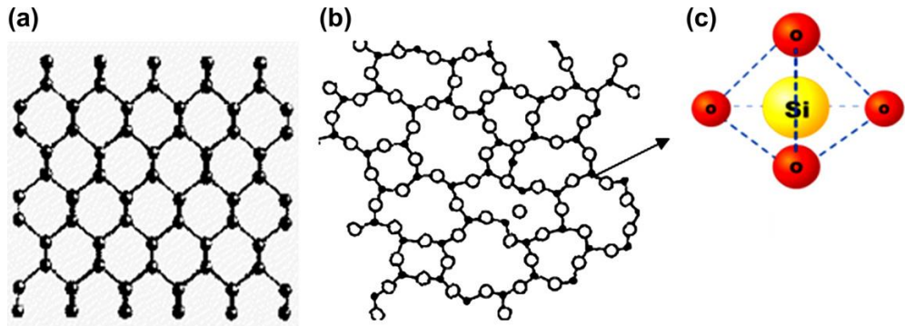
Fig. 2-7. Crystalline structures (a), amorphous randomized structures (b), and the molecular structure of silica-based glass (c) [65]
