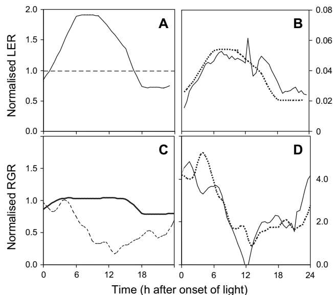
Fig. 7. Addition of the effects of temperature and endogenous rhythms in Z. mays (A, B) and N. tabacum (C, D). (A, C) Effect of temperature (solid line) and of endogenous rhythms (dotted line). (B, D) Experimental diel pattern (mean of experiments on days 2–4, solid lines) and simulation from the superposition of the two effects presented in (A) and (C).
