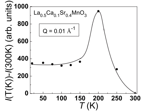
FIG. 12. SANS intensity as a function of temperature at Q = 0.01 \text{ \AA}^{-1} for \text{La}_{0.5}\text{Ca}_{0.1}\text{Sr}_{0.4}\text{MnO}_3 ( x=0.4 ) sample. The continuous line is a guide for the eyes.
