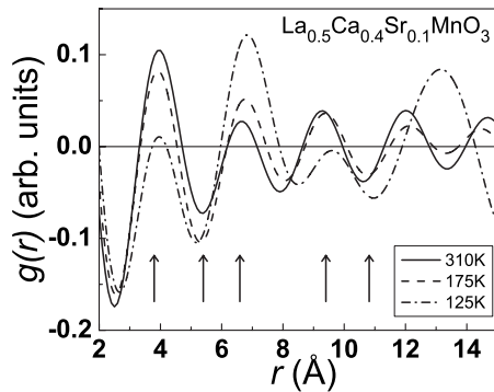
FIG. 7. Radial correlation function g(r) for \text{La}_{0.5}\text{Ca}_{0.4}\text{Sr}_{0.1}\text{MnO}_3 ( x=0.1 ) at 310, 175, and 125 K. Arrows indicate the five nearest-neighbor bond distances for Mn sublattice.
