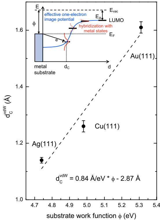
FIG. 7. (Color online) Vertical bonding distances d_C^{\text{vdW}} of PTCDA corrected by the van der Waals radii ( r_{\text{vdW}} ) of the surface atoms versus workfunctions \phi on different (111) coinage metal surfaces ( d_C^{\text{vdW}} = d_C - r_{\text{vdW}} ). The correction by r_{\text{vdW}} accounts for differences in the atomic sizes (Ref. 51). For the d_C values of PTCDA/Cu(111) and PTCDA/Au(111) see Refs. 21 and 20, respectively. Work functions of the clean metals are from Ref. 53. The dashed line represents a linear fit to the data points. The empirically found correlation between d_C^{\text{vdW}} and \phi is given. The inset illustrates schematically the energetic lowering and occupation by electrons of the LUMO and is discussed in the text.
