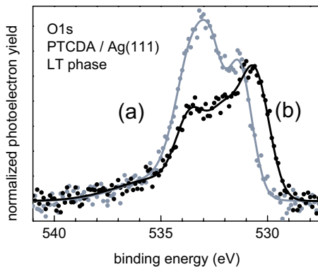
FIG. 2. Adsorption of water at low temperatures. O 1s photoemission spectra of the LT phase of PTCDA on Ag(111) for different times of exposure to the x-ray beam taken at a pass energy of 23 eV. (a) Fresh spot of a sample being held at low temperature for 11 h. (b) Same spot after 6 h exposure to the x-ray beam. The change in the peak shape is due to photon-induced desorption of water. The photon energy was about 17 eV below the Bragg condition.
