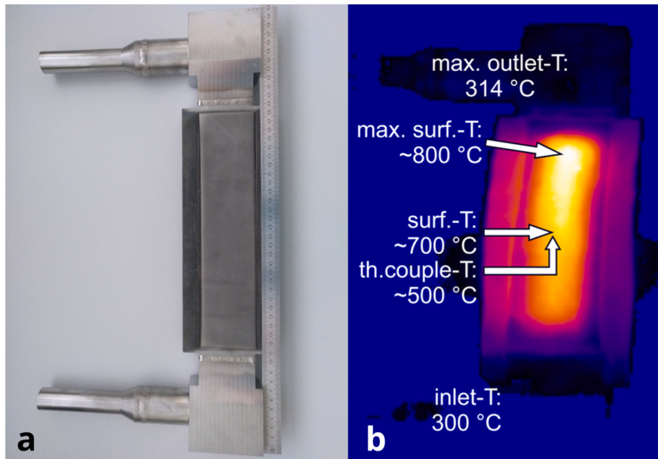
Fig. 3. (a) Mock-up with coated area 270 \times 65 \text{ mm}^2 for use in high heat flux test. (b) Infrared thermograph showing temperature of the mock-up during high heat flux test. Image reprinted and adapted from ref. [16] with permission from the IAEA and Euratom.
