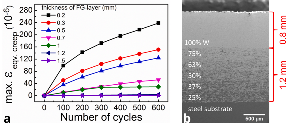
Fig. 1. (a) Maximum equivalent creep strain in the steel substrate for varying coating thickness, over several hundred simulated operational cycles. Image reprinted from ref. [6] with permission from Elsevier. (b) Cross section of functionally graded coating with interlayer tungsten content indicated.
