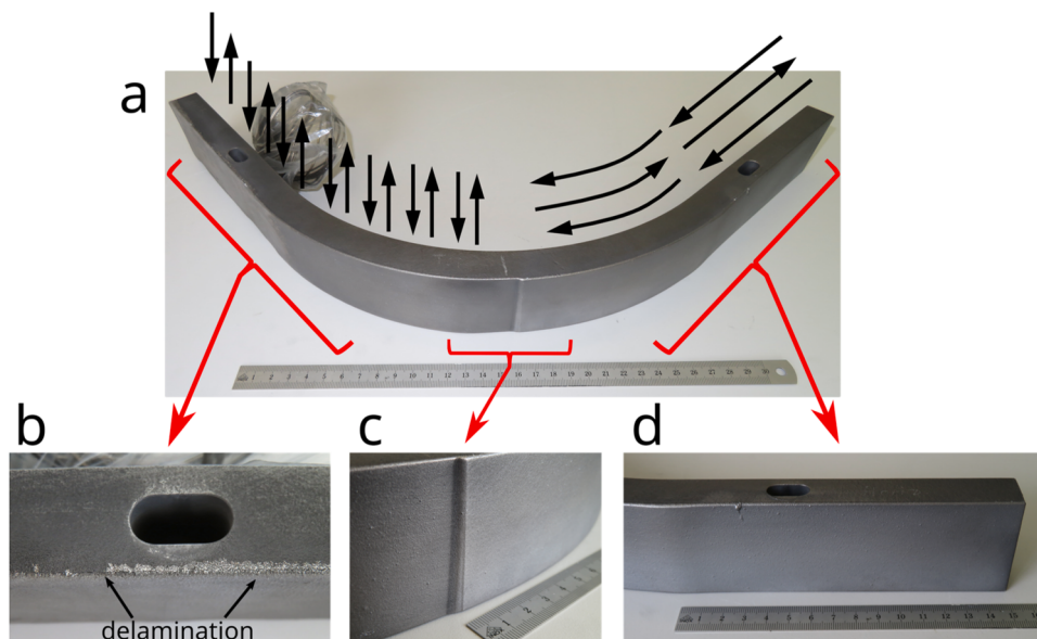
Fig. 6. (a) Experimental coating on substrate with transition from straight to curved geometry, comparing vertical coating deposition (left, b) with horizontal deposition (right, d). Delamination was found near bearing for vertical coating direction (b). No delamination was found near coating tips in middle (c) or for horizontal coating direction (d).
