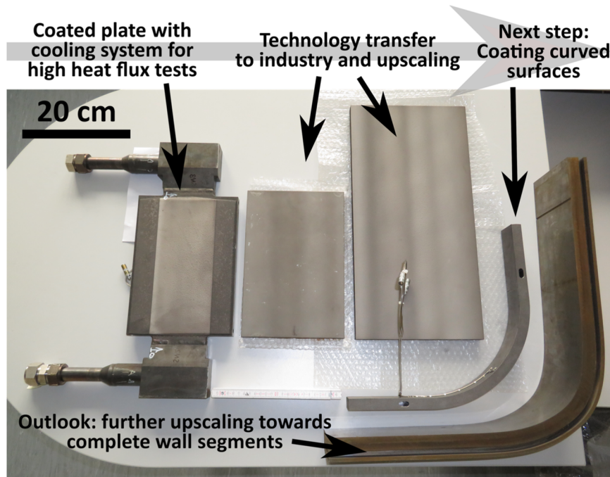
Fig. 2. Overview of different development steps during upscaling of coating technology.
