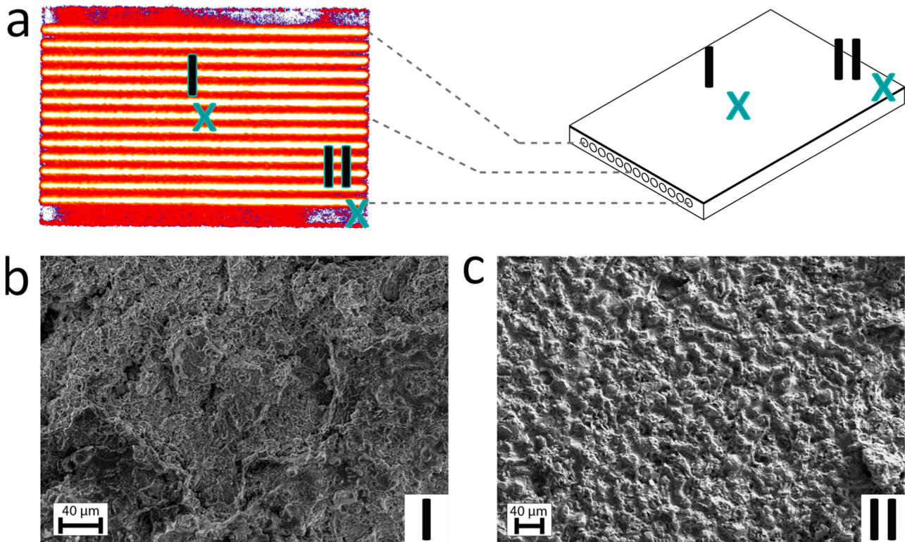
Fig. 4. (a) Ultrasonic analysis of coated 300 \times 200 \text{ mm}^2 plate and schematic illustration of plate. (b,c) Fracture surfaces at coating-substrate interface after provoked delamination, samples from regions marked I, II in (a).
