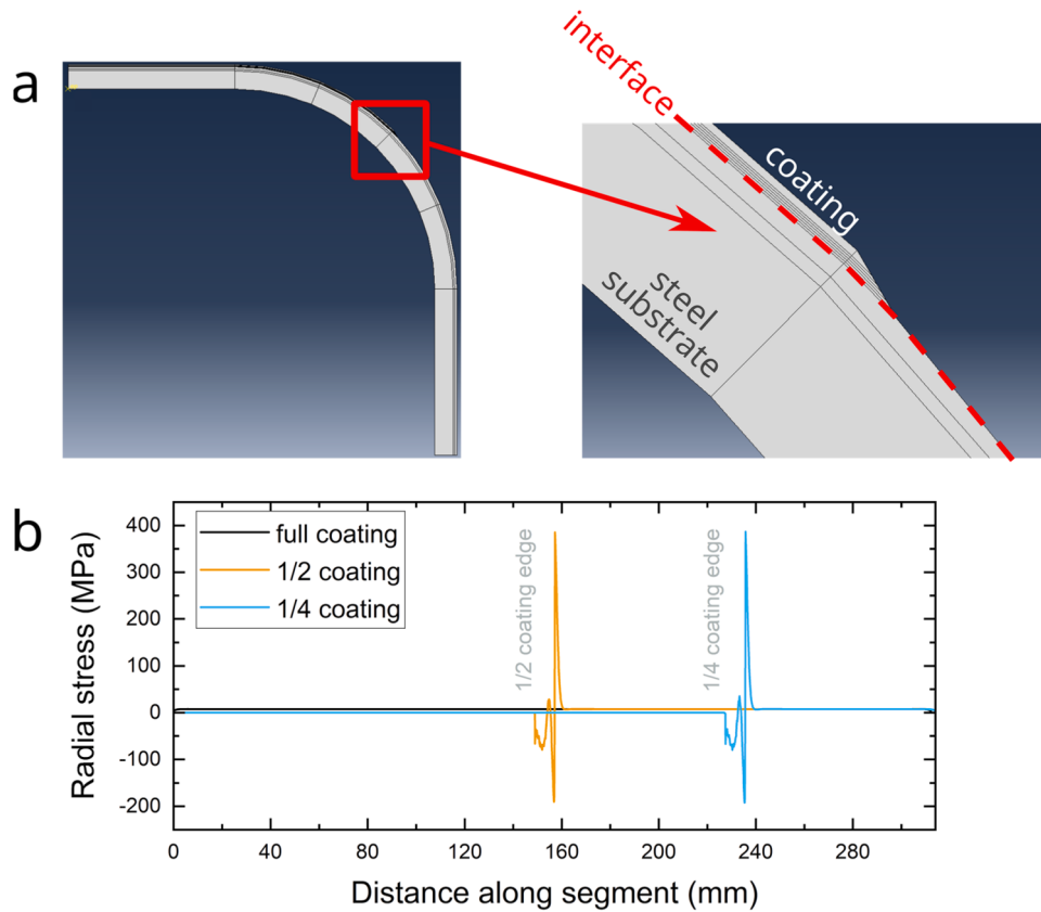
Fig. 5. (a) Finite element model of a curved substrate with outer radius of 200 mm and coating over the top half of the outer surface (“ \frac{1}{2} coating” in text). Magnification shows edge of coating. (b) Simulated radial stress at coating-substrate interface along curved segment with full / \frac{1}{2} / \frac{1}{4} coating. For the \frac{1}{2} and \frac{1}{4} coatings, the uncoated region is on the left (zero stress) and the coating begins towards the right, at the stress peaks.
