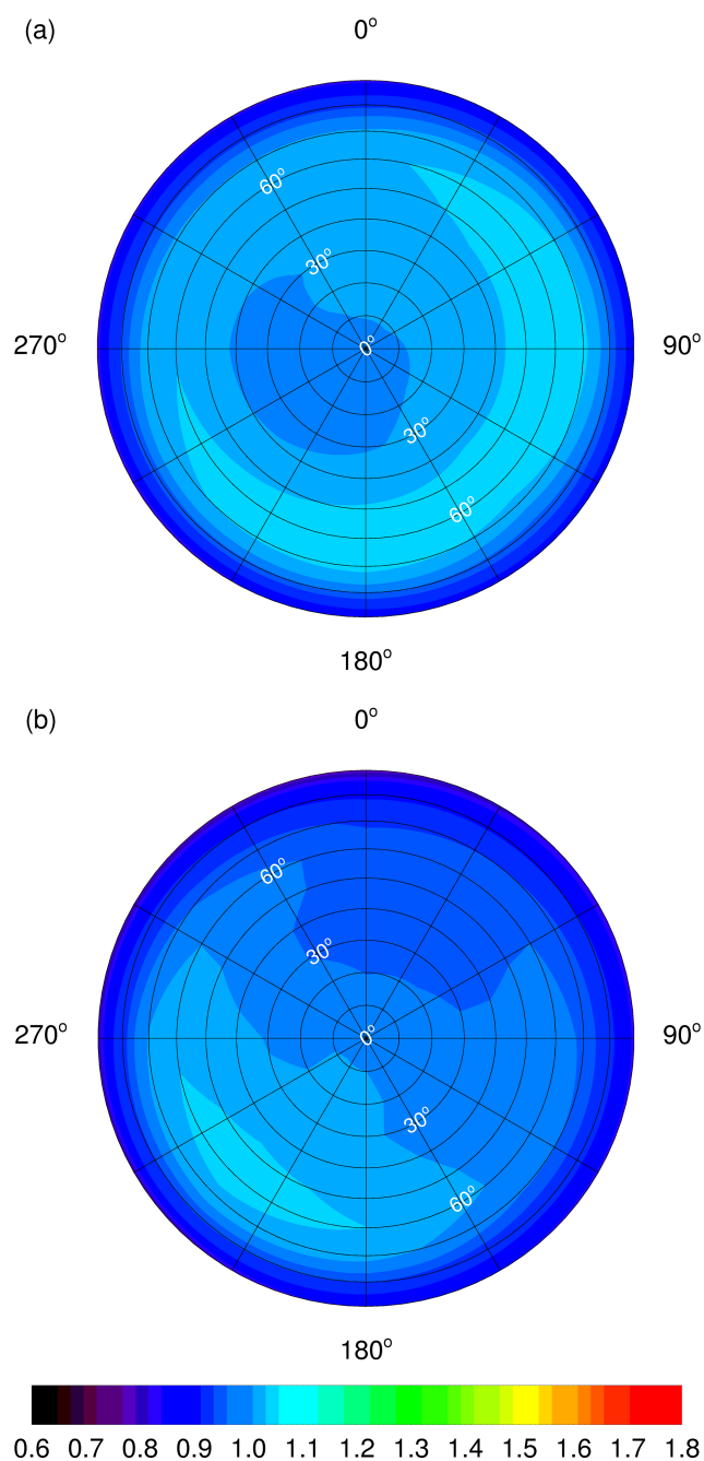
Figure 4. Contour plots of hemispherical relative angular sensitivities Z_p of HALO 2π (a) and (b) receivers at 400 nm (top views). Azimuth angles of 0° correspond to flight directions of aircraft-installed receivers. Polar angles of incidence are indicated (white). Note that cross-talk to the lower hemisphere is invisible in this representation. The colour scale was chosen for better comparability with Fig. 6.
