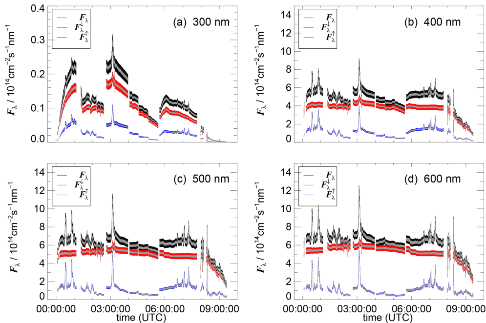
Figure 18. Total ( F_{\lambda} ), downward ( F_{\lambda}^{\downarrow} ) and upward ( F_{\lambda}^{\uparrow} ) spectral actinic flux densities of the HALO flight shown in Fig. 17 for the four selected wavelengths in panels (a)–(d). The colour-coded error bars correspond to total uncertainties, including those from corrections and calibrations (Sect. S7). The overlying grey error bars indicate the uncertainties from the corrections alone.
