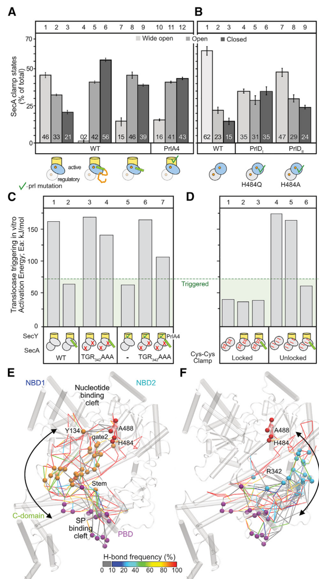
Figure 3. Clamp closing underlies translocase triggering
