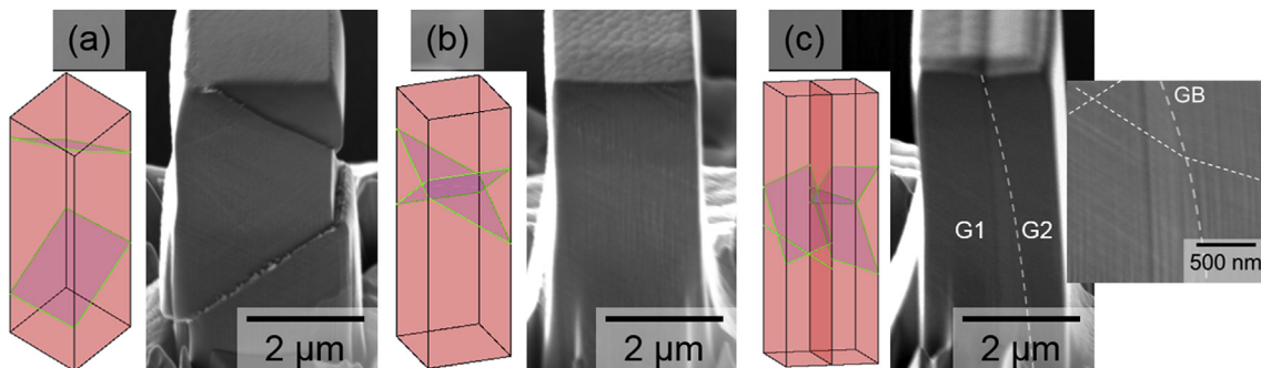
Fig. 2. SEM micrographs (45° tilt angle) of deformed micropillars (a) G1, (b) G2, and (c) G12 after 100 loading cycles. The corresponding sketches show the activated slip planes. The inset of (c) shows the slip lines on the pillar face of the two crystal orientations in G12 at higher magnification.
