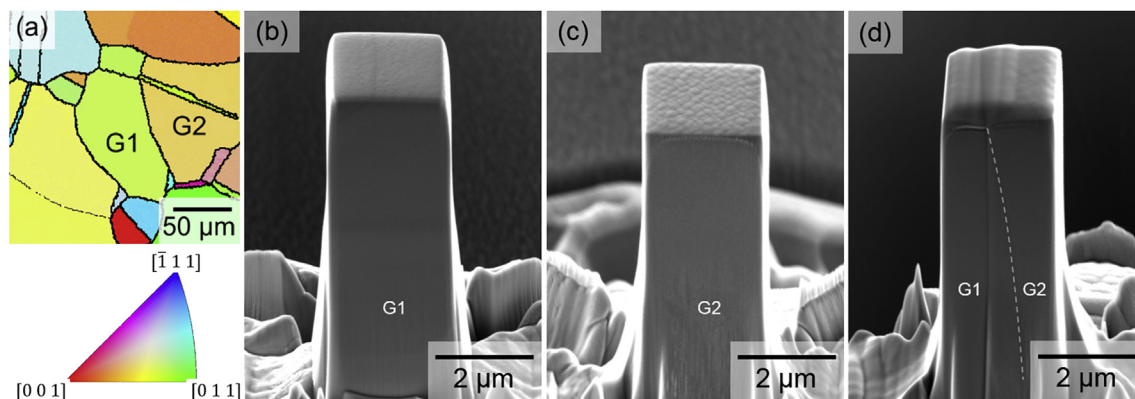
Fig. 1. (a) EBSD map of the high-purity Ni foil after annealing; (b), (c) SEM micrographs (52° tilt angle) of single crystal micropillars, which were fabricated by FIB-milling in selected grains G1 and G2; (d) bicrystal pillar G12 containing the grain boundary in-between grains G1 and G2.
