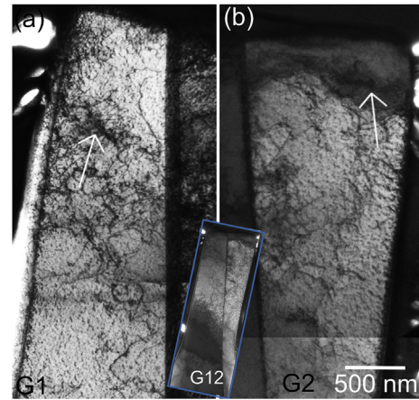
Fig. 5. Bright-field-TEM micrographs of the bicrystalline micropillar G12, with (a) showing G1 and (b) showing G2. The white arrows mark the position of early-stage vein structures in both grains.
