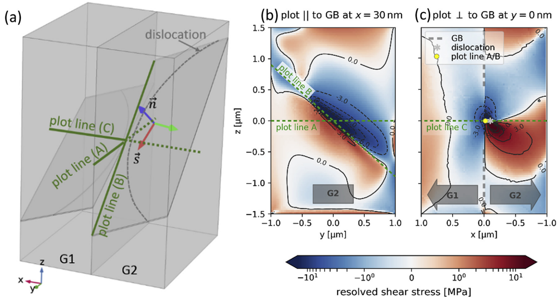
Fig. 9. (a) Geometry of the bicrystal used for the discrete dislocation simulation. The origin of the x-y-z coordinate system is in the center of the pillar, \vec{n} is the slip plane normal and \vec{s} the slip direction parallel to the Burgers vector \vec{b} . (b) and (c) show the RSS for the (111)[01 \bar{1} ] G2 system near the grain boundary plane (left plot) and in a plane cutting perpendicularly through the grain boundary (right plot).
