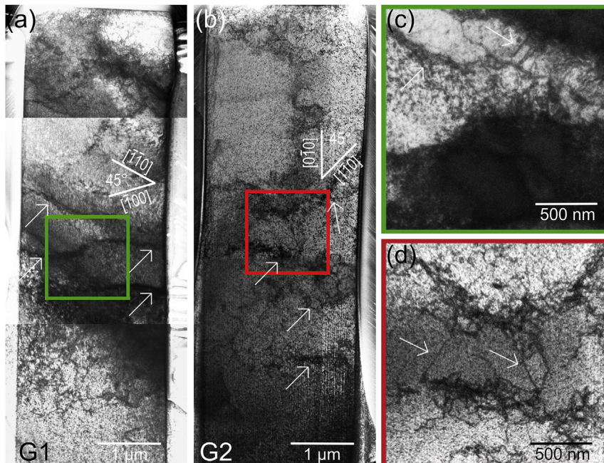
Fig. 4. (a),(b) Bright-field-TEM micrographs of micropillars G1 and G2 after cyclic deformation: The zone axis in both samples is close to [001] . White arrows mark the dislocation cell walls in the structure. (c), (d) Magnified bright-field TEM micrographs of the regions marked in (a) and (b) showing screw dislocations confined between the channels (indicated by white arrows).
