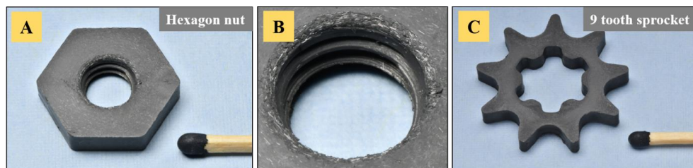
Figure 4. 5: Powder injection molded \text{Ti}_2\text{AlC} -based components: (A) M8 hexagon nut, (B) magnified threaded hole and (C) 9-tooth sprocket.
