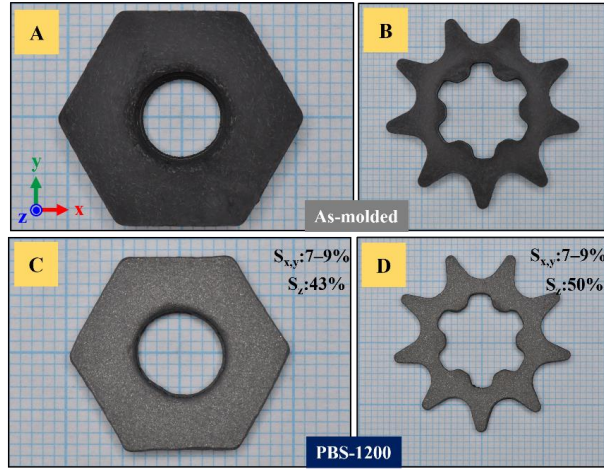
Figure 5. 14: Powder bed sintered monolithic and N720 alumina fiber-reinforced (20 vol.%) \text{Ti}_2\text{AlC} nuts and sprockets: (A) and (B) are as-molded, (C) and (D) are PBS parts. Sintering shrinkage in each direction is given by the S values.
