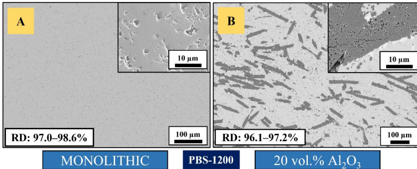
Figure 5. 15: Microstructure of powder bed sintered monolithic and N720 alumina fiber-reinforced (20 vol.%) \text{Ti}_2\text{AlC} . RD designates the achieved relative density.
