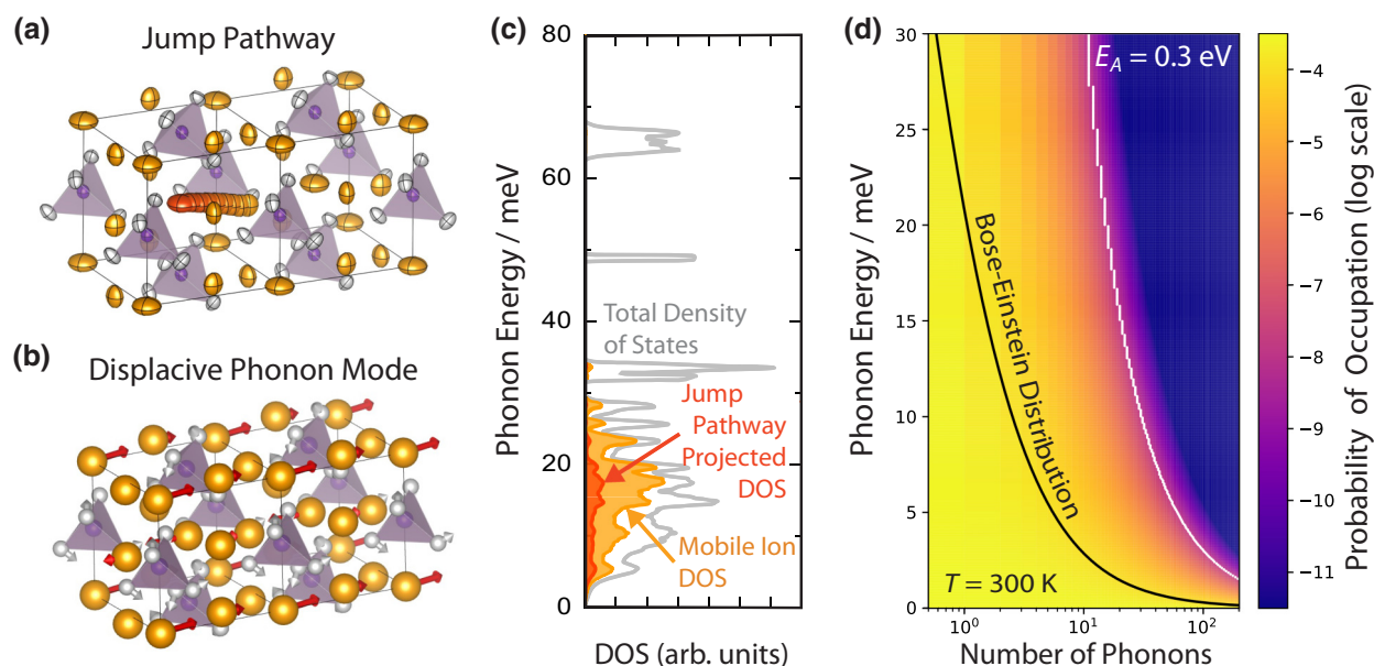
FIG. 4. Vibrational understanding of ionic transport. (a) Schematic of the lowest energy pathway for a mobile ion to move between crystallographic sites. (b) Single low-frequency phonon mode, where phonon eigenvectors indicate a displacive motion of mobile ions along the jump pathway shown in panel (a). (c) By analyzing the phonon eigenvectors for all of the mobile ion vibrational modes, it is possible to see the spectral density of states of vibrations that contribute to the net motion of the mobile ion along the jump pathway. (d) Bose-Einstein distribution gives the average number of thermal phonons expected to be populated at a given temperature and vibrational mode energy (frequency), where lower frequency modes have higher average phonon occupations; however, the instantaneous occupation of phonons in a vibrational mode is a fluctuating quantity and the probability of a given number of phonons follows a Boltzmann distribution (see the color map). Also shown is the number of phonons that would be required in a given phonon mode to achieve a thermal energy of 0.3 eV, which is a typical activation barrier energy for ion transport in fast ion conductors.
