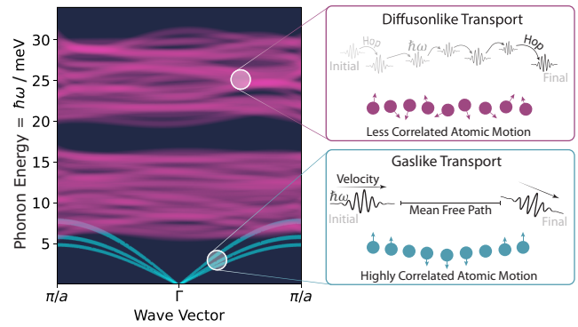
FIG. 2. Phonon character and thermal transport behavior. Schematic phonon dispersion in which acoustic (blue) vibrational modes are highly dispersive and distinct, resulting in gaslike phonon transport of vibrational energy \hbar\omega , whereas optical (pink) vibrational modes have little dispersion and a high degree of (quasi-)degeneracy, which gives rise to diffusonlike hopping transport of vibrational energy \hbar\omega as an atomic scale random walk.
