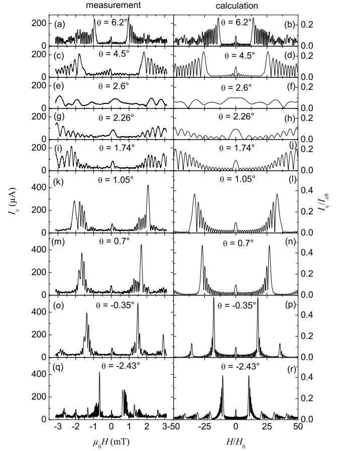
FIG. 4. I_c(H) patterns for different misalignment angles \theta .
