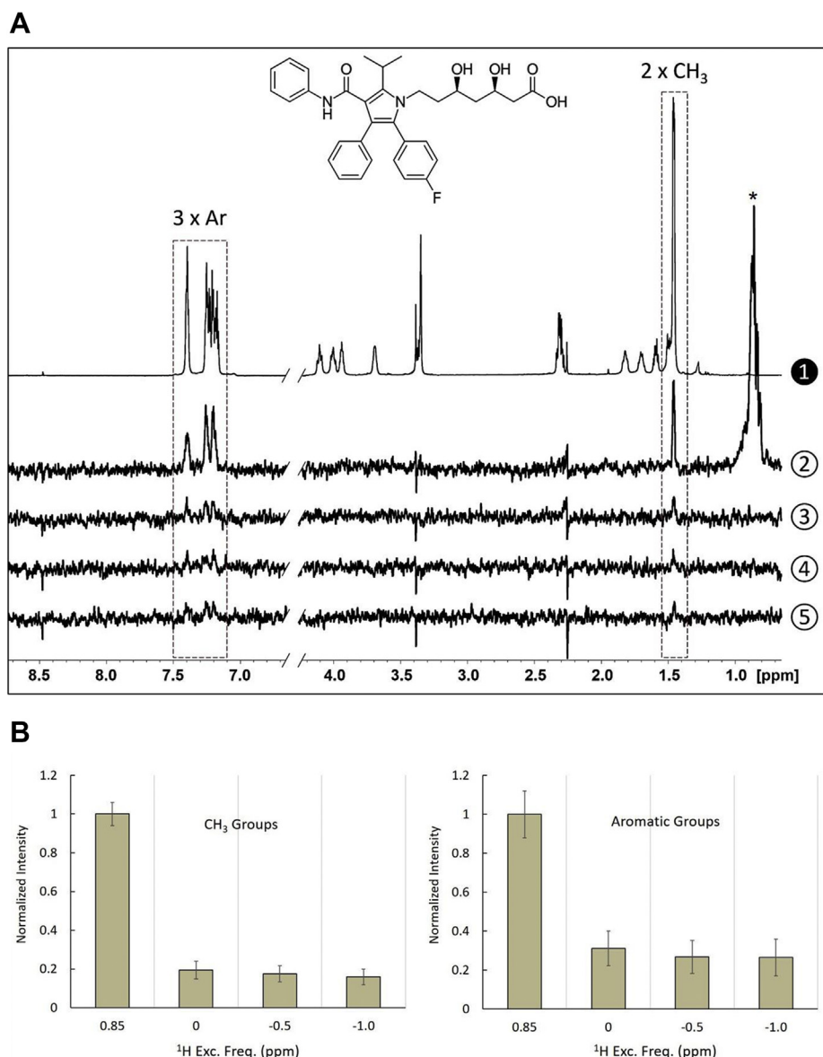
Figure 6. STD-NMR of 5.0 \mu M A \beta 42 in the presence of 300 \mu M Ca-free Ator at 310 K. A, Ator's 1D ^1\text{H} NMR spectrum was used as a reference (①). The saturation of A \beta 42 at 0.85 ppm resulted in the appearance of Ator's STD signals belonging to its \text{CH}_3 and aromatic groups (②). The NMR signal marked by asterisk belongs to A \beta 42's \text{CH}_3 groups saturated at this frequency. A \beta 42 saturation at 0 (③), -0.5 (④), and -1.0 (⑤) ppm, resulted in a similar phenomenon so that the saturation was transferred to Ator's \text{CH}_3 and aromatic groups. B, normalized intensity of Ator's signals as a function of A \beta 42 ^1\text{H} saturation frequency showed that there is a significant interaction between Ator and A \beta 42 oligomers. Ca-free Ator, calcium-free atorvastatin; STD, saturation-transfer difference.
