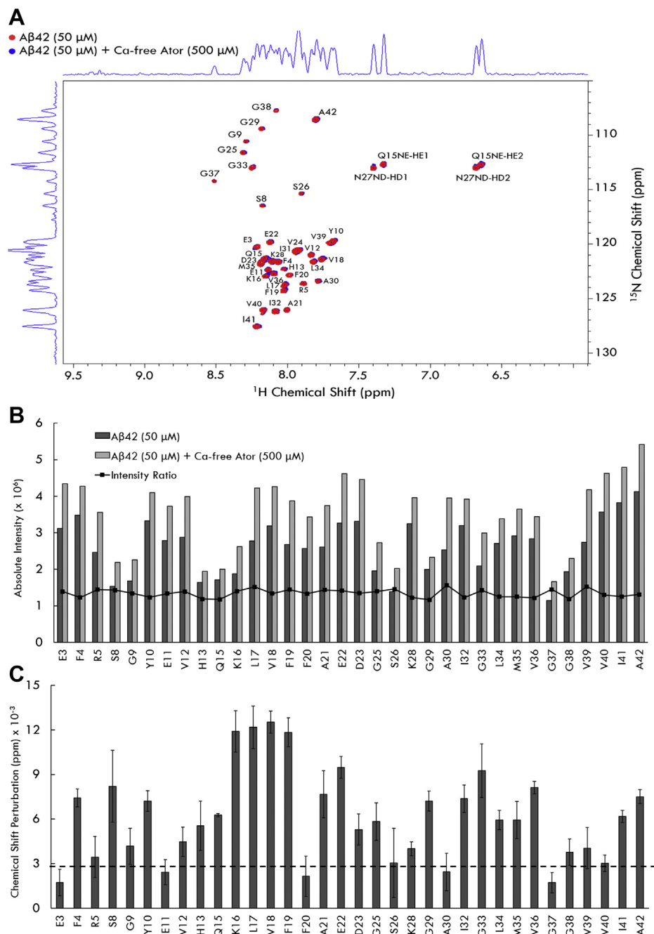
Figure 5. Interaction of monomeric Aβ42 with atorvastatin (Ator) probed at single-residue resolution. A, shows the 1 H- 15 N HSQC spectra of 50 μM monomeric Aβ42 treated with 0 (red) or 500 μM Ca-free Ator (blue). B, shows Ator-induced perturbations in the intensity of Aβ42's crosspeaks over the peptide sequence. A nearly uniform intensity gain is observed along the Aβ42 sequence. C, shows the combined 1 H, 15 N chemical shift perturbation of Aβ42 induced by Ator as a function of residue number. Residues K16, L17, V18, and F19 exhibit the largest chemical shift perturbations, when compared with the background chemical shift variation (presented as the dashed line). Ca-free Ator, calcium-free atorvastatin; HSQC, heteronuclear single quantum coherence.
