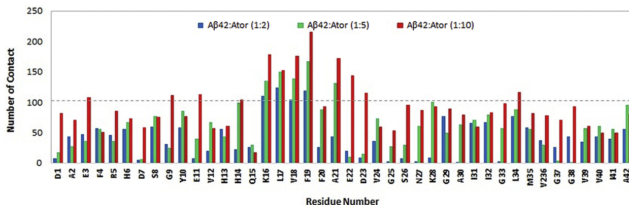
Figure 9. Time-averaged number of nonpolar contacts between A \beta 42 residues and atorvastatin (Ator) molecules in A \beta 42:Ator (1:2), A \beta 42:Ator (1:5), and A \beta 42:Ator (1:10) systems. Ator, atorvastatin.
