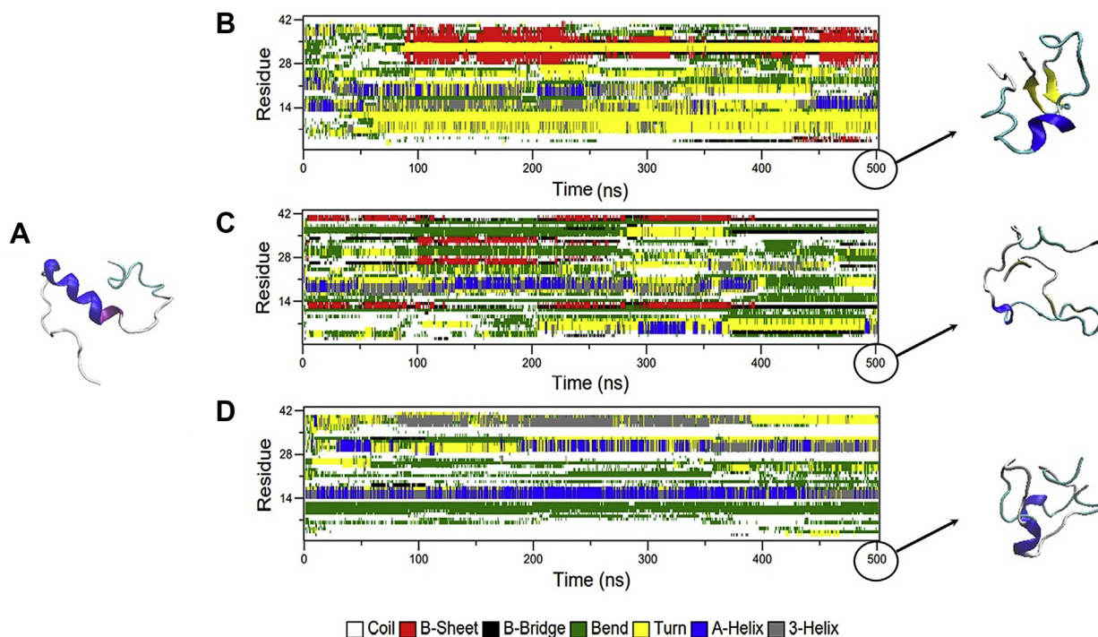
Figure 7. Secondary structure analysis of various Aβ42-Ator systems using the DSSP program. A, initial structure of Aβ (Protein Data Bank ID: 2LFM). Time evolution of the secondary structures of Aβ42 for Aβ42:Ator (1:2) (B), Aβ42:Ator (1:5) (C), and Aβ42:Ator (1:10) (D) systems. As shown, as the concentration of Ator increases, the conformational transition of residues 28–38 to β-sheet structures is prevented. Ator, atorvastatin.
