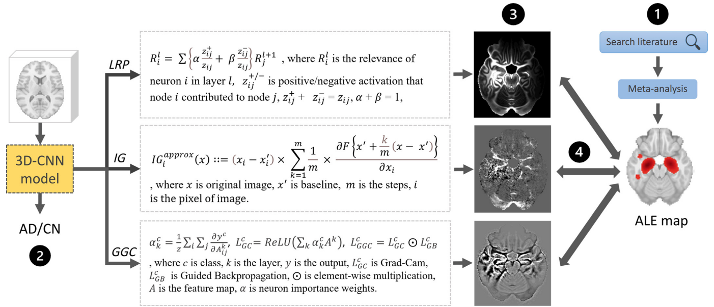
Fig. 1. An overview of the present study. (1) A VBM meta-analysis was conducted to derive an Activation Likelihood Estimation (ALE) map summarizing AD effects on the brain visible in T1-weighted MRI scans. (2) 3D CNNs were trained to classify AD and CN ADNI T1-weighted MRI scans. (3) Three heatmap methods were applied to the CNN models with the highest cross-validation accuracy. (4) The heatmaps were compared with the meta-analysis map.
