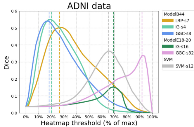
Fig. 5. For each heatmap method, the Dice curve of ADNI data corresponding to the spatial smoothing reaches the best overlap with the meta-analysis. ModelB44 achieved the best accuracy and ModelE18-20 achieved the best accuracy among residual networks. Linear SVM with SVM-C parameter of 0.001 achieved the best accuracy among tested SVMs. LRP-s7 corresponds to the LRP heatmap after 7 mm FWHM Gaussian smoothing, and similarly for other methods.
