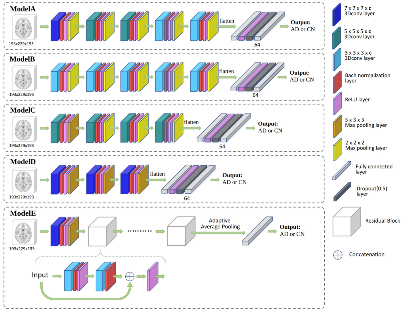
Fig. 2. CNN models used in this study to classify ADNI AD participants and controls. For each architecture, several numbers of channels c were tested. The number of channels c corresponds to the number of 3D convolutional kernels used in each convolutional layer. Increasing numbers of layers were tested for ModelE. The Residual Block used in ModelE concatenates its input with the output of two 3 \times 3 \times 3 \times c convolutional layers.
