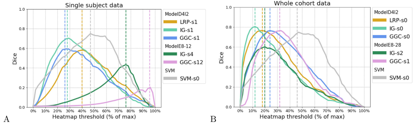
Fig. 3. Dice curves reaching the best overlap between the brain region altered in the synthetic data for heatmaps and SVM activation patterns; (A) for the single subject data set, and (B) for the whole cohort data set. ModelD4I2 achieved the best accuracy for both datasets. ModelE8-12 achieved the best accuracy among the residual networks for single subject data and ModelE8-28 for whole cohort data. Only the best SVM model is shown. s0 indicates a heatmap that was unsmoothed, s1 indicates a heatmap smoothed by a Gaussian kernel of 1 mm FWHM, and s2 indicates a 2 mm FWHM smoothing.
