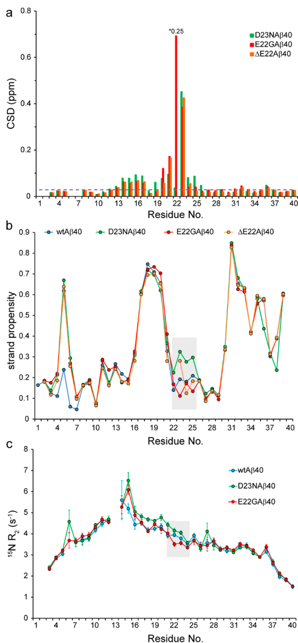
Figure 3. Effect of FAD mutations on the structure and dynamics of Aβ40 variants. (a) Combined 15 N and 1 H chemical shift deviation (CSD) of D23N-, E22G-, and ΔE22-Aβ40 peptides with respect to the wild-type-Aβ40, showing significant chemical shift differences around the respective mutation sites and to a lower extent around residues H14-L17. The dashed line represents the noise level in chemical shift values. For the sake of visibility, the CSD value of residue 22 in the E22G-Aβ40 peptide has been scaled down by a factor of 4. (b) The strand propensity of wild-type-, D23N-, E22G-, and ΔE22-Aβ40, calculated on the basis of their backbone (CO, Cα, N, HN, Hα) plus Cβ chemical shifts. The shaded area shows how the respective mutations alter the strand propensity around the site of mutation (see also Supplementary Figure S3). (c) Residue-specific 15 N transverse relaxation ( R_2 ) rates of Aβ40 variants measured at 278 K. Note the larger R_2 of D23N-Aβ40 and smaller R_2 of E22G-Aβ40 around the mutation site (shaded area), indicating respectively their relative rigidity and flexibility when compared with the wild-type-Aβ40. The relative rigidity of the D23N-Aβ40 variant extends further proximally to Q15-K16.
