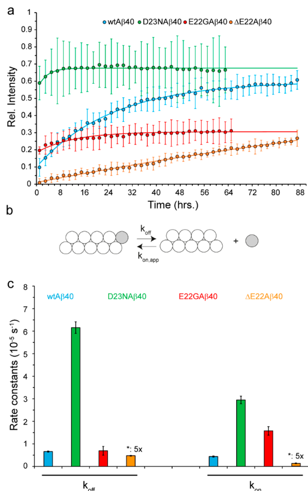
Figure 2. Stability of A\beta 40 aggregates against high pressure. (a) Pressure-induced monomer release from A\beta 40 aggregates, as followed by real-time NMR experiments at 2000 bar, 278 K, through average ( \pm SD) peak intensities. (b) A simple kinetic model of A\beta 40 disaggregation, involving only two states (aggregate state, monomer state) and two rates (dissociation, k_{\text{off}} , and back-association, k_{\text{on}} ). (c) Rate constants obtained from the analysis of monomer release kinetic data shown in (a), according to the simple model shown in (b). The D23N- A\beta 40 variant showed much larger k_{\text{off}} and k_{\text{on}} rates than the wild-type variant, while the \Delta E22- A\beta 40 variants showed smaller k_{\text{off}} and k_{\text{on}} rates. See the text for further details and interpretations. For the sake of visibility, the rate constants of \Delta E22- A\beta 40 are multiplied by a scaling factor of 5. The error bars represent fitting errors.
