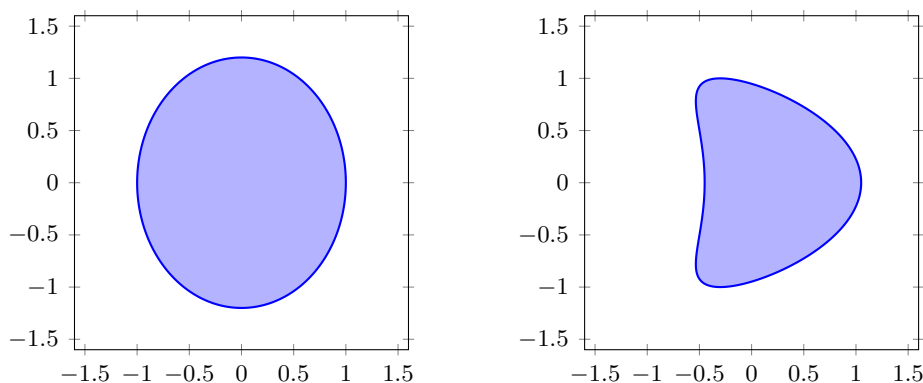
Figure 4: Graphical representation for the elliptical and kite-shaped domains considered in this section.
