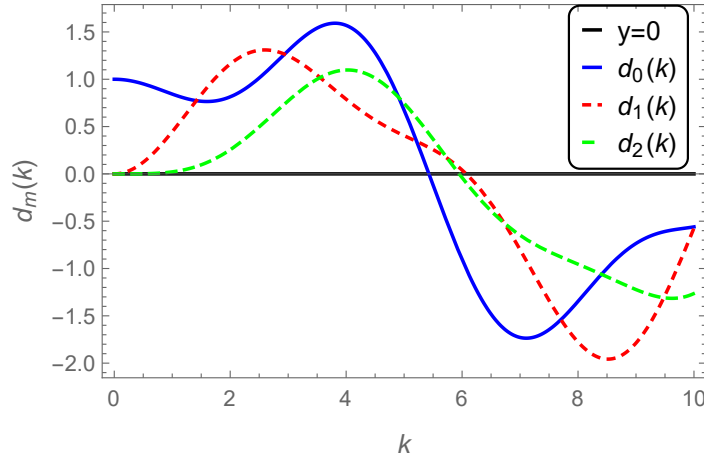
Figure 3: The plots of the determinant function d_m(k) for m = 0, 1, 2 . Here the parameters are given by n = 1/6 , \lambda = 5 , and \eta = -1 .
