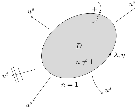
Figure 1: Illustration of the direct scattering problem in \mathbb{R}^2 .
