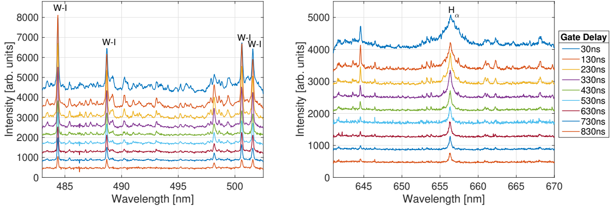
Figure 2. Time resolved emission from the tungsten sample under fs laser irradiation in argon. The gate width is set to 100 ns and the laser fluence is determined as 31 \text{ J/cm}^2 . For visibility 400 counts are added across two distinct spectral ranges for each given gate delay.
