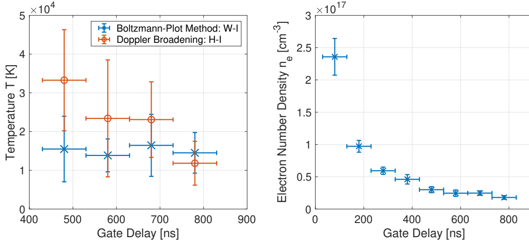
Figure 3. Left: Plasma temperature T evaluated from the observed tungsten (W) spectrum by using the Boltzmann-plot method including atomic W-I lines in blue crosses and the Doppler Broadening of the H_\alpha line in orange circles. Right: Electron number density n_e evaluated by Stark broadening of the same line. Error-bars indicate statistical deviations from the measured values on the y-axis and the used gate width on the x-axis.
