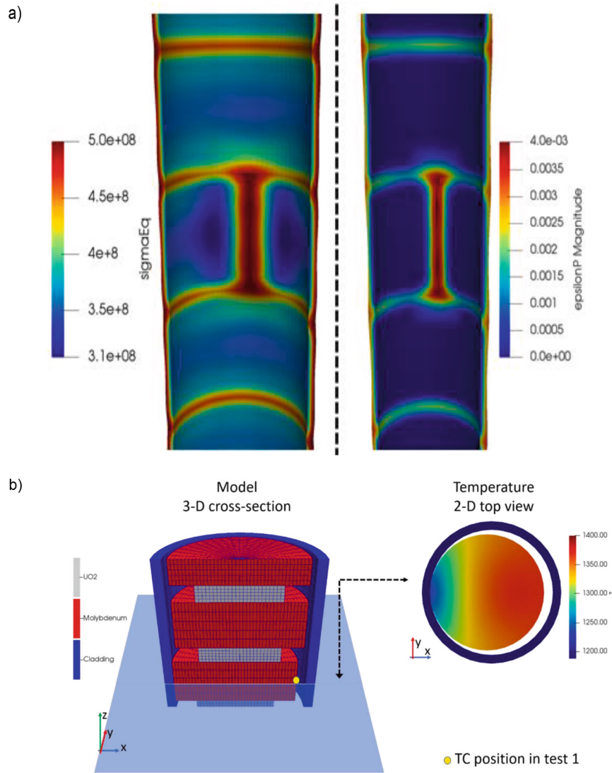
Fig. 8. a) 3-D thermo-mechanical simulation of a pin, including a missing pellet surface ( \sigma_{Eq} and \epsilon_{P} represent the Von Mises stresses and the plastic deformations, respectively). b) Cross section of a 100% eccentricity model used for the stack S41 from the HBRP experiment (left); detail showing the 2-D temperature distribution on a radial slice at the center of the eccentric molybdenum disc (right).
