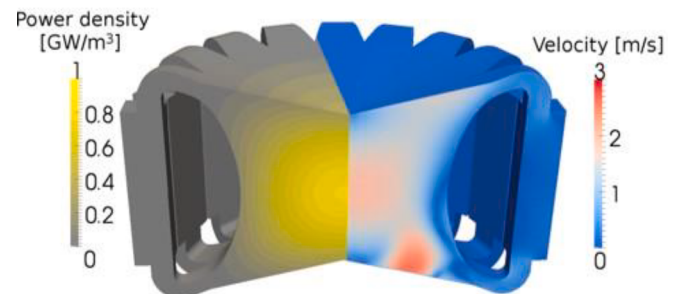
Fig. 2. Velocity and power density fields in the MSFR after the single pump failure accident obtained in first OpenFOAM solver for MSR (Aufiero, 2014).
